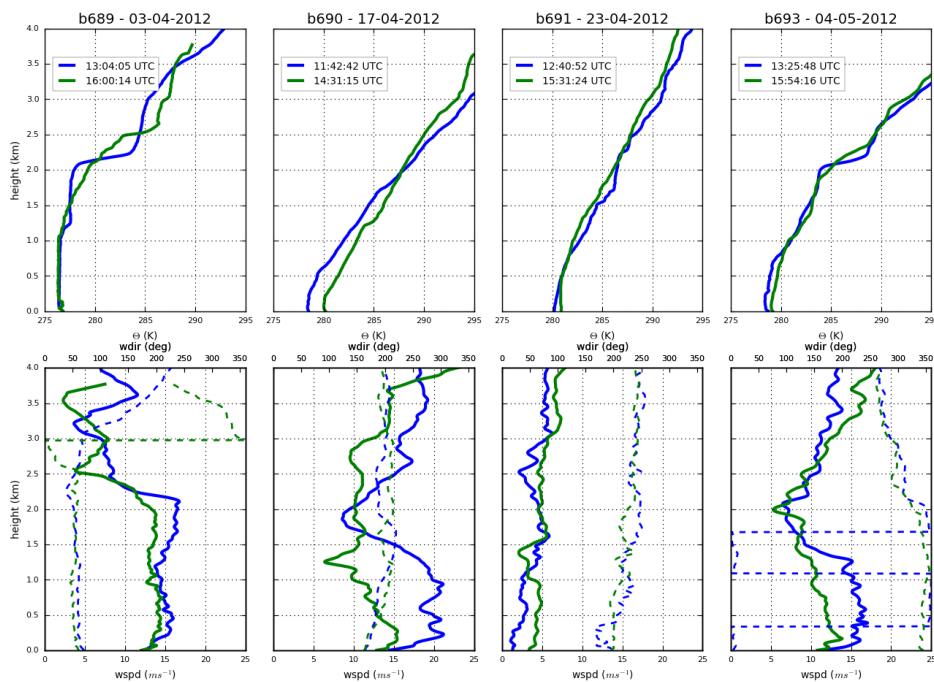
5 Figure 5: Profiles of potential temperature (upper panel) and wind speed (solid lines) and direction (dashed lines) (lower panel) from dropsonde data early (blue) and late (green) in the flight for B689, B690, B691, and B693.
