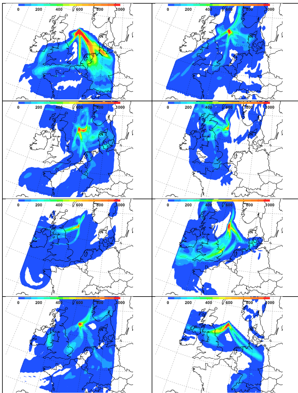
Figure 9: Weekly HYSPPLIT calculations of methane concentration over the European domain for weeks commencing (left to right, top to bottom) 28 th March, 4 th April, 11 th April, 18 th April, 25 th April, 2 nd May, 9 th May and 16 th May. Concentrations (colour shaded, ppb m) are vertically integrated from 0 to 2000 m; integrated concentrations < 1 ppb m not shown.
