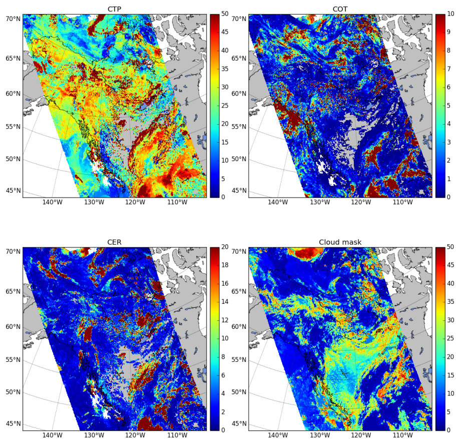
Figure 6. Absolute uncertainties of MODIS AQUA retrieval data for study area NA2 and CTP [hPa], COT, CER [ \mu\text{m} ], and Cloud mask [%].
