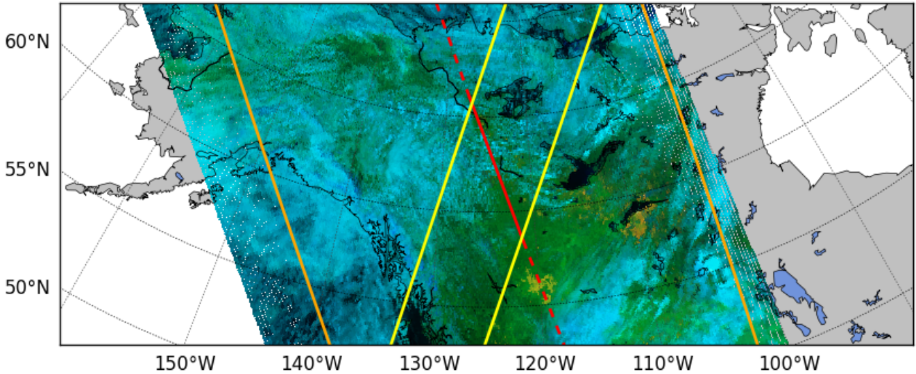
Figure 10. Study area NA2 (North America 2). As Figure 08, but at 07/22/2008, 20:58 LST.
