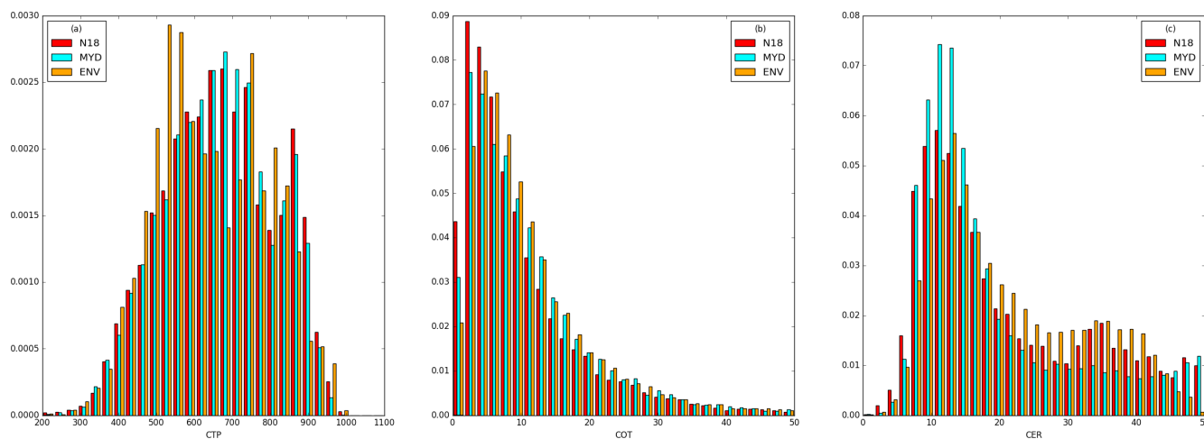
Figure 7. Density histograms of NOAA18 (N18), MODIS AQUA (MYD), and AATSR (ENV) retrieval data for study area NA2 and (a) CTP, (b) COT, and (c) CER.
