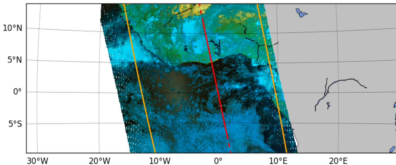
Figure 14. Study area AFR (Africa). As Figure 08, but at 10/24/2009, 13:45 LST.
