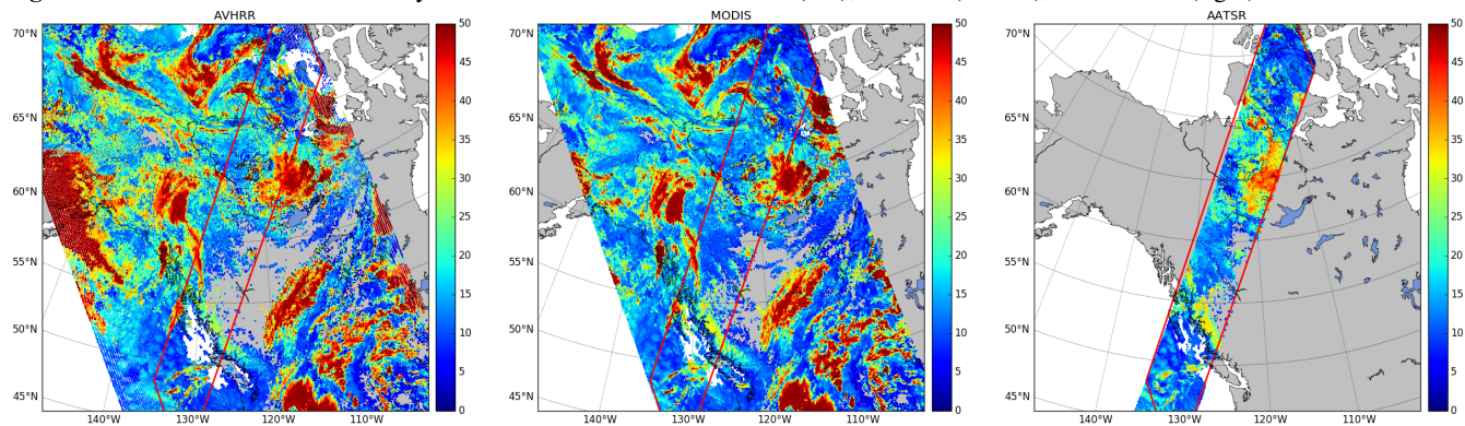
Figure 4. COT retrieval values for study area NA2 with data from AVHRR (left), MODIS (middle), and AATSR (right).
