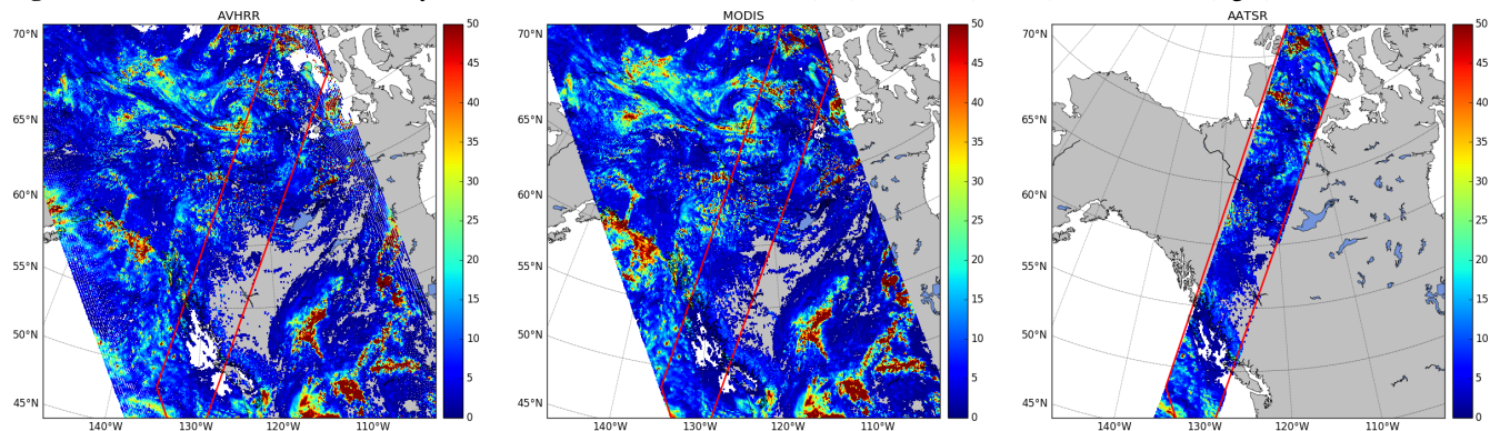
Figure 3. CTP retrieval values for study area NA2 with data from AVHRR (left), MODIS (middle), and AATSR (right).
