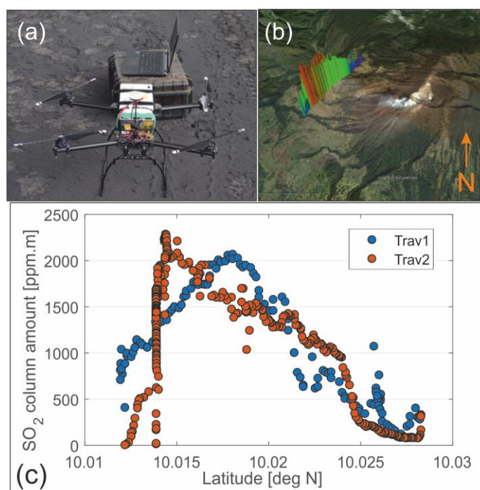
5 Figure 8: (a) Drone-operated miniature DOAS setup, (b) Illustration of SO 2 column amounts measured by DROAS at Turrilaba volcano, (c) SO 2 column amounts during the transversal flight underneath the plume
