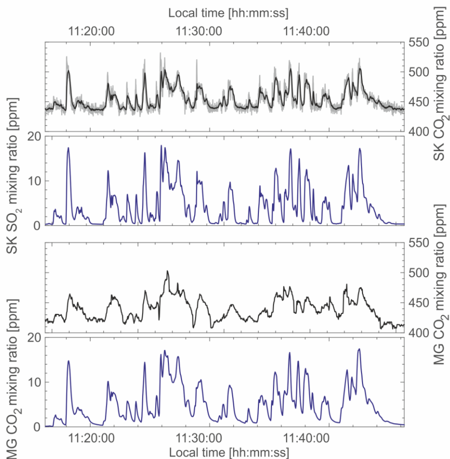
Figure 6: Comparison of SO 2 and CO 2 time series of a Multi-GAS (MG) instrument and the Sunkist (SK) unit at the Masaya volcano crater rim (for SK SO 2 raw data in grey, resampled data in black), both instruments inlets were placed in proximity to each other (14 th July 2016); SK CO 2 /SO 2 = 3.63±0.43 (background CO 2 = 439 ppm); MG CO 2 /SO 2 = 2.94 ± 0.30 (background CO 2 = 413 ppm); (additional scatter plots in the supplementary material)
