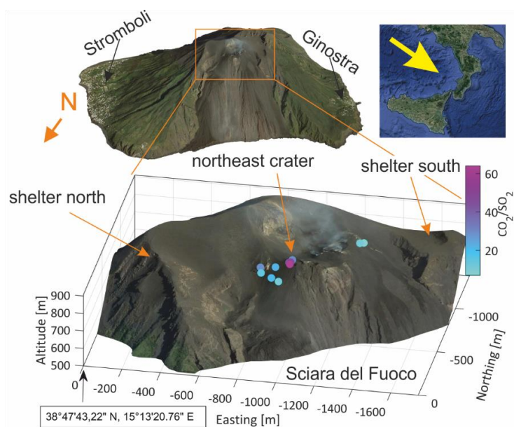
Figure 1: Overview on the sampling site at Stromboli Volcano with the locations of the retrieved \text{CO}_2/\text{SO}_2 mixing ratios given in Table 2
