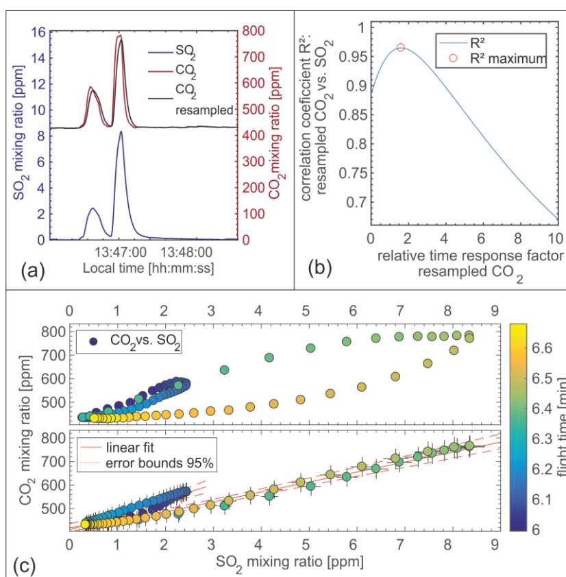
10 Figure 5: (a) Example of time series for mixing ratios of SO 2 and CO 2 (original data in red, resampled data in black), showing discrete gas masses at Stromboli volcano (1st flight on 05 th April 2016), (b) Correlation plot for the determination of the relative time response factor for the CO 2 gas sensor with a maximum at a relative time response factor of 1.7, (c) CO 2 over SO 2 mixing ratios, showing the outcome of the resampling of the fast CO 2 with a relative time response factor of 1.7 (lower plot), linear regression results CO 2 /SO 2 ratios of 64 \pm 16 the first peak and 42 \pm 4 for the second.
