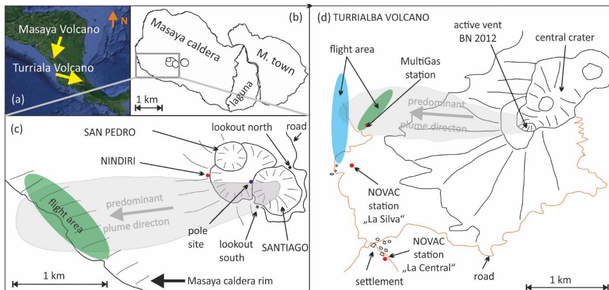
Figure 2: Overview on the field work sites at (a-c) Masaya volcano (Nicaragua) and (d) Turrialba volcano (Costa Rica). Sampling locations mentioned in Table 3 are marked in (c) as follows: Santiago rim, lookout south (black marker); Santiago rim, pole site (blue marker); Nindiri rim (red marker)
