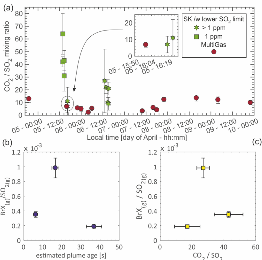
5 Figure 7: (a) Measured CO 2 /SO 2 gas ratios over a 5-day period by a Multi-GAS station (located east of the crater terrace) and airborne measurements with the Sunkist system, data point shapes indicate the lower SO 2 mixing ratio limits for the linear fit over the CO 2 vs SO 2 data, (b) development of the gaseous reactive bromine species over SO 2 over the estimated plume age (derived from distance to crater and estimated wind speed), (c) gaseous reactive bromine/SO 2 ratios vs. CO 2 /SO 2 ratio
