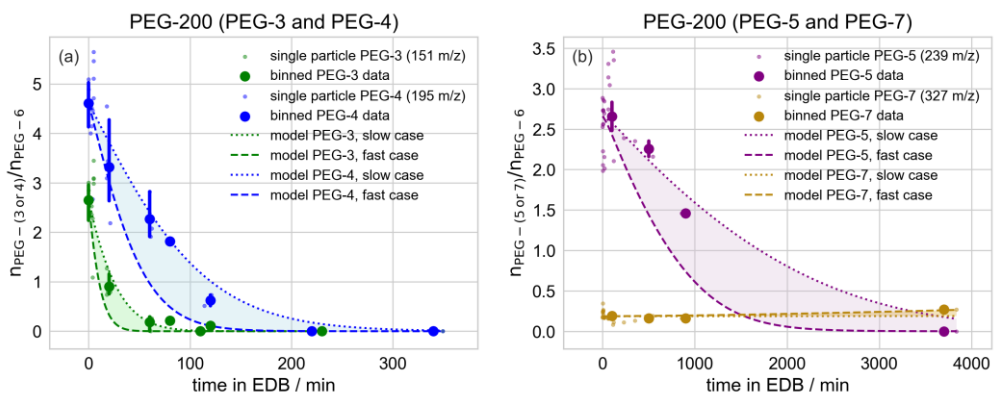
Figure 5: Evaporation of PEG-200 droplets of mixed composition, as in Fig. 4. Here, observations are binned in 10, 20, 50, and 50 min intervals for PEG-3, PEG-4, PEG-5, and PEG-7, respectively. The same data set is used for tracking the evaporation of all PEG molecules; plots are split across two figures ((a): PEG-3 and PEG-4; (b): PEG-5 and PEG-7) due to the significantly differing evaporation timescales.
