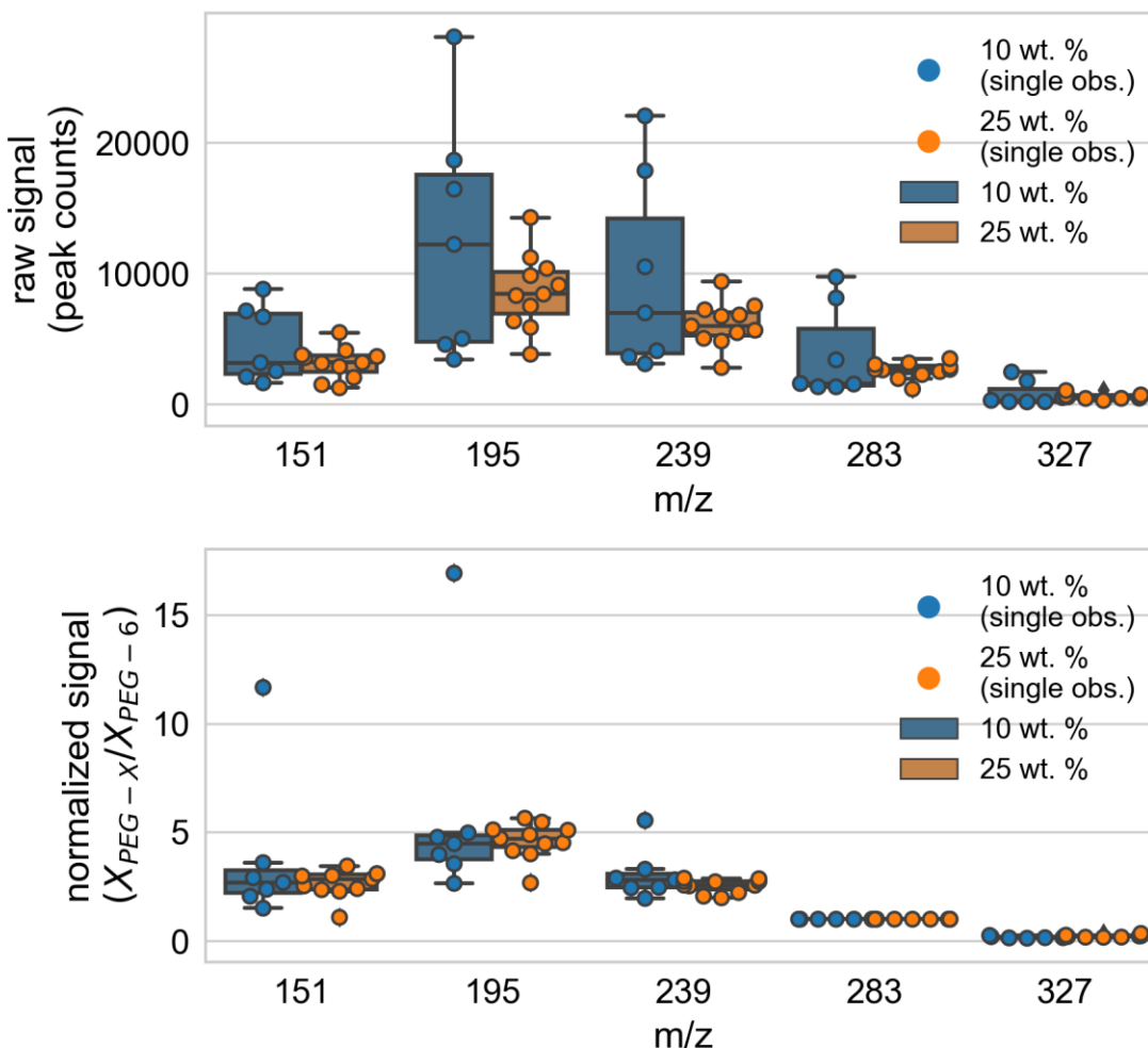
"Figure A1: Analysis of the role of normalization and particle size on particle-to-particle mass spectrum signal variability, comparing particles generated from solutions of 10 and 25 wt. % PEG-200. Top: particle-to-particle raw signal variability. Bottom: particle-to-particle normalized signal variability. Box-and-whisker plots are shown for each tracked m/z (corresponding to PEG-3 through PEG-7), with outliers defined as observations more than 1.5 times the interquartile range beyond the low and high quartiles. Individual observations are overlaid as points (distributed horizontally for clarity)."
