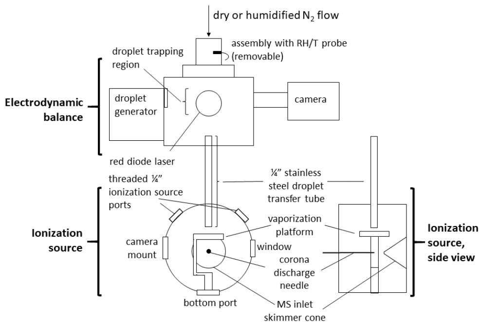
Figure 1: Schematic of experimental setup. A ~140 pL droplet is ejected from the inkjet cartridge, charged, and trapped in the electrodynamic balance (EDB). Once the droplet is ready to be destructively analyzed by the mass spectrometer, it is transferred out of the EDB, down the transfer tube, and to the ionization source. In the ionization source, the droplet strikes the heated vaporized platform (220 °C) and the resulting analyte vapors are drawn toward the mass spectrometer (MS) inlet. The corona discharge from a high-voltage needle ionizes the analyte molecules (positive mode) before the molecules enter the MS. The transfer tube terminates ~4 mm above the vaporization platform. The tip of the corona discharge needle is ~2 cm in front of the MS inlet skimmer cone.
