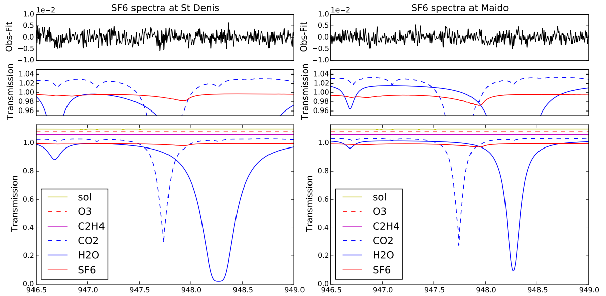
Figure 2. The typical spectrum of SF 6 retrieval microwindow (946.5–949.0 cm −1 ) at St Denis (left) and Maïdo (right). The top panels show the transmittance residual (observed-calculated) , and the bottom panels list the absorption contribution from each species. To clarify the absorption lines, the transmittance is shifted by 0.02 for each species and the solar (sol) line list. The middle panels only show the transmittance between 0.95 and 1.05 to identify the SF 6 absorption line. The top panels show the transmittance residual (observed-calculated).
