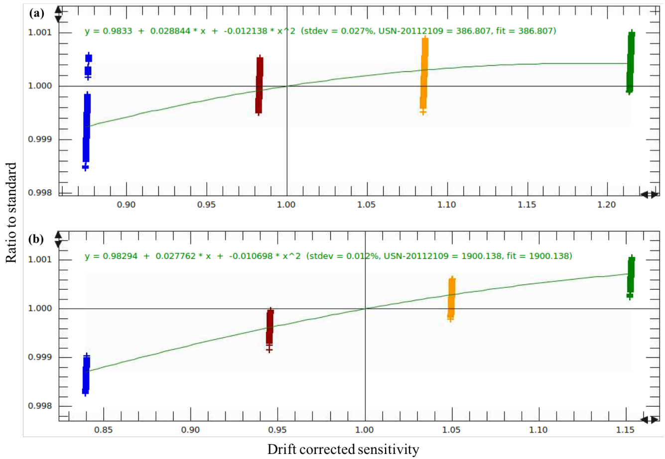
5 Figure 4: An example of a non-linear fit used for (a) CO 2 and (b) CH 4 at TAC from 02/04/2012 to 01/10/2015. Curve coefficients are shown within the plots, along with the standard used (USN-20112109), the assigned values and the adjusted values (fit = ). Drift corrected sensitivity is a function of the measured cylinder dry mole fraction divided by its assigned value, over the measured standard dry mole fraction divided by the assigned/adjusted standard value, as outlined in Eq. 2.
