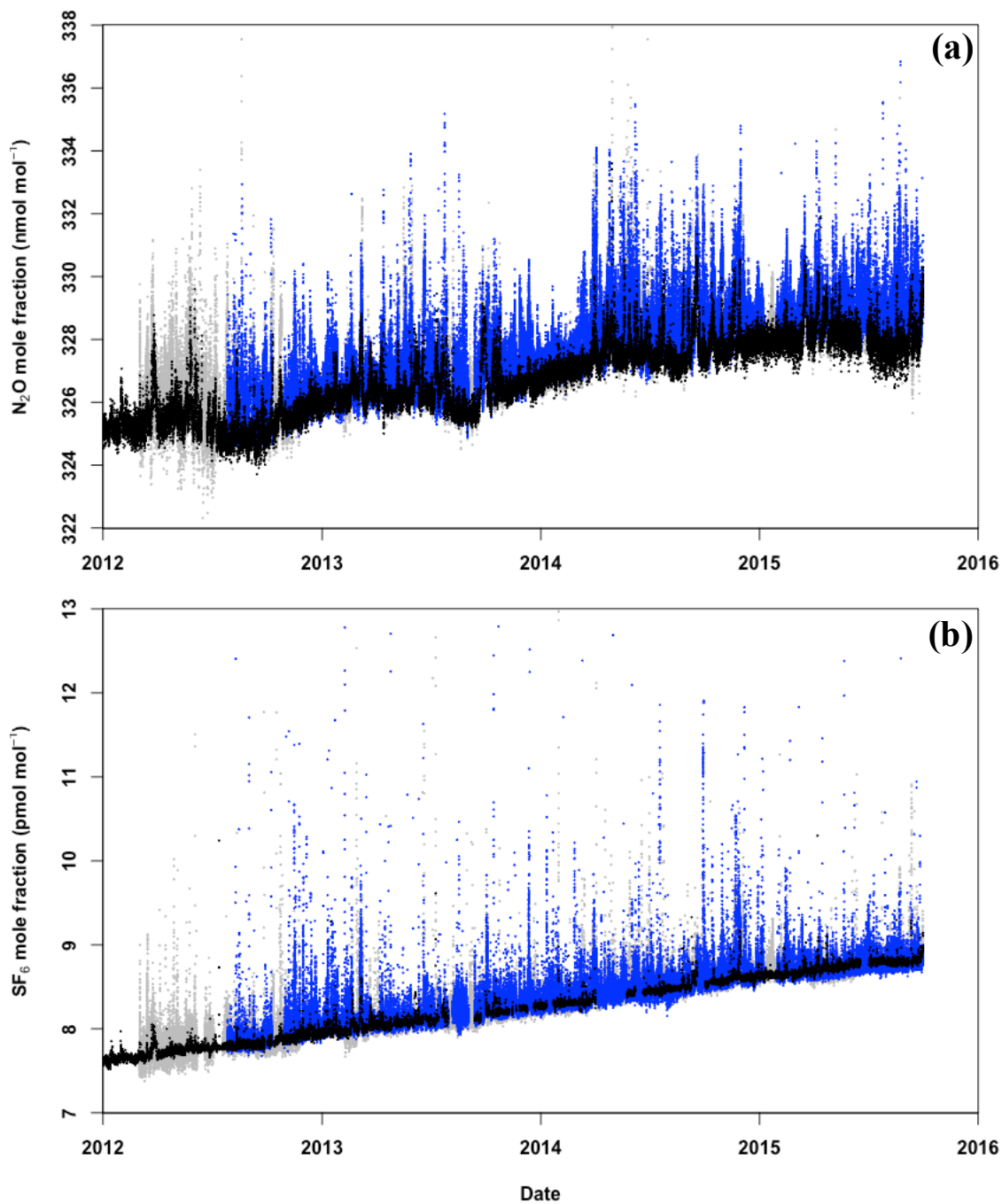
5 Figure 7: Time series of (a) N 2 O and (b) SF 6 mole fractions at MHD (black; 10 m inlet), RGL (grey; 90 m inlet) and TAC (blue; 100 m inlet) from 1 January 2012 to 30 September 2015. All results shown are hourly averages. N 2 O results are shown in nmol mol -1 and are on the SIO-98 scale, whilst SF 6 results are shown in pmol mol -1 and are on SIO-05 scale. SF 6 results from MHD are made using the Medusa GC-MS.
