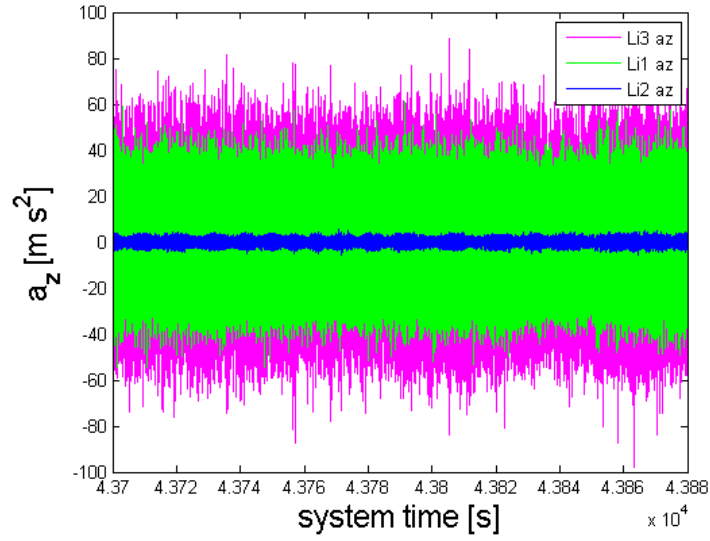
Figure 6. Time series of the accelerations in z direction of the three LICOR sensors during a flight section of 3 min duration on 23 October 2013, illustrating the vibrations the LICOR sensors were exposed to. The flight section took place above agricultural land at 220 m altitude. The acceleration measurements of this flight section are representative for other flight sections at different, but constant altitude. The acceleration measurements at the Li1 are shown in green, at the Li2 in blue, and at the Li3 in magenta. The data were obtained during the part of the flight indicated in yellow in Fig. 3.
