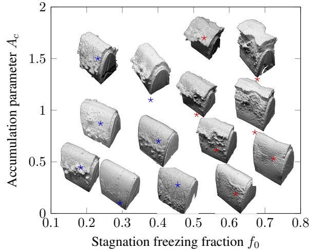
Figure 30. Experimentally observed SLD ice shapes on a NACA0012 leading edge in the parameter space of f_0 and A_c , \text{Re} = 2 \cdot 10^6 , \text{MVD} = 80 \mu\text{m} , \text{AoA} = 0^\circ . Results reproduced from Steiner and Bansmer (2016).
