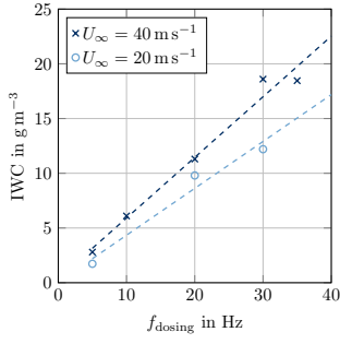
Figure 24. Ice water content depending on dosing frequency f_{\text{dosing}} and injected ice particle flow \dot{m}_{\text{ice,inj}}
