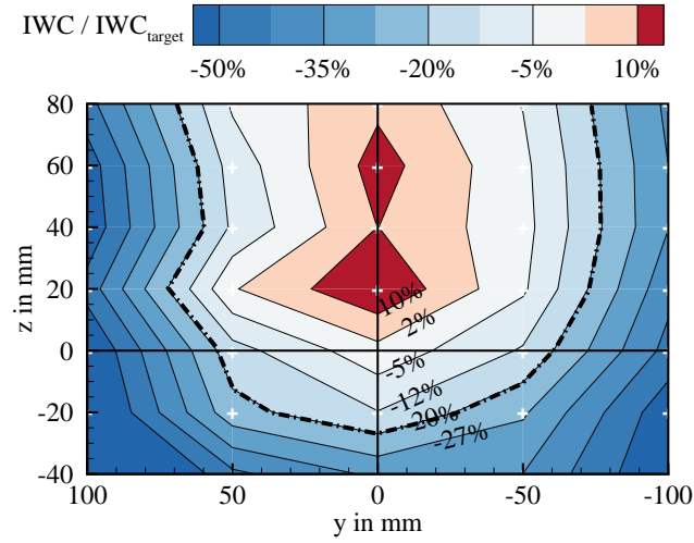
Figure 25. Percentaged deviation of IWC from centerline value, U_\infty = 40 \text{ m s}^{-1} , f_{\text{dosing}} = 20 \text{ Hz} .
