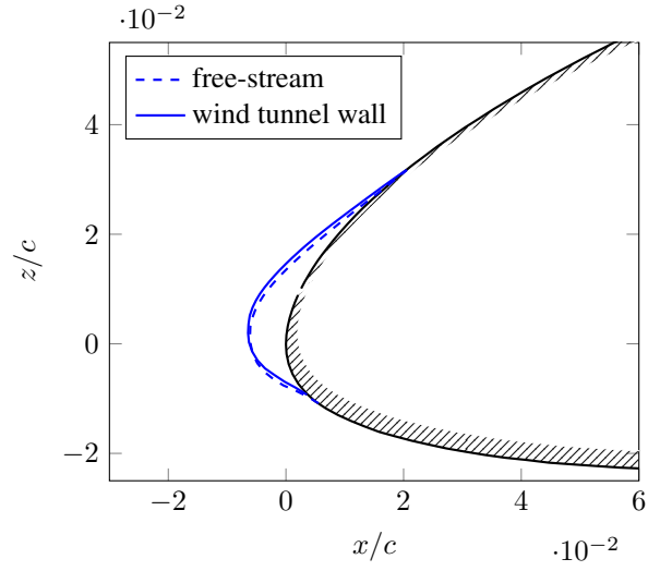
Figure 11. Inviscid wall effect on ice accretion for a AH-94-W-145 airfoil, c = 0.75 m, U_\infty = 40 m s ^{-1} , T_\infty = -10 °C, LWC = 0.3 g m ^{-3} , MVD = 15 \mu m, IWC = 0 .
