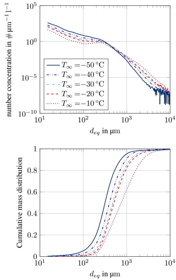
Figure 14. Ice particle size distribution (MMD) based on HAIC Falcon 20 flight measurements from Darwin and Cayenne in dependence on of ambient air temperature.
