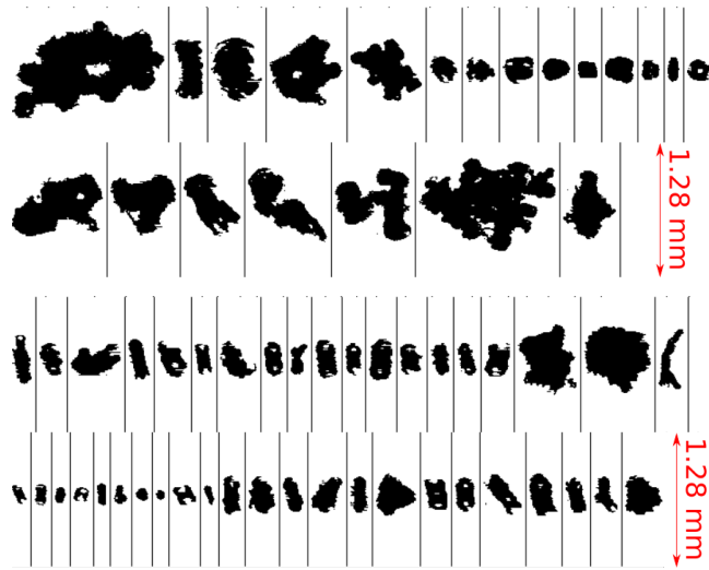
Figure 13. Ice particle images captured by 2D-S probe during the Darwin Campaign. Top: Stratiform cloud region , \text{MMD} \approx 150 \mu\text{m} , \text{IWC} \approx 1.2 \text{ g m}^{-3} , T_{\infty} \approx -10^{\circ}\text{C} . Bottom: Convective cloud region, \text{MMD} \approx 80 \mu\text{m} , \text{IWC} \approx 3 \text{ g m}^{-3} , T_{\infty} \approx -10^{\circ}\text{C} .
