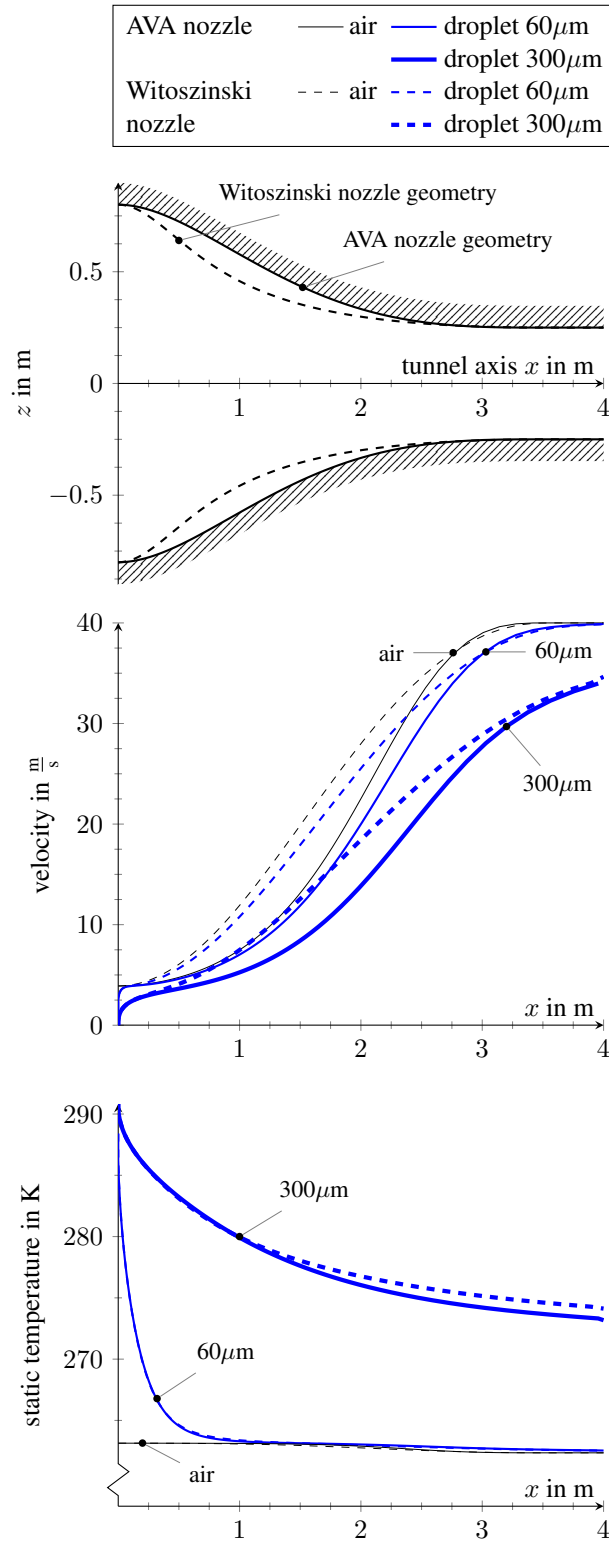
Figure 9. Velocity and temperature slope for air and two different sized droplets inside two tunnel nozzle configurations.
