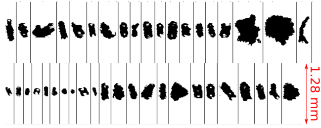
Figure 15. Ice particle images captured by 2DS probe in convective cloud region during the Darwin Campaign, MMD \approx 80\mu m , IWC \approx 3.0g/m^3 , T_\infty \approx -10^\circ C
