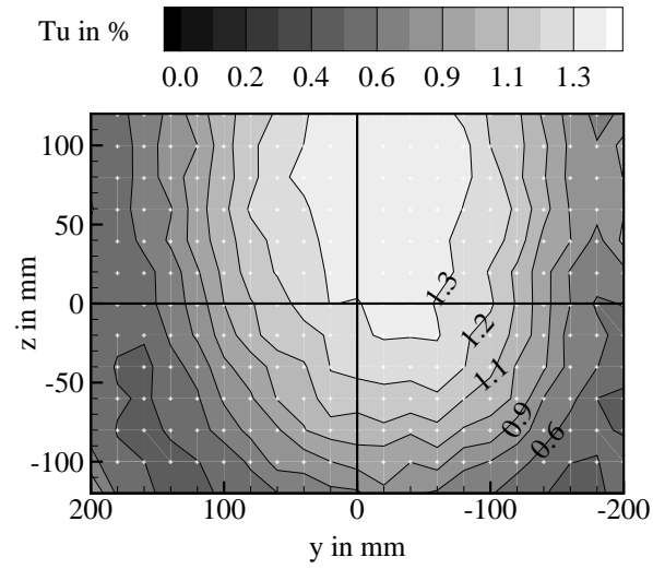
Figure 27. Spatial distribution of turbulence intensity for the mixed phase configuration
