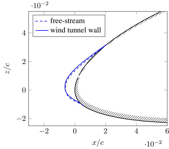
Figure 12. Inviscid wall effect on ice accretion for a AH-94-W-145 airfoil, c=0.75 m, U_\infty=40 m/s, T_\infty = -10 °C, LWC=0.3 g/m 3 , MVD=15 \mu m, IWC=0 .
