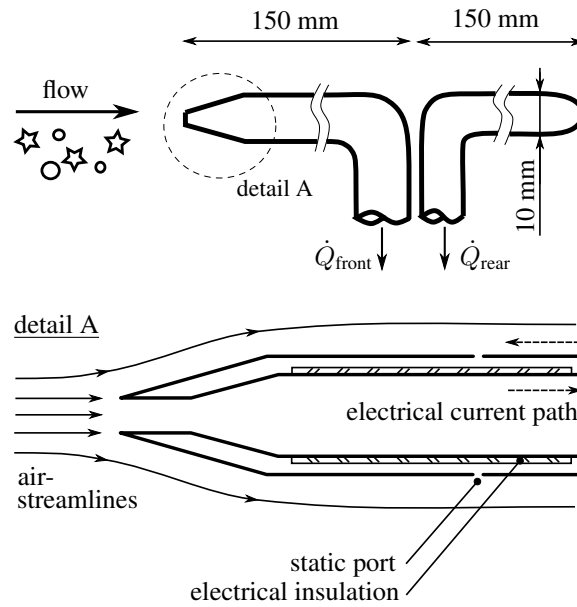
Figure 23. Isokinetic probe to measure the total water content TWC, developed at Cranfield university.
