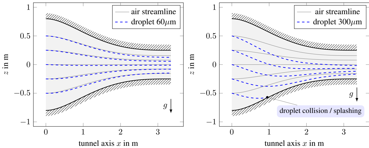
Figure 8. Droplet trajectories in the wind tunnel nozzle and their deviation from the air streamlines under the influence of gravity. Large droplets may collide with the tunnel walls thereby altering the droplet size distribution.
