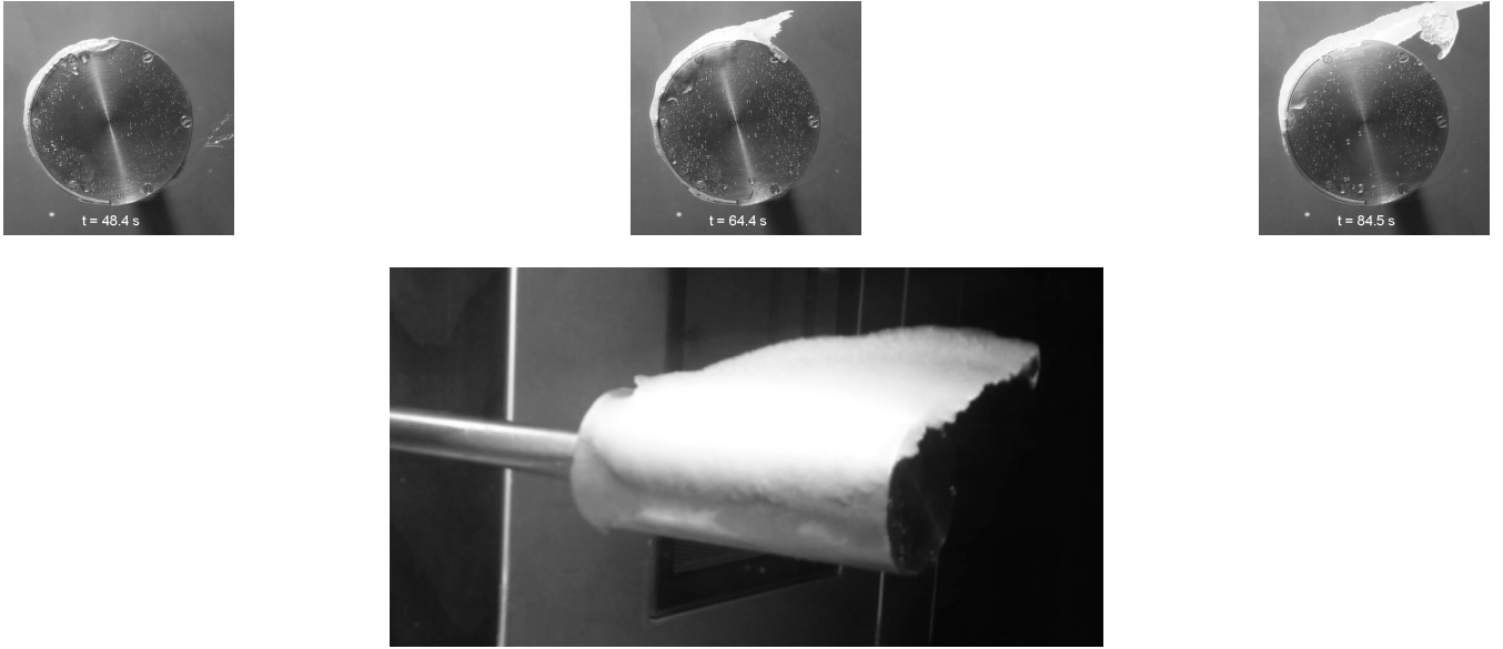
Figure 42. Side view of ice accretion when heating the cylinder, T_{\infty} = -5^{\circ}\text{C} , TWC = 6.8\text{g}/\text{m}^3 and m_r = 0.5
