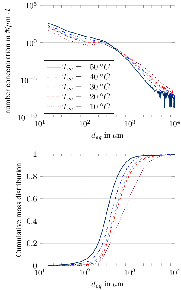
Figure 16. Ice particle size distribution (MMD) based on HAIC Falcon 20 flight measurements from Darwin and Cayenne, dependence on ambient air temperature
