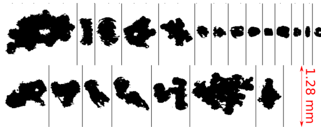
Figure 14. Ice particle images captured by 2DS probe in stratiform cloud region during the Darwin Campaign, MMD \approx 150\mu m, IWC \approx 1.2 g/m 3 , T_\infty \approx -10 °C
