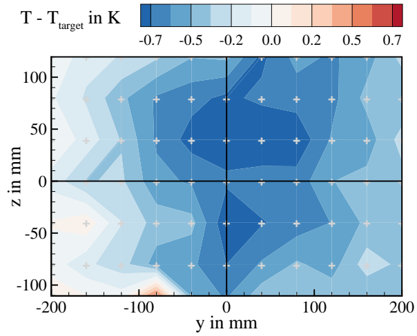
Figure 28. Spatial distribution of temperature variation for the mixed phase configuration
