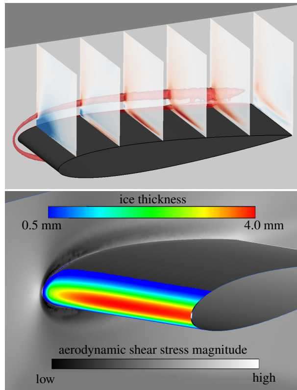
Figure 11. The junction flow between a NACA0012 airfoil ( c = 75 \text{ cm} , \alpha = 0^\circ ) and wind-tunnel side wall creates a horseshoe vortex, which is altering the ice accretion. U_\infty = 40 \frac{\text{m}}{\text{s}} , T_\infty = -10^\circ \text{C} , \text{LWC} = 1 \frac{\text{g}}{\text{m}^3} , \text{IWC} = 0 .
