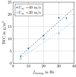
Figure 32. Ice water content depending on dosing frequency f_{\text{dosing}} and injected ice particle flow \dot{m}_{\text{ice,inj}}
