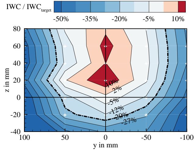
Figure 33. Percentaged deviation of IWC from centerline value, U_\infty = 40 m/s, f_{\text{dosing}} = 20 Hz.
