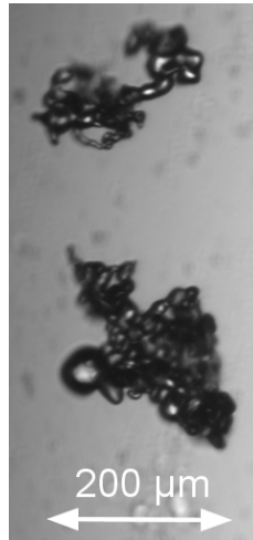
Figure 21. Ice particle structure after storage, dosing and sieving procedure
