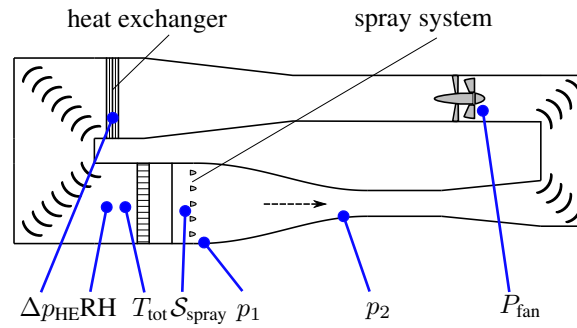
Figure 13. Basic instrumentation of the Braunschweig Icing Wind Tunnel.
