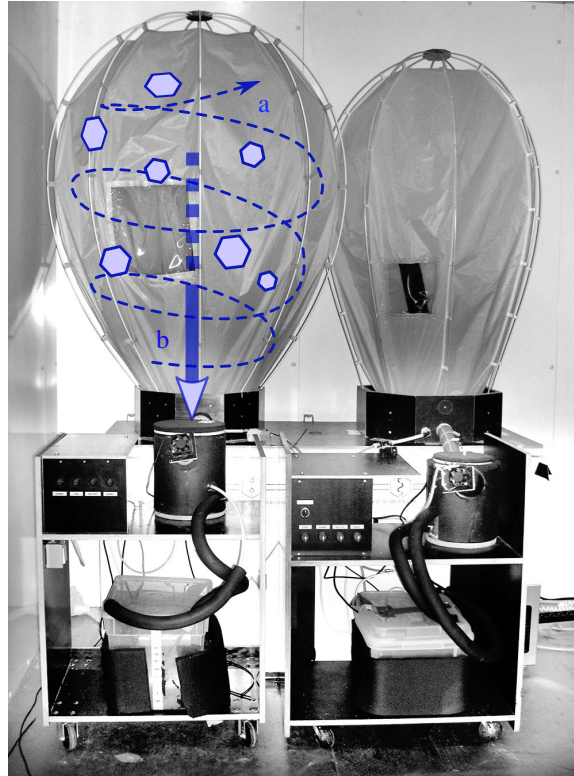
Figure 17. Ice crystal generators. A jet of air (a) circulates the flow allowing for ice crystal growth. When the crystals are large enough, they fall into a chest freezer (b).
