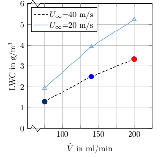
Figure 29. Liquid water content calibration at the tunnel centreline based on IKP measurements. Left: LWC history. Right: LWC depending on supplied water flow-rate.
