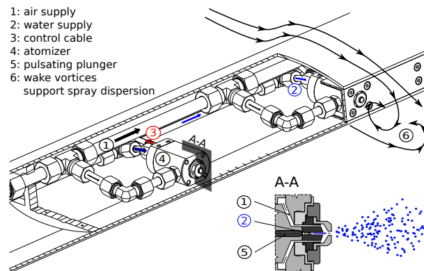
Figure 6. Spray system for low MVD and low LWC.
