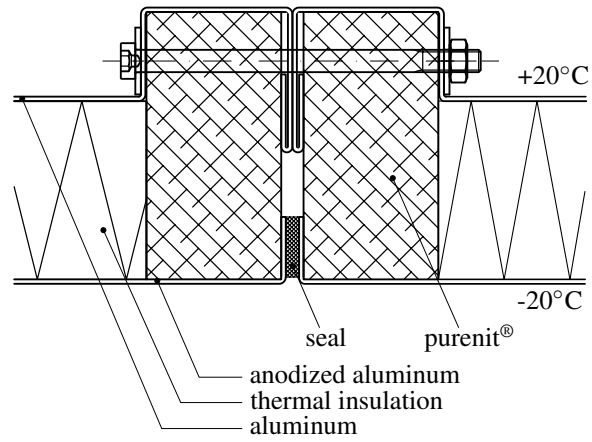
Figure 10. Mechanical design of the icing wind tunnel walls.
