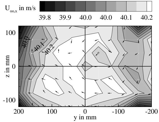
Figure 26. Spatial distribution of axial flow velocity U_{\infty,x} , for the standard setup.
