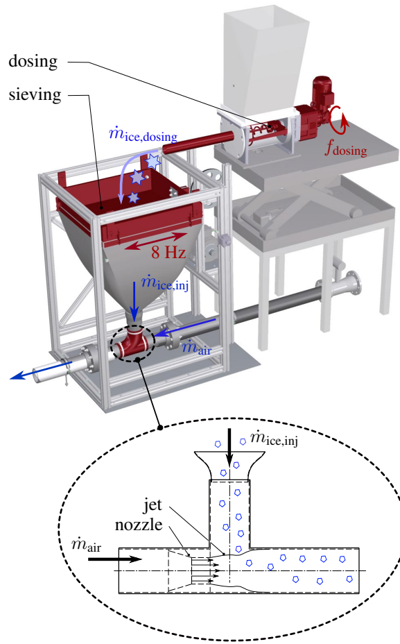
Figure 19. Assembly for ice particle dosing and fluidization.
