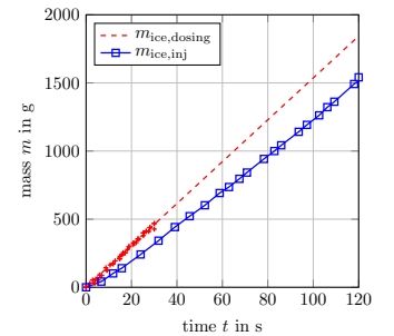
Figure 20. Ice particle massflow. Left: Dependence on dosing machine frequency. Right: Ice particle supply over time at a dosing frequency of f_{\text{dosing}} = 21 Hz.
