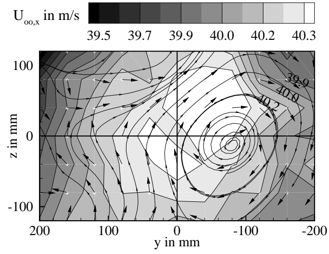
Figure 25. Spatial distribution of axial flow velocity U_{\infty,x} , for the ice-crystal-icing setup.
