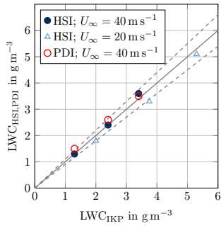
Figure 23. Comparison of HSI, PDI and IKP measurements for supercooled droplet conditions. Left: Optical array probes vs. IKP. Right: MVD vs. LWC.
