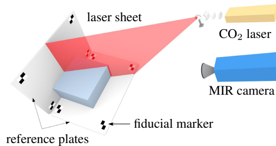
Figure 35. Infrared laser line scanning technique. The mid-infrared camera records the distorted \text{CO}_2 -laser line on the ice surface. With a prior calibration, the 3D geometry of the object can be reconstructed. Image reproduced from Gong and Bansmer (2015a).
