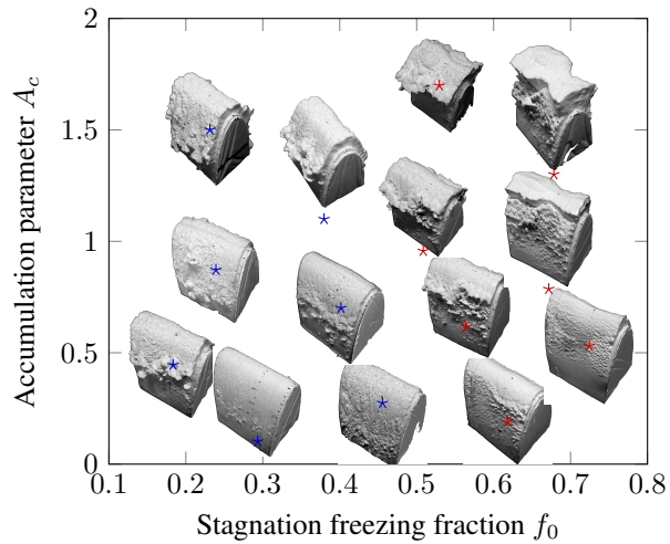
Figure 32. Experimentally observed SLD ice shapes on a NACA0012 leading edge in the parameter space of f_0 and A_c , Re=2 \cdot 10^6 , MVD=80 \mu m , AoA=0^\circ . Results reproduced from Steiner and Bansmer (2016).
