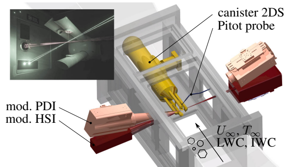
Figure 27. Setup of the probe inter-comparison exercise. Alternatively to the canister 2D-S probe, which is shown here, the canister HSI probe was mounted. Upper left: C-HSI probe mounted inside the icing wind tunnel, modular PDI and HSI laser beams are adjusted close to the C-HSI sampling volume
