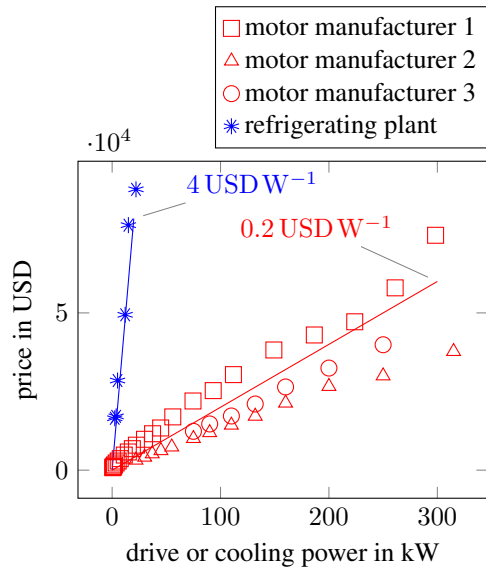
Figure 3. Pricing as of 2017 for asynchronous motors from different manufacturers and for CO 2 refrigerating plants before tax and tolls.
