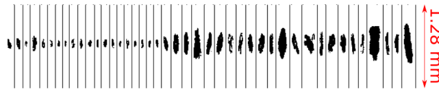
Figure 30. Ice particle images captured by the 2D-S probe inside the Braunschweig Icing Wind Tunnel test section, MMD = 79 \mu\text{m} , IWC = 3.2 \text{gm}^{-3} , T_\infty = -15^\circ\text{C}
