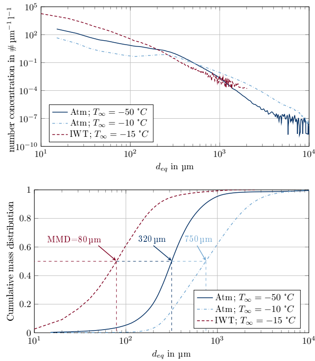
Figure 31. Comparison of artificial ice particle cloud to atmospheric cloud conditions. Top: Particle size distribution. Bottom: Cumulative particle size distribution.
