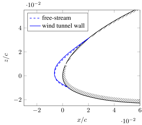
Figure 11. Inviscid wall effect on ice accretion for a AH-94-W-145 airfoil, c = 0.75 m, U_\infty = 40 \text{ms}^{-1} , T_\infty = -10 ^\circ\text{C} , \text{LWC} = 0.3 \text{g m}^{-3} , \text{MVD} = 15 \mu\text{m} , \text{IWC} = 0 .
