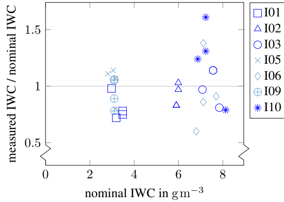
Figure 28. Results of the probe intercomparison between 2D-S (LAMP), 2D-S (DLR), M-HSI, C-HSI for seven different test points at glaciated icing conditions
