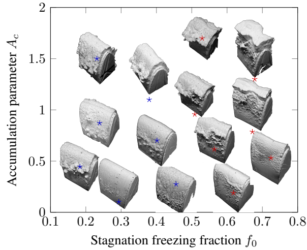
Figure 30. Experimentally observed SLD ice shapes on a NACA0012 leading edge in the parameter space of f_0 and A_c , \text{Re}=2 \cdot 10^6 , \text{MVD}=80 \mu\text{m} , \text{AoA}=0^\circ . Results reproduced from Steiner and Bansmer (2016).
