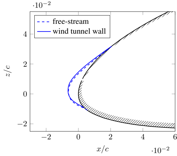
Figure 11. Inviscid wall effect on ice accretion for a AH-94-W-145 airfoil, c = 0.75 m, U_\infty = 40 m s ^{-1} , T_\infty = -10 °C, LWC=0.3 g m ^{-3} , MVD=15 \mu m, IWC=0.
