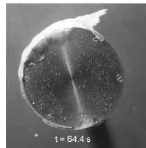
Figure 32. Side view of ice accretion when heating the cylinder, T_{\infty} = -5\text{ }^{\circ}\text{C} , \text{TWc}=6.8\text{ g m}^{-3} and m_r = 0.5 .
