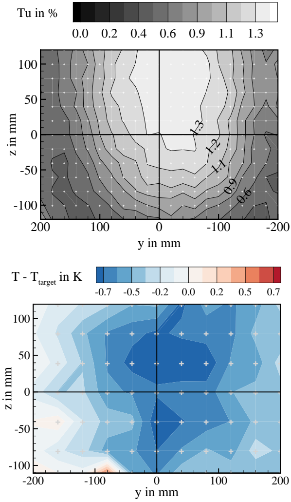
Figure 20. Spatial distribution of turbulence intensity ( top ) and temperature variation ( bottom ) for the mixed phase configuration.
