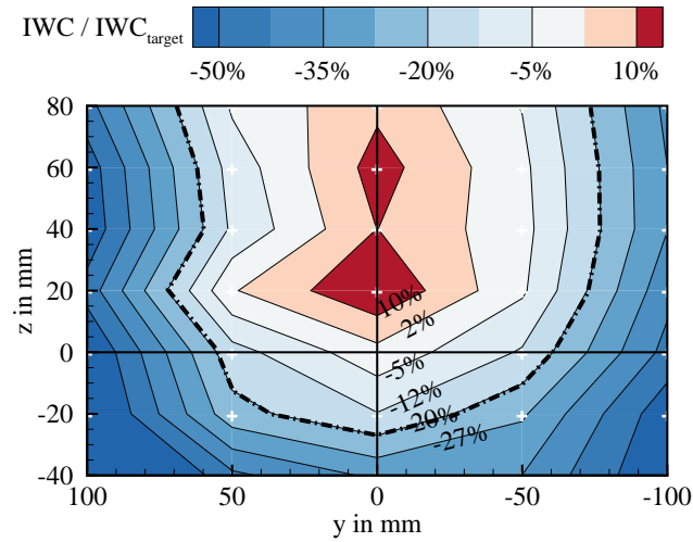
Figure 25. Percentaged deviation of IWC from centerline value, U_\infty=40\ m\ s^{-1} , f_{dosing}=20\ Hz .
