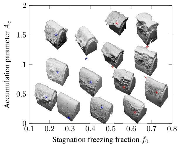
Figure 30. Experimentally observed SLD ice shapes on a NACA0012 leading edge in the parameter space of f_0 and A_c , Re=2 \cdot 10^6 , MVD=80 \mu m , AoA=0^\circ . Results reproduced from Steiner and Bansmer (2016).
