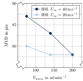
Figure 22. Comparison of HSI, PDI and IKP measurements for supercooled droplet conditions. Left: Optical array probes vs. IKP. Right: MVD vs. volumetric flow rate of liquid water at the spray system.
