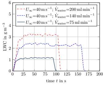
Figure 21. Liquid water content calibration at the tunnel centreline based on IKP measurements. Left: LWC history. Right: LWC depending on supplied water flow-rate \dot{V}_{\text{water}} .
