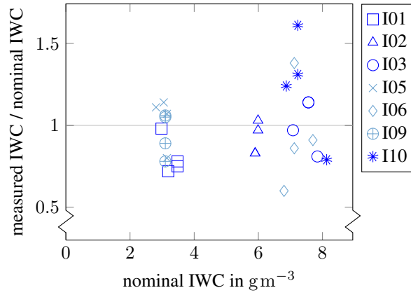
Figure 27. Results of the probe intercomparison between 2D-S (LAMP), 2D-S (DLR), M-HSI, C-HSI for seven different test points at glaciated icing conditions.
