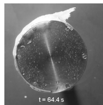
Figure 32. Side view of ice accretion when heating the cylinder, T_{\infty} = -5^{\circ}\text{C} , \text{TWC}=6.8\text{ g m}^{-3} and m_r = 0.5 .
