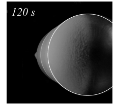
Figure 31. Side view of ice accretion shapes on a cylinder for \text{TWC}=12\text{ g m}^{-3} , m_r = 0.12 and U_{\infty} = 40\text{ m s}^{-1} , with a variation of temperature.
