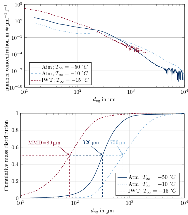
Figure 29. Comparison of artificial ice particle cloud to atmospheric cloud conditions. Top: Particle size distribution. Bottom: Cumulative particle size distribution.
