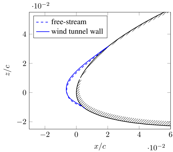
Figure 11. Inviscid wall effect on ice accretion for a AH-94-W-145 airfoil, c = 0.75 \text{ m} , U_\infty = 40 \text{ m s}^{-1} , T_\infty = -10^\circ \text{C} , \text{LWC} = 0.3 \text{ g m}^{-3} , \text{MVD} = 15 \mu\text{m} , \text{IWC} = 0 .
