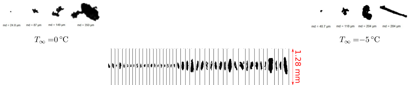
Figure 28. Ice particle images captured at the test section of the Braunschweig Icing Wind Tunnel. Top: Images taken by C-HSI probe. Bottom: Images taken by 2D-S probe, MMD = 79 \mu\text{m} , IWC = 3.2 \text{g m}^{-3} , T_\infty = -15^\circ\text{C} .
