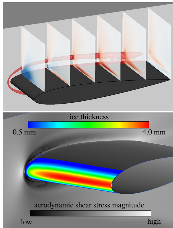
Figure 10. The junction flow between a NACA0012 airfoil ( c = 0.75 m, \alpha = 0^\circ ) and wind-tunnel side wall creates a horseshoe vortex (upper image), which is altering the ice accretion (lower image). U_\infty = 40 \text{ m s}^{-1} , T_\infty = -10^\circ \text{C} , \text{LWC} = 1 \text{ g m}^{-3} , \text{IWC} = 0 .
