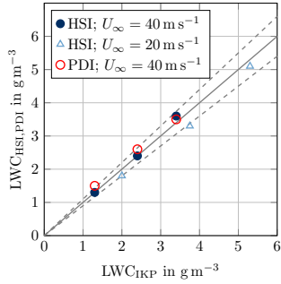
Figure 22. Comparison of HSI, PDI and IKP measurements for supercooled droplet conditions. Left: Optical array probes vs. IKP. Right: MVD vs. volumetric flow rate of liquid water at the spray system.
