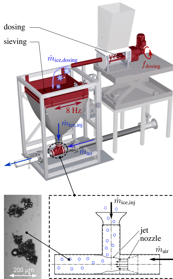
Figure 16. Assembly for ice particle dosing and fluidization. Ice particle structure after storage, dosing and sieving procedure.
