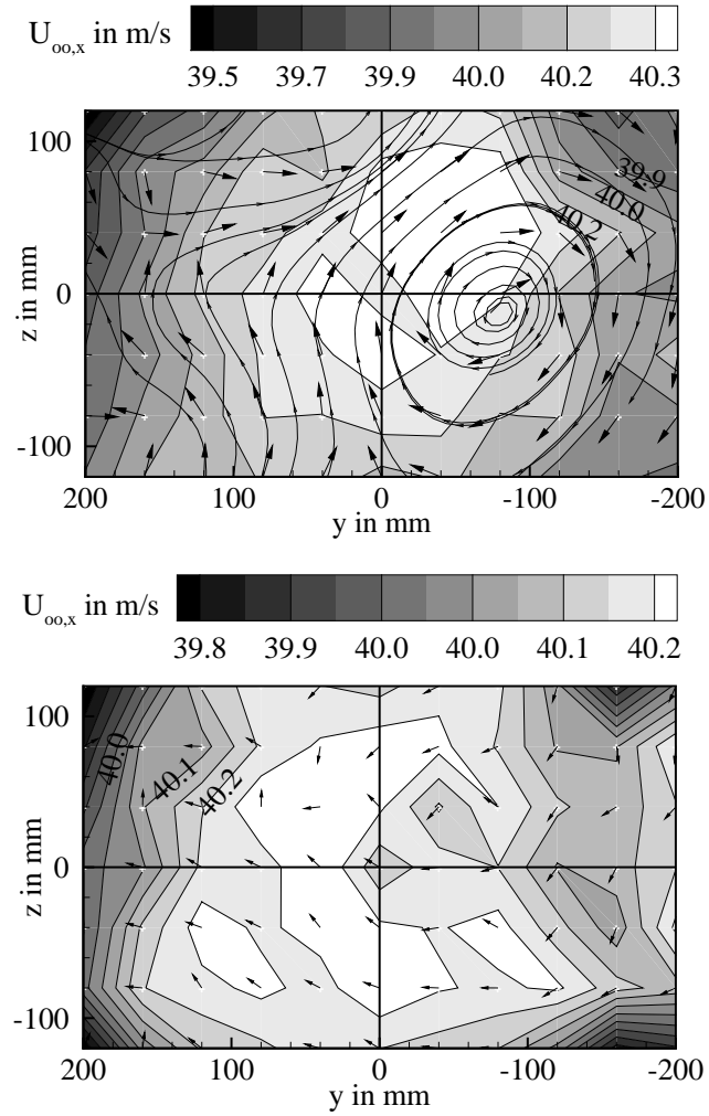
Figure 19. Spatial distribution of axial flow velocity U_{\infty,x} . Top: ice-crystal-icing setup. Bottom: standard setup of the icing wind tunnel.
