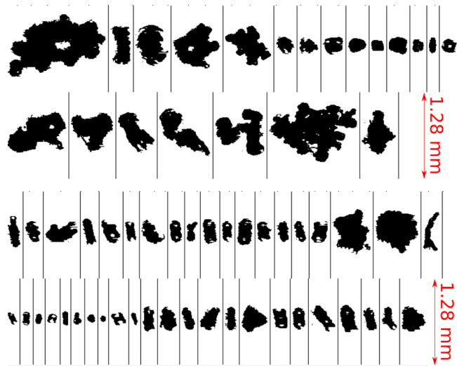
Figure 13. Ice particle images captured by 2D-S probe during the Darwin Campaign. Top: Stratiform cloud region , MMD \approx 150 \mu\text{m} , IWC \approx 1.2 \text{ g m}^{-3} , T_\infty \approx -10^\circ\text{C} . Bottom: Convective cloud region, MMD \approx 80 \mu\text{m} , IWC \approx 3 \text{ g m}^{-3} , T_\infty \approx -10^\circ\text{C} .
