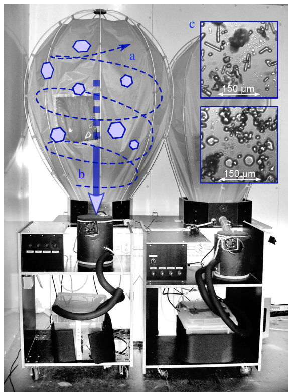
Figure 15. Ice crystal generators. A jet of air (a) circulates the flow allowing for ice crystal growth. When the crystals are large enough, they fall into a chest freezer (b). Microscopic images of ice particles inside the cloud chambers (c). Both plate crystals and needles can be generated.
