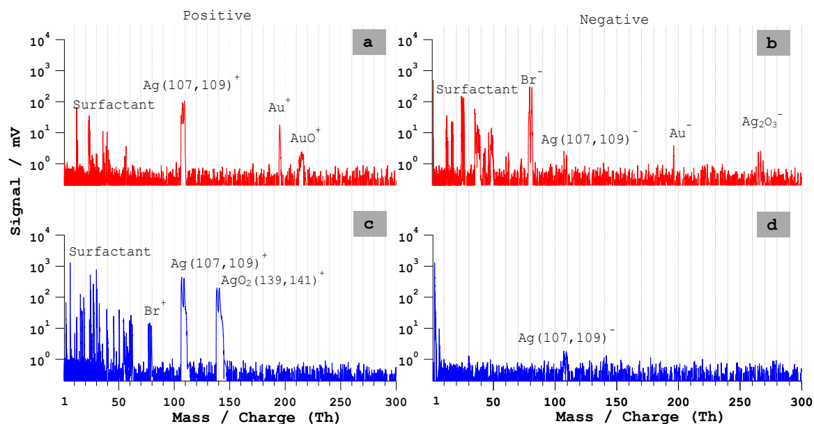
Figure 7: Bipolar mass spectra of gold-silver core-shell particles of d_p = 600 nm. a – b: Typical ns-LAAPTOF spectra; c – d: fs-LAAPTOF ( \lambda = 800 nm) spectra. The pulse energy is 4 mJ for the ns-laser and 3.2 mJ for the fs-laser.
