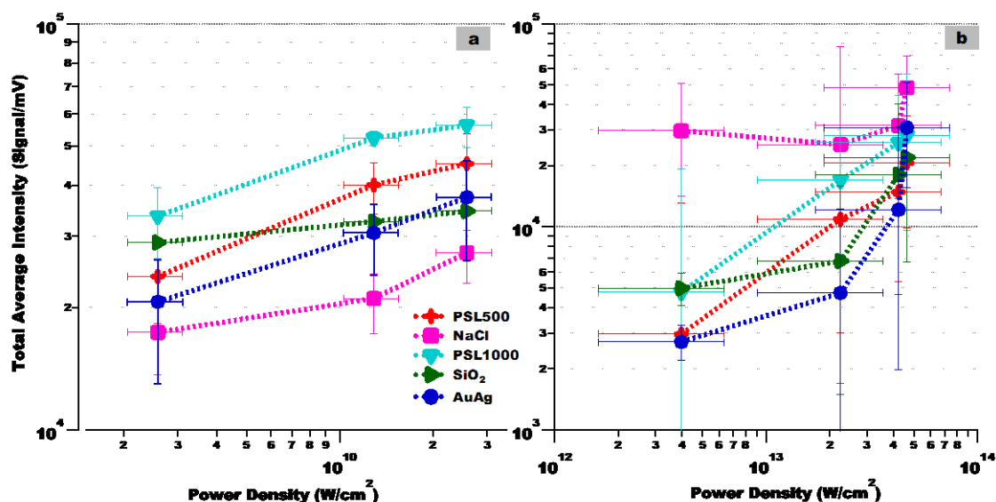
Figure 9: Average ion intensity versus laser power density for different particle types. (a) Excimer laser, (b) fs-laser. Error bars of the average ion signal intensity correspond to \pm 1 standard deviation, error bars of the power density to the value of power density of the laser beam at the corresponding possible maximum and minimum position of particle-laser interaction.
