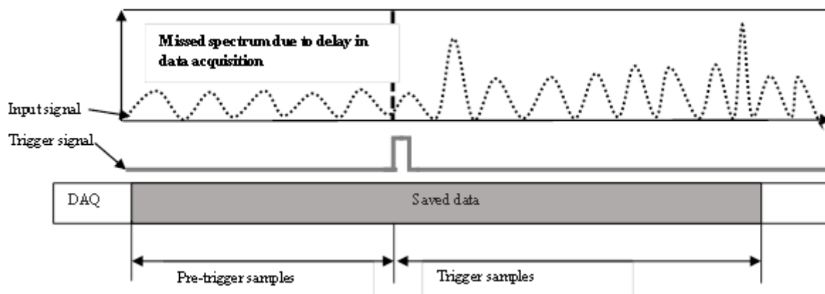
790 Figure 2: Pre-trigger sampling mechanism of the data acquisition system. The data (input signal, the dotted wavy line) arriving before the trigger event (pre-trigger samples) are saved in the temporary memory of the data acquisition card and then combined with the trigger samples.
