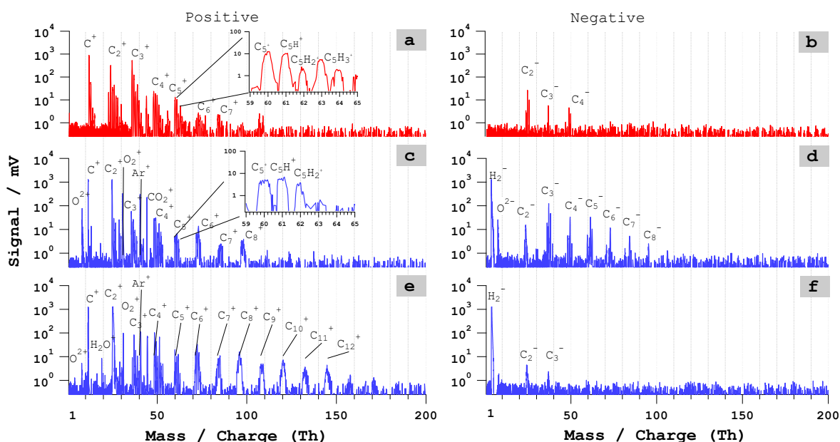
795 Figure 3: Bipolar mass spectra of single PSL particles of d_p = 500 nm. a – b: Typical ns-laser spectra; c – d: fs-laser ( \lambda = 800 nm) spectra for 54 % of particles (type 1); e – f: fs-laser ( \lambda = 800 nm) spectra for 42 % of particles (type 2). The pulse energy is 4 mJ for the ns-laser and 3.2 mJ for the fs-laser.
