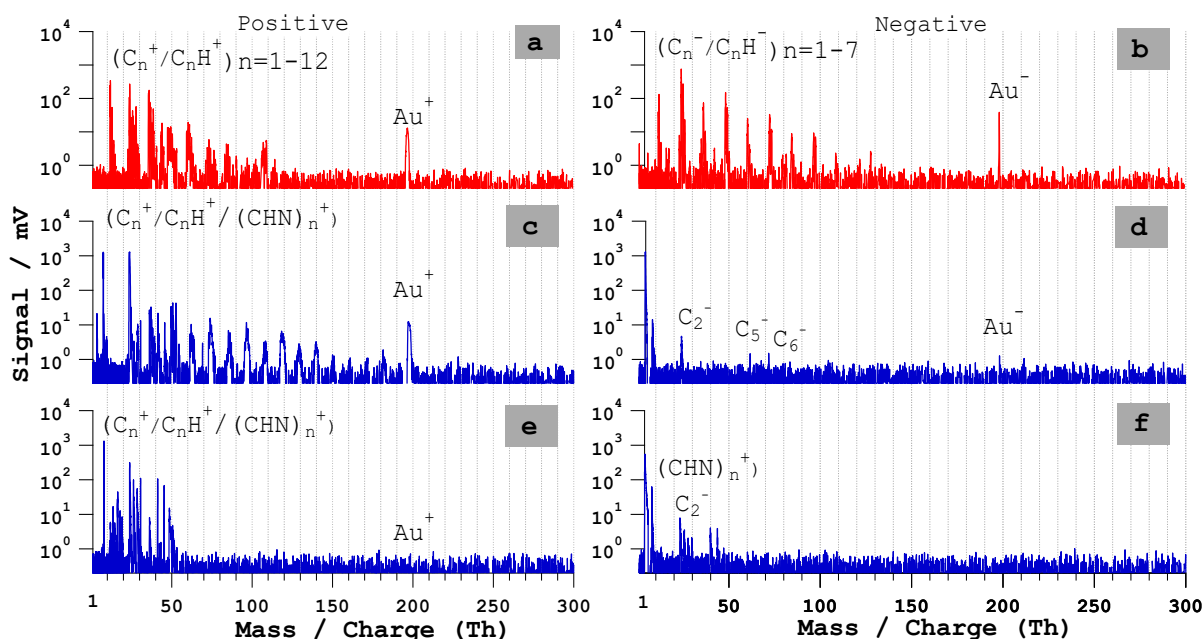
Figure 8: Bipolar mass spectra of Au-PAH core-shell particles. a – b: Typical ns-LAAPTOF spectra; c – d: fs-LAAPTOF ( \lambda = 800 nm) spectrum that contains both gold and PAH signal, e-f: fs-LAAPTOF ( \lambda=800 nm) spectrum without gold signal. The pulse energy is 4 mJ for the ns-laser and 3.2 mJ for the fs-laser.
