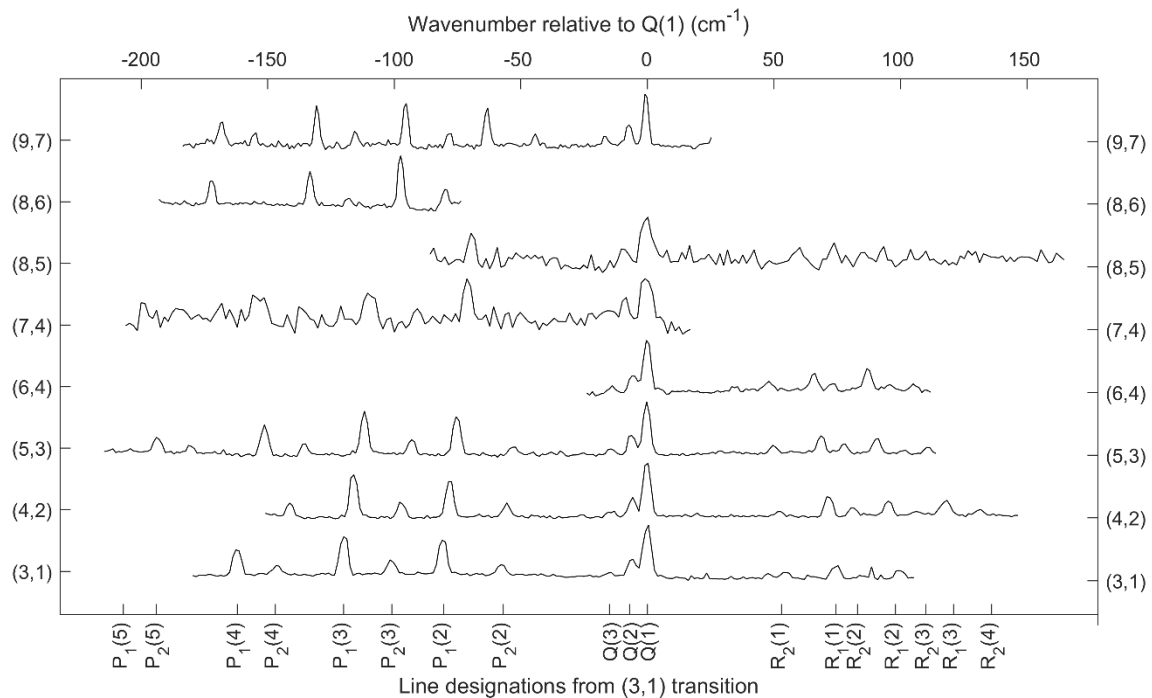
5 Figure 4: Spectra from the H -, J - and K -bands in wavenumbers relative to the Q(1) line in each band. The Q(1) lines of each spectrum are aligned. Line positions for the (3,1) transition are shown..
