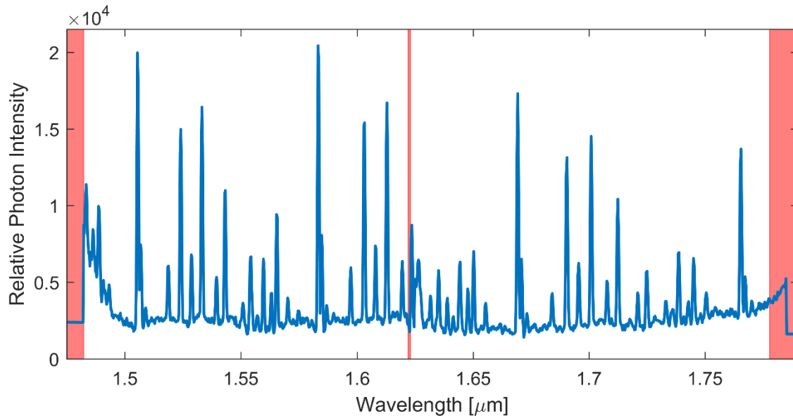
10 Figure 2: H -band spectrum of atmospheric OH extracted from the data frame presented in Fig. 1. Red shading highlights parts of the spectrum not used in the subsequent rotational temperature fitting.
