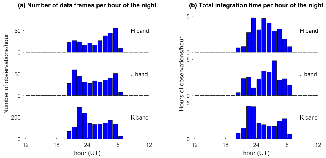
Figure 7: (a) Total number of spectroscopic data frames recorded in each hour and each band with NOTCam between November 2007 and June 2016. (b) Total hours of on-target integration time for spectroscopic data recorded in each hour and each band with the NOTCam in the same period of time.
