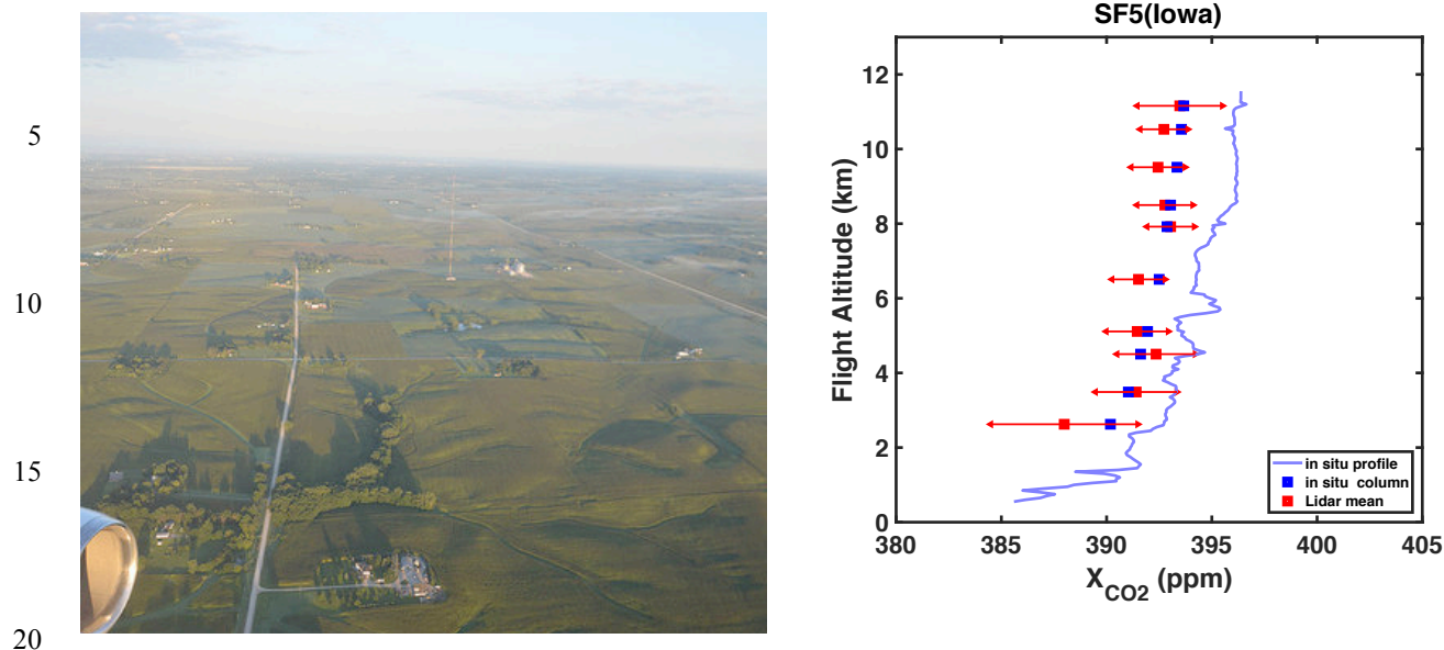
Figure 21 – (Left) Photo of the Iowa topography and the West Branch tower taken from the aircraft on 2014 SF5. (Right) Summary of the in situ (blue) and the retrievals from the lidar measurement (red) versus altitude. The lidar results are for retrievals based on 10-s average from the altitude where the results are plotted, and the error bars are for 1 standard deviation. The X_{CO_2} computed from the in situ sensor from the plotted altitude to the ground are shown as the blue dots. The in situ sensor shows the drawdown in CO_2 concentrations at lower altitudes caused by cropland, and that general trend is seen in the X_{CO_2} values computed from in situ and in lidar retrievals.
