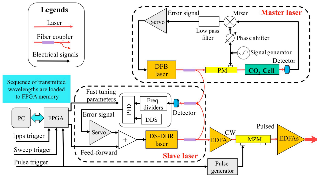
Figure 2- Instrument block diagram for the 2014 and 2016 versions of the CO 2 Sounder lidar described here. The inset shows the transmitted pulse train sequence that is repetitively stepped in wavelength across the CO 2 line.
