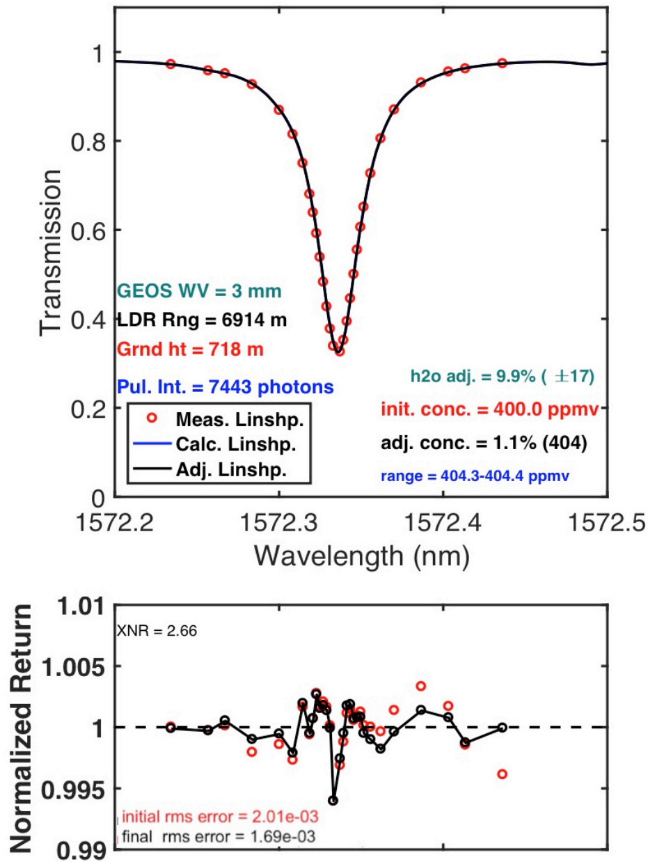
Figure 9 – (Upper plot) Example of the CO 2 transmission line shape measured by the lidar from an altitude of 7.6 km. The line shape samples from the lidar are the red dots. The line shape computed from the retrieval is shown as the black line. (Lower plot) The ratio of the retrieved line shape and lidar retrievals with the red dots being the initial trial XCO 2 value of 400 ppm and the black dots and line being the final best fit retrieved XCO 2 value of 404 ppm.
