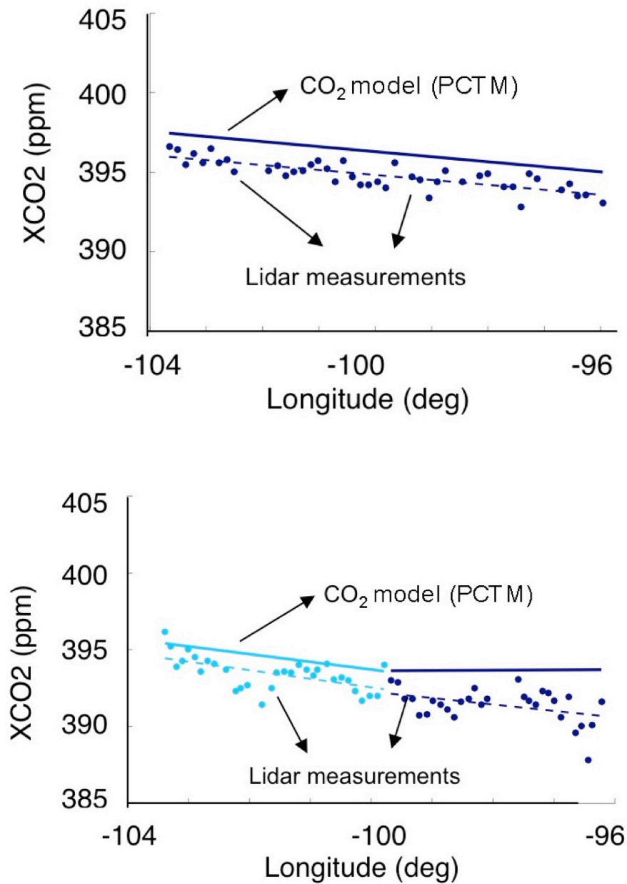
Figure 18 – Retrieved XCO 2 from lidar measurements vs longitude for the transit flights to/from Colorado to Iowa on 2014 SF3. ( Top ) Outbound leg (West to East flight direction, SF3G1, measured from 11.2 km altitude) and ( Bottom ) Return flight leg (East to West flight direction, SF3G2, with dark blue points measured from 5.6 km altitude and light blue points from 6.3 km altitude). The measurements shown are for retrievals using 50-s data averages, and the flight altitudes are indicated. The solid lines show the XCO 2 values computed from the PCTM atmospheric model for that location and these times.
