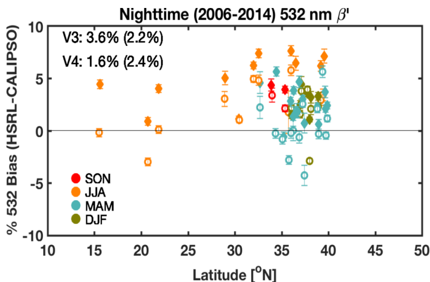
Figure 17. Difference between HSRL and CALIOP attenuated backscatter measurements for nighttime clear-air profiles as a function of latitude. The data are colored by the season of measurement. V3 differences are shown as filled diamonds and the corresponding V4 differences are shown as open circles. The error bars for each point represent the standard deviation of the mean.
