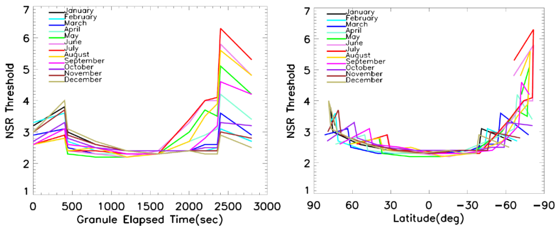
Figure 5. The NSR thresholds employed in V4 algorithm for various months (same for all years) as a function of granule elapsed time (left panel) and latitude (right panel).
