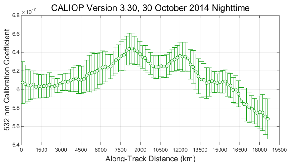
5 Figure 4. Mean 532 nm calibration coefficients ( \text{km}^3 \text{sr} ) as a function of orbit along-track distance computed for all nighttime data acquired on 30 October 2014. The peaks in the curve at \sim 8250 km and \sim 12000 km are the result of aerosol contamination in the 30–34 km calibration region. The marked drop-off beginning just after 15000 km is attributed to thermal beam steering caused by warming as the satellite first enters the sunlit portion of the orbits.
