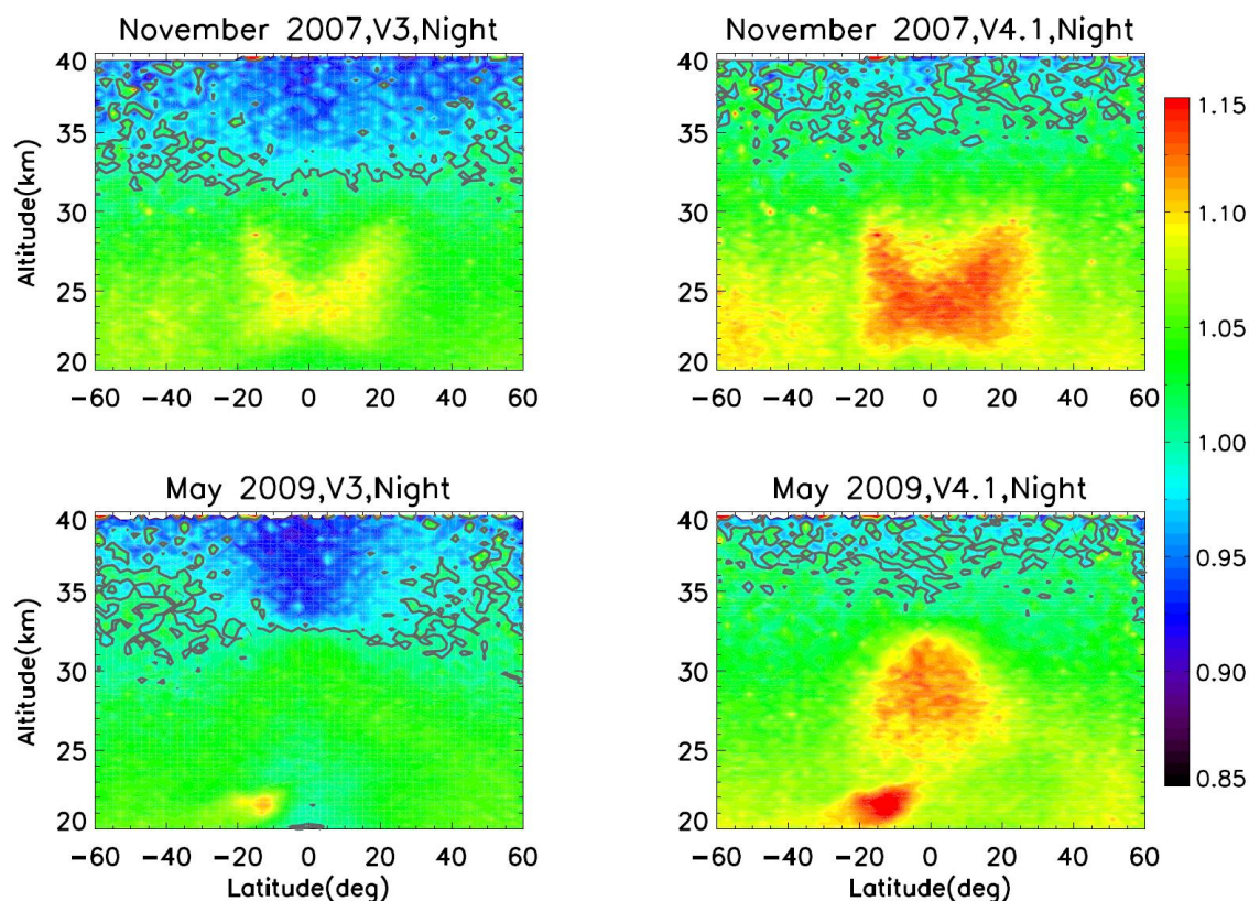
5 Figure 16. Zonally averaged height latitude cross sections of R' calculated using V3 and V4 level 1 data for November 2007 (top two panels) and for May 2009 (bottom two panels). The contour lines shown are for R'=1 .
