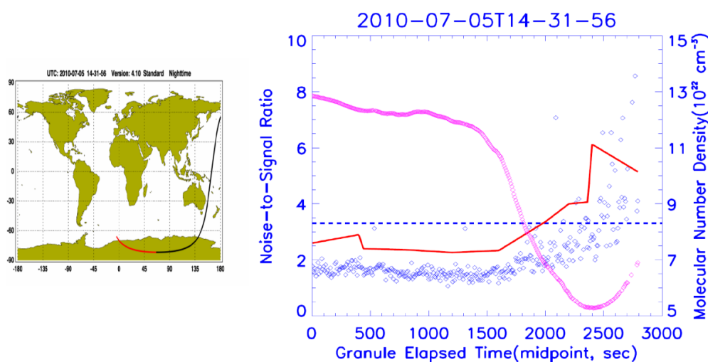
Figure 6. Noise-to-signal ratio (blue diamonds) for a single granule (orbit track shown in the left panel) showing the effect of V3 (blue dashed line) and V4 (red line) thresholds. Also plotted are the molecular number densities, averaged over 36-39 km, along the orbit (in magenta). Extreme outliers beyond NSR of 10 and negative values have not been plotted.
