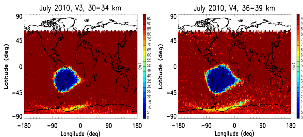
Figure 7. Spatial distribution of the calibration success rates for V3 and V4 for the month of July 2010. The data are binned in 2^\circ \times 2^\circ in latitude and longitude.
