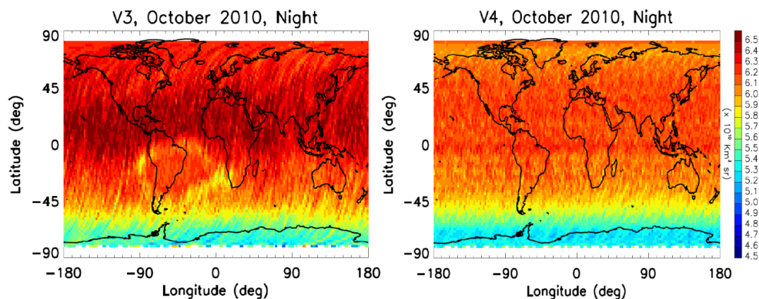
Figure 9. Spatial distribution of the 532 nm nighttime calibration coefficient ( \text{km}^3 \text{sr} ) for October 2010, (left) from V3 and (right) from V4.
