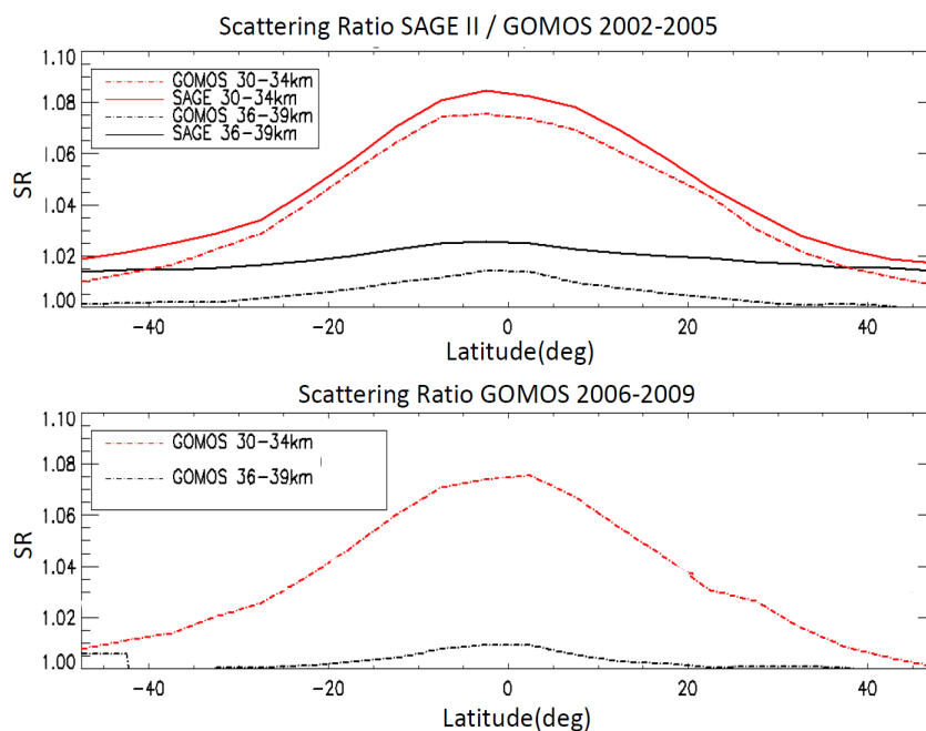
Figure 2. Scattering ratio at 30-34 km and 36-39 km at 532 nm (top) from SAGE II and GOMOS for the years 2002-2005 and (bottom) from GOMOS for the years 2006-2009.
