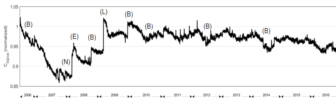
20 Figure 8. Time series of the granule-averaged V4 532 nm CALIOP nighttime parallel channel calibration coefficient, smoothed over 10 consecutive granules. The values have been normalized by the initial value ( 6.1483 \times 10^{10} \text{ km}^3 \text{ sr} ). Letters indicate a subset of most significant instrument events
