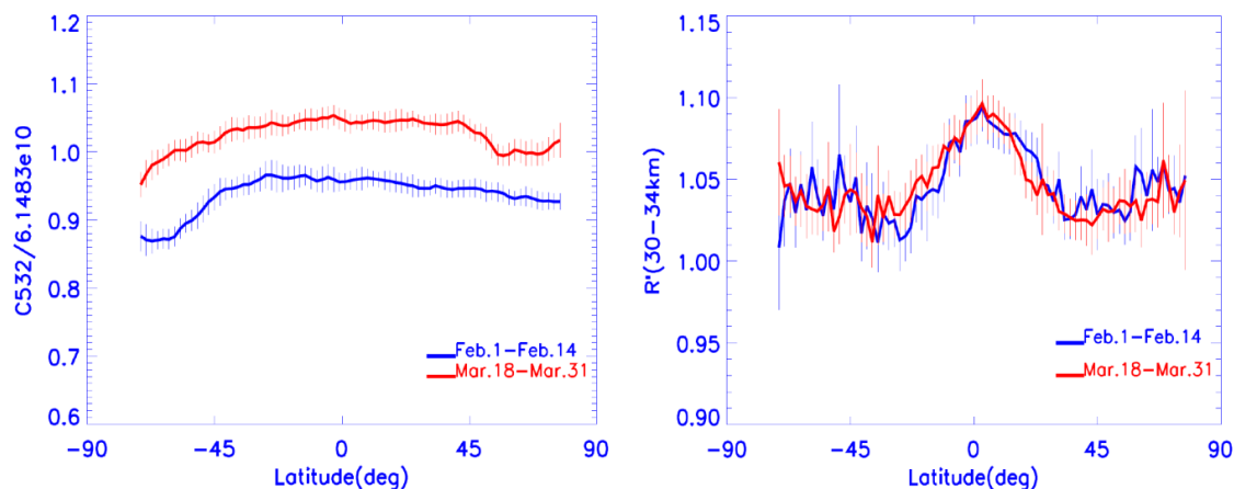
Figure 13. (left) Means and standard deviations of the zonally averaged 532 nm calibration coefficients normalized with respect to the initial value in Figure 8, (i.e., 6.1483 \times 10^{10} \text{ km}^3 \text{ sr} ), and (right) mean and standard deviation of R' averaged over 30-34 km. Both time series were calculated using 2 weeks' worth of data before (February 1-14, 2009) and after (March 18-31, 2009) the laser switch. R' profiles were calculated over 2^\circ latitude intervals from each granule and then averaged over all granules for the latitude bin, with a minimum number of 50 R' profiles required in each bin. Data over the SAA were not included.
