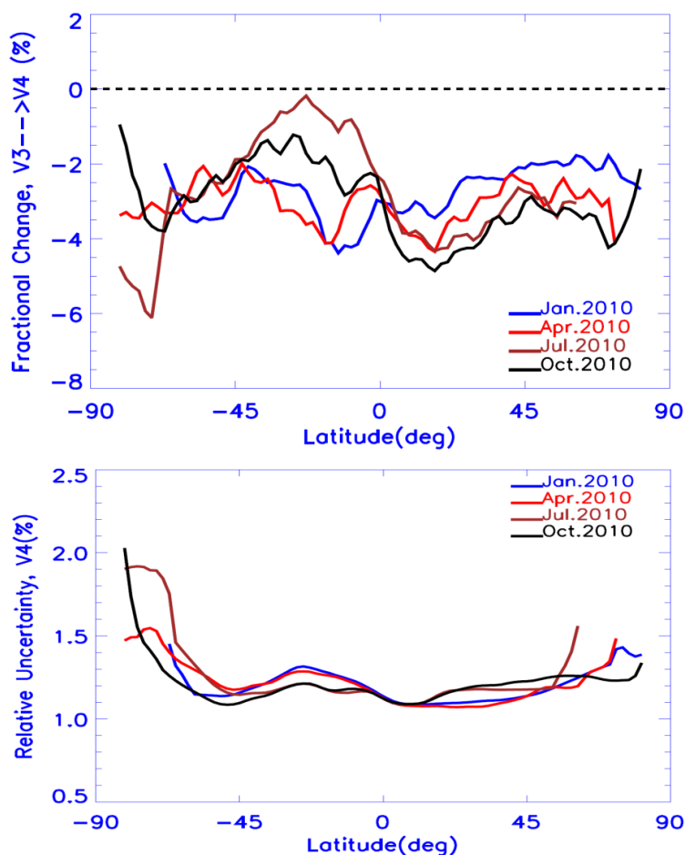
5 Figure 10. The fractional change from V3 to V4, (V4-V3)/V3 in the zonally averaged 532 nm calibration coefficient for 4 months in 2010 (top panel) and the zonally averaged relative uncertainty ( \Delta C_{532}/C_{532} ) in the V4 calibration coefficient for the same months (bottom panel).
