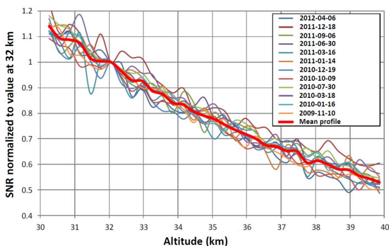
Figure 3. 12 SNR profiles from CALIOP measurements representing various latitudes and seasons.
