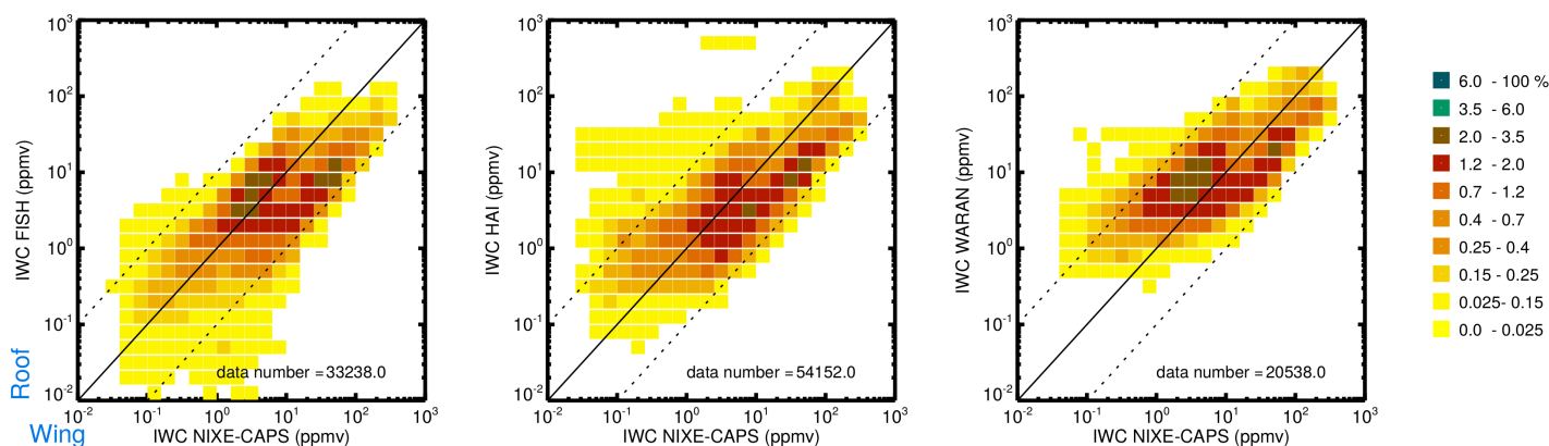
Figure 8. Comparison of IWCs from roof-mounted closed-path hygrometers FISH, HAI and Waran (see Equation 1, H_2O_{gas} from SHARC) and wing-mounted cloud spectrometer NIXE @HALO during ML-CIRRUS 2014 (color code: frequencies; solid black: 1:1 line; dashed: \pm factor 10 to 1:1 line).
