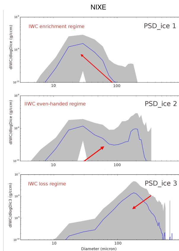
Figure 11. Three types of cirrus mass size distributions dIWC/d\log D_{ice} , exemplarily for the flight on 4 April 2014. Blue lines represent the mean PSDs, the grey area the standard deviation; note that for the portrayal of the PSD we use the ice particle diameter and not radius to clearly distinguish from the mean mass radius R_{ice} of the ice particle population used in Figures 10.
