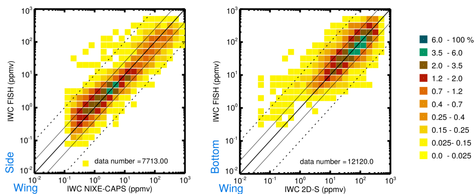
Figure 9. Comparison of IWCs from left: side mounted closed-path FISH (see Equation 1, H_2O_{gas} from FLASH) and wing-mounted cloud spectrometer NIXE @Geophysica during StratoClim 2017; right: bottom-mounted closed-path FISH (see Equation 1, H_2O_{gas} from HWV) and wing-mounted cloud spectrometer 2D-S @WB-57 during MacPex 2011 (color code: frequencies; solid black: 1:1 line; dashed/thin: \pm factor 10/2.5 to 1:1 line).
