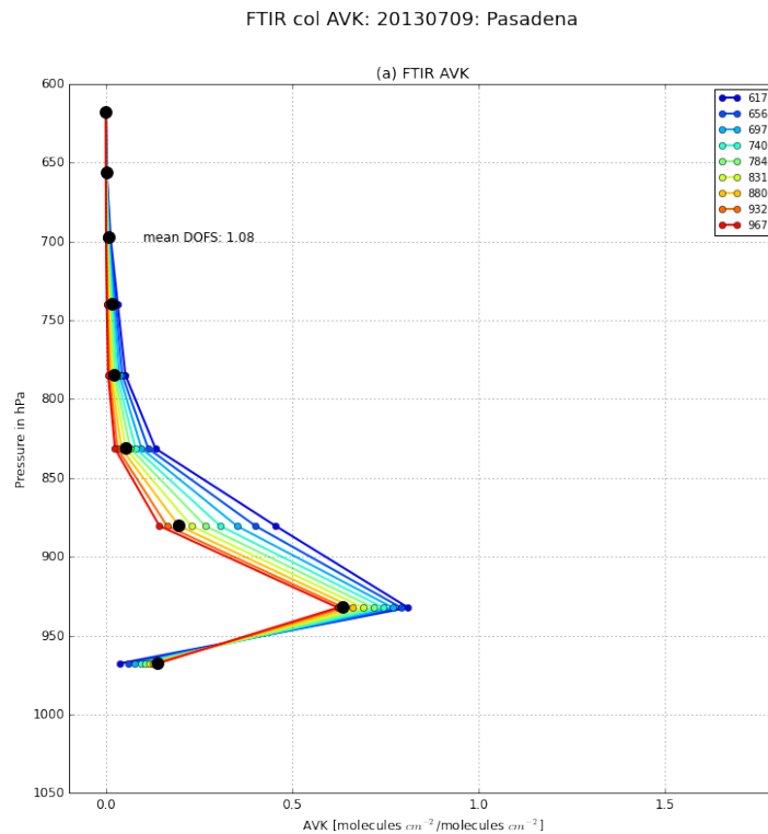
Fig. 1. FTIR averaging kernel in [molecules \text{cm}^{-2} / molecules \text{cm}^{-2} ]. The black dots show the matrices diagonal values.
