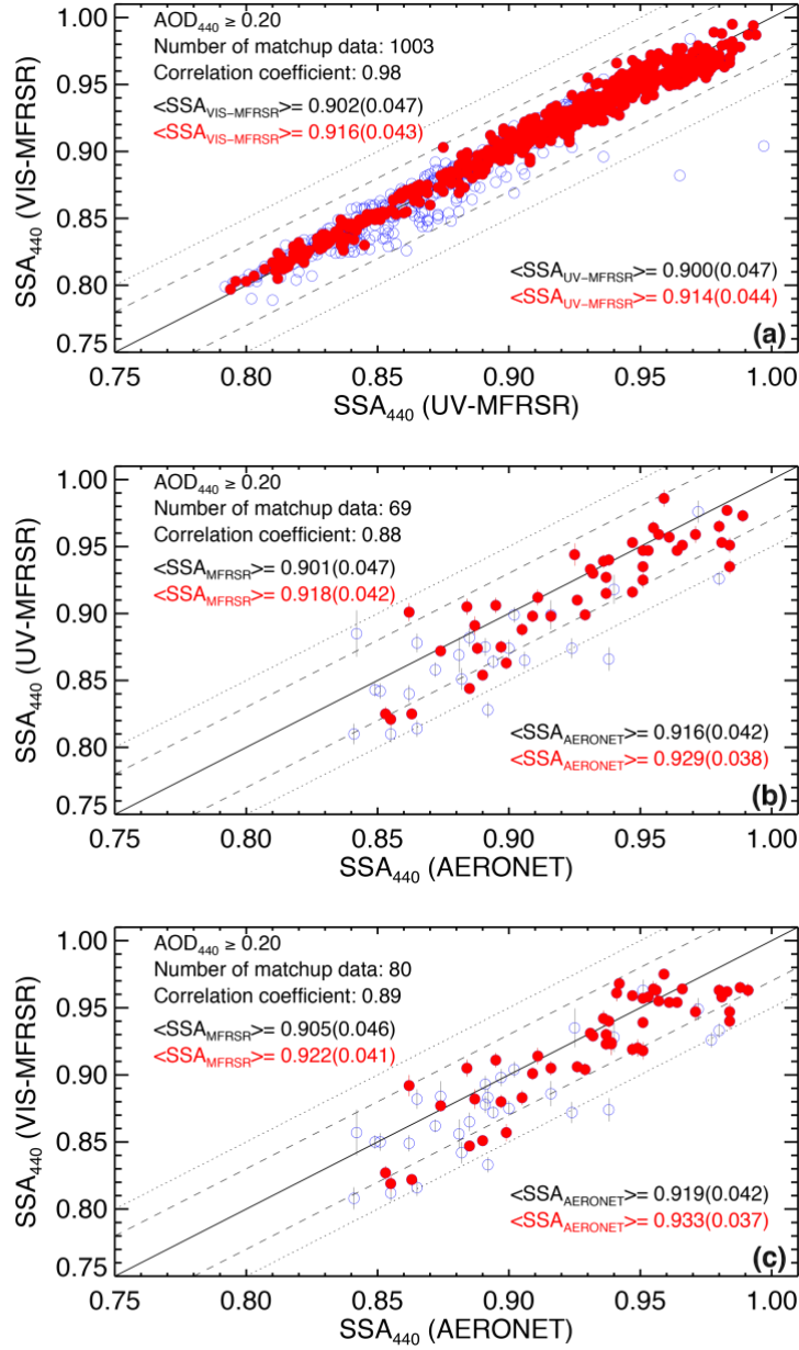
Figure 3. Comparison between SSA at 440 nm retrieved from AERONET-only and AMP retrievals in Seoul: (a) all 1-minute UV-MFRSR versus VIS-MFRSR retrievals, (b) AERONET inversions versus 32-minute average UV-MFRSR retrievals, and (c) AERONET inversions versus 32-minute average VIS-MFRSR retrievals. MFRSR SSA mean errors are shown assuming 3% error in diffuse to direct ratio. The UV- and VIS-MFRSR SSA in (b) and (c) are averaged within \pm 16 minutes from the AERONET retrieval time. The dashed lines show SSA agreement within \pm 0.03 , which is assumed SSA error. The dotted lines are \pm 0.05 of the 1:1 line. Red color shows comparisons for \text{AOD}_{440} \geq 0.4 , consistent with the best quality Level 2 AERONET inversions. Blue dots indicate retrievals for 0.2 \leq \text{AOD} < 0.4 . Combined SSA statistics for \text{AOD} \geq 0.2 are shown in black. Standard deviation of SSA is indicated in parentheses.
