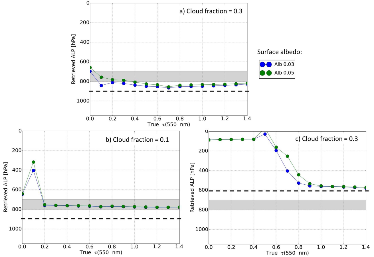
Figure 14. Same as Fig. 10 but with one unique aerosol \omega_0 value ( = 0.9 ) and the inclusion of a cloud (dashed thick black line) in addition to the aerosol layer. The cloud reflectance is simulated via a simple opaque (cloud albedo = 0.8) and Lambertian layer: (a) Effective cloud fraction = 0.3 and cloud pressure = 900 hPa, (b) Effective cloud fraction = 0.1 and cloud pressure = 900 hPa, (c) Effective cloud fraction = 0.3 and cloud pressure = 600 hPa.
