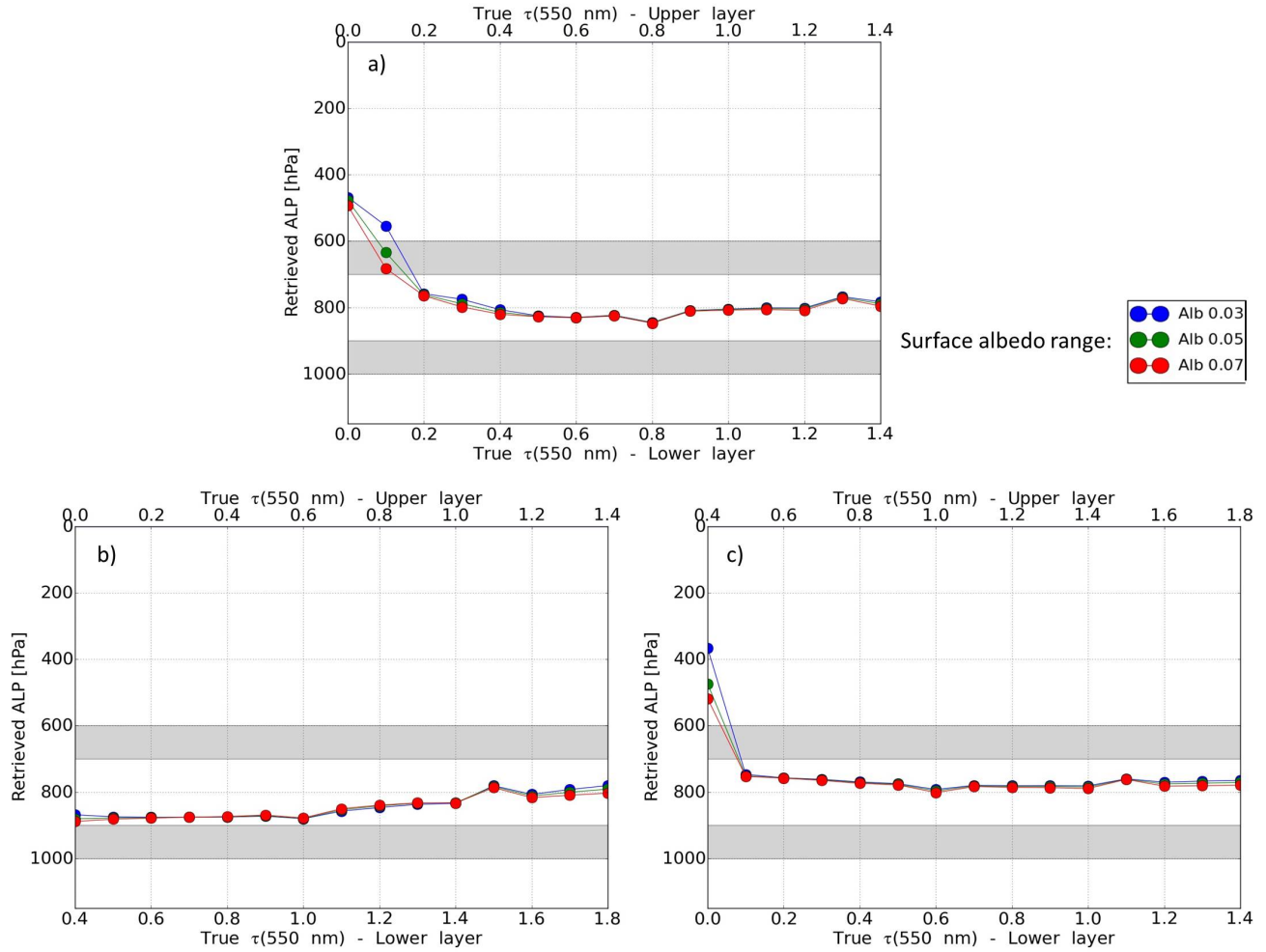
Figure 12. Same as Fig. 10 but with one unique aerosol \omega_0 value ( = 0.9 ) and 2 separate aerosol layers included in the simulated spectra. The bottom x-axis corresponds to the \tau(550 \text{ nm}) value of the lower layer, while the top x-axis is the \tau(550 \text{ nm}) value of the upper layer. Both layers have same geometric thickness (i.e. 100 hPa). The first is located between 600 and 700 hPa, and the second is between 900 and 1000 hPa. (a) Both aerosol layers have same optical properties and \tau(550 \text{ nm}) values, (b) Both aerosol layers have same optical properties but different \tau(550 \text{ nm}) values: the lower layer has systematically a higher \tau(550 \text{ nm}) (i.e. +0.4 for each scenario), (c) Both aerosol layers have same optical properties but different \tau(550 \text{ nm}) values: the upper layer has systematically a higher \tau(550 \text{ nm}) (i.e. +0.4 for each scenario)
