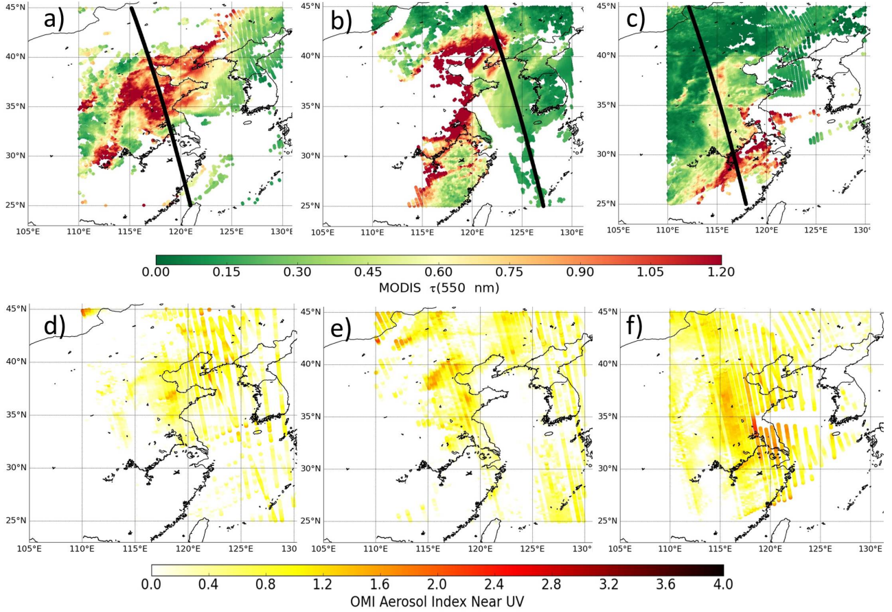
Figure 1. Maps of MODIS Aqua \tau(550\text{nm}) from the combined DT and DB Collection 6 (cf. Sect. 2.3), and collocated OMI aerosol index from near UV (UVAI) values (cf. Sect. 3) over cloud-free scenes for the urban and industrialized cases in east China. The dark thick lines represent the track of CALIPSO space-borne sensor over the selected case studies: (a d) 2006.10.02, (b e) 2006.10.06, (c f) 2006.11.01.
