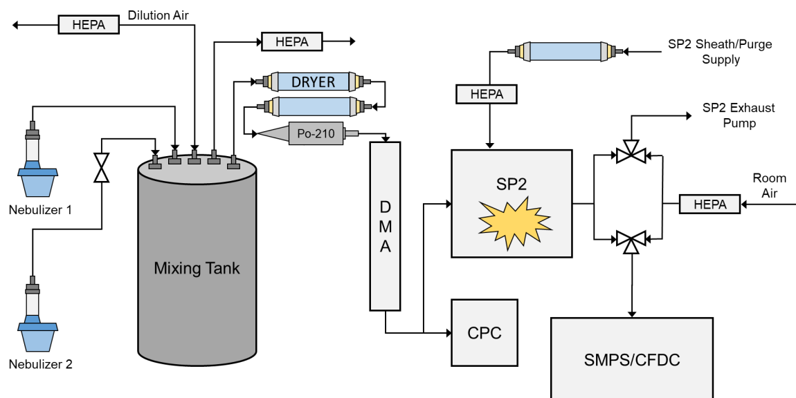
Figure 1. The experimental setup for unmixing, internal mixing, and external mixing studies with the SP2-SMPS/CFDC.
