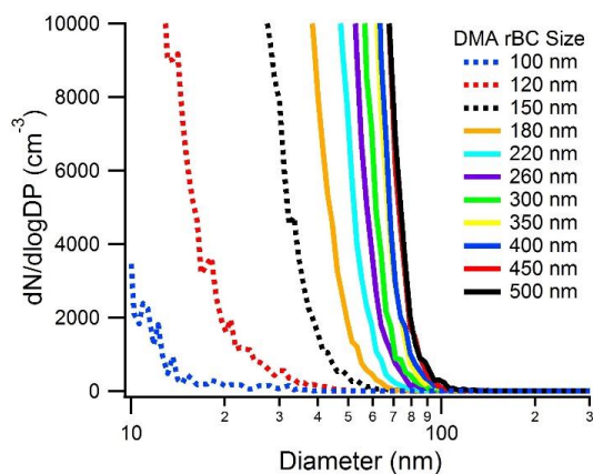
Figure 4: Size distribution of SP2 exhaust from different sized-selected rBC particles. The concentration of size-selected rBC particles was approximately 1000 \text{ cm}^{-3} .
