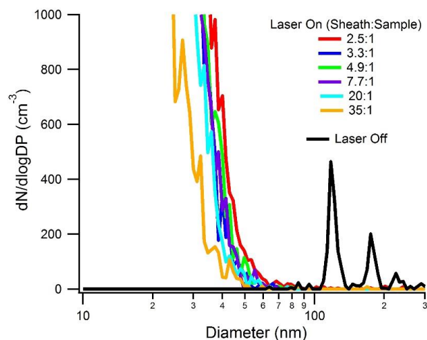
Figure 3: Size distribution of the SP2 exhaust from a 125-nm Aquadag® particle under different sheath-to-sample ratios. For reference, the size distribution of a 125-nm Aquadag particle at a sheath-to-sample ratio of 4.9:1 is shown in black
