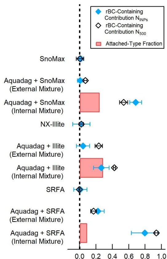
Figure 8. The rBC-containing contribution of INPs ( N_{INPs} ) active at -30\text{ }^{\circ}\text{C} and 105% RH, particles greater than 500 nm ( N_{500} ), and the number fraction of attached-type particles for the internally-mixed scenarios. As shown, the attached-type fraction correlates poorly with rBC contributions to N_{INPs} .
