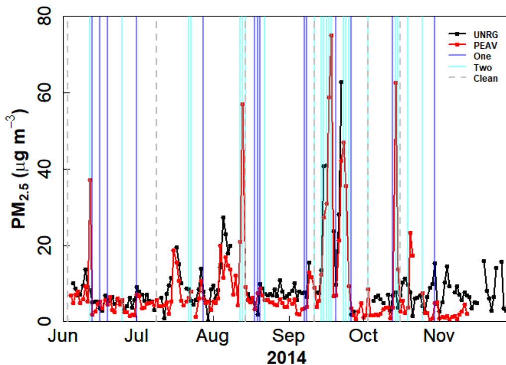
Figure 2: PM 2.5 ( \mu\text{g m}^{-3} ) at PEAV (red) and UNRG (black) for June to November 2014. Vertical dark blue lines are days with aggregates on one inlet, vertical light blue lines are days with aggregates on two inlets, dashed grey lines are days when the inlets were cleaned.
