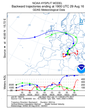
Figure 3: In panel a , it is shown the comparison between RCS profiles obtained from MUSA and MiniMPL on 29 August 2016 from 19:16 to 20:47 UT; In panel b , the corresponding air mass back trajectory analysis performed using NOAA HYSPLIT model is reported; HYSPLIT simulations have been initialized at the three levels from the ground to the top height of the highest layer observed by both MUSA and MiniMPL lidars.
