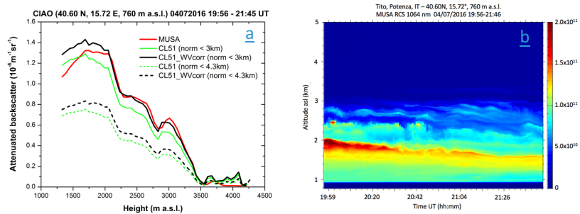
Figure 9: Panel a, comparison between the attenuated backscatter vertical profiles retrieved from MUSA and CL51 on 4 July 2016 from 19:56 to 21:45 UT and obtained using two different normalization ranges, the first below 3 km (solid lines) and the second below 4.3 km (dashed lines); both the raw calibrated profiles and the water vapor calibrated corrected profiles are shown; panel b, time series of the RCS measured with MUSA at 1064 nm during the same time period used to create the average profiles in the panel a.
