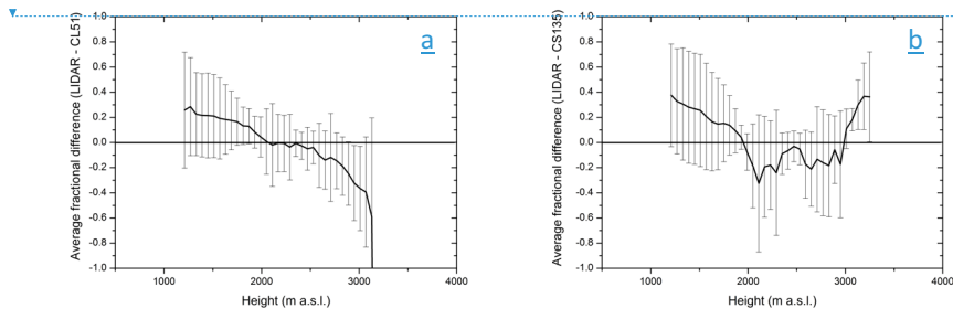
1195 Figure 11: Panel a , profiles of the average fractional difference between CIAO LIDARs and CL51 values of the attenuated backscatter calculated for 19 cases of simultaneous and collocated measurements; panel b , same as panel a but for CIAO LIDARs and CS135 calculated for 9 cases. The vertical bars are the standard deviations of fractional differences.
