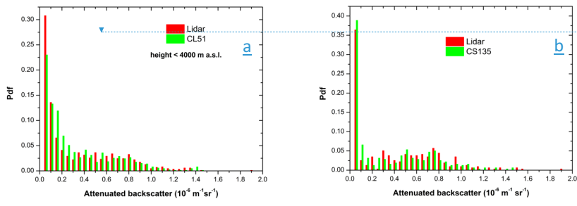
1245 Figure 12: Pdfs of the attenuated backscatter values measured or estimated by CIAO LIDARs and CL51 (panel a) and by CIAO LIDARs and CS135 (panel b) below 4 km, respectively.
