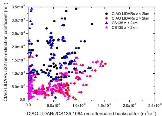
Figure 13: Comparison of the scatterplots showing the 532 nm CIAO LIDAR aerosol extinction coefficient vs 1064 nm attenuated backscatter from CIAO LIDARs and CL51 (panel a), and from CIAO LIDARs and CS135 (panel b). Black dots are the values of CIAO LIDARs measured below 2 km, red dots are the values of CIAO LIDARs measured above 2 km, blue triangles are the values of CL51/CS135 measured below 2 km, and pink triangles are the values of CL51/CS135 measured above 2 km.
