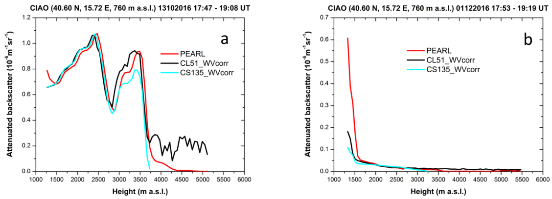
845 Figure 8: Panel a , comparison between the attenuated backscatter profiles retrieved from PEARL, CL51 and CS135 on 13 October 2016 in the time interval from 17:47 to 19:08 UT and obtained normalizing the ceilometer profiles on the PEARL profile in the region between 1.8 and 3.0 km; panel b , same as panel a , but for the 01 December 2016 in the time interval from 17:53 to 19:19 UT. All the ceilometer profiles are corrected for the water vapor absorption affecting the signal extinction at 910-912 nm.
