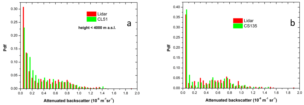
980 Figure 12: Pdfs of the attenuated backscatter values measured or estimated by CIAO LIDARs and CL51 (panel a ) and by CIAO LIDARs 985 and CS135 (panel b ) below 4 km, respectively.
