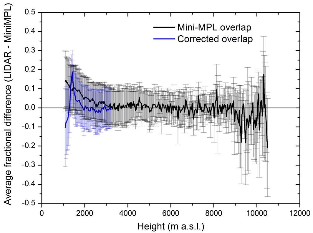
740 Figure 5: Profiles of the average fractional difference between MUSA and MiniMPL values of RCS calculated on 12 cases of simultaneous and collocated measurements (black line). Blue line is the same as black line but applying an additional overlap 745 correction factor to the MiniMPL data processing estimated using the ratio between MUSA and MiniMPL profiles during the cleanest simultaneous measurement session available during INTERACT-II. The vertical bars are the standard deviations of fractional difference.
