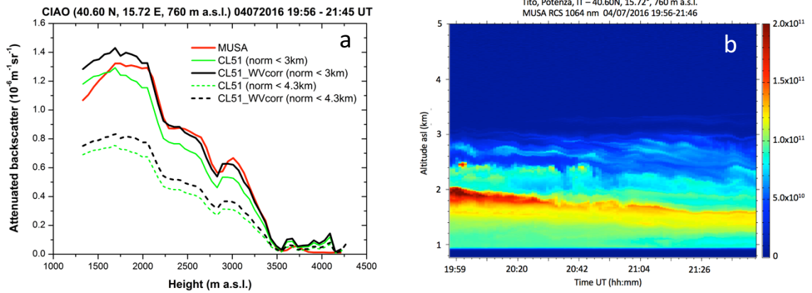
880 Figure 9: Panel a , comparison between the attenuated backscatter vertical profiles retrieved from MUSA and CL51 on 4 July 2016 from 19:56 to 21:45 UT and obtained using two different normalization ranges, the first below 3 km (solid lines) and the second below 4.3 km (dashed lines); both the raw calibrated profiles and the water vapor calibrated corrected profiles are shown; panel b , time series of the RCS measured with MUSA at 1064 nm during the same time period used to create the average profiles in the panel a .
