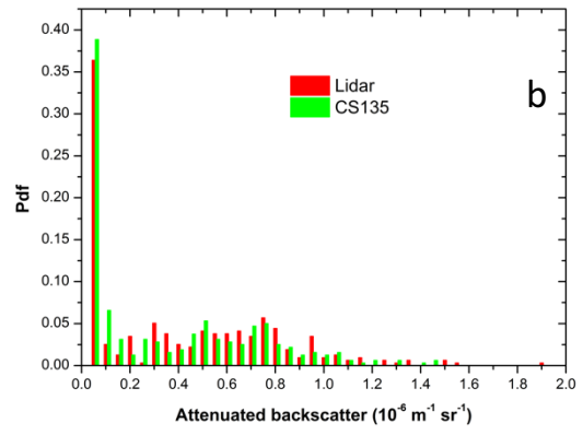
Figure 12: Pdfs of the attenuated backscatter values measured or estimated by CIAO LIDARs and CL51 (panel a ) and by CIAO LIDARs and CS135 (panel b ) below 4 km, respectively.
