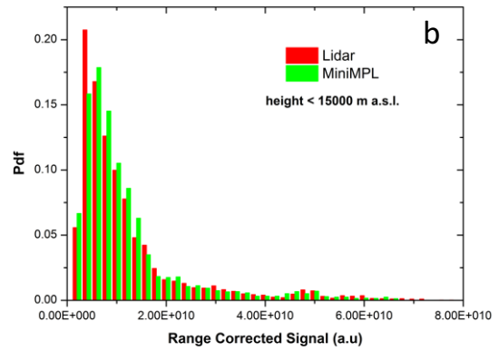
Figure 6: Panel a , pdfs of the RCS values measured by CIAO LIDARs and MiniMPL below 4 km; panel b , same as panel a but for the entire vertical range of observed lidar profiles, below 15 km .
