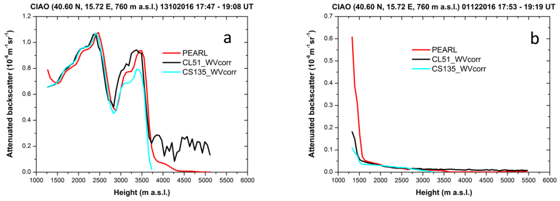
Figure 8: Panel a , comparison between the attenuated backscatter profiles retrieved from PEARL, CL51 and CS135 on 13 October 2016 in the time interval from 17:47 to 19:08 UT and obtained normalizing the ceilometer profiles on the PEARL profile in the region between 1.8 and 3.0 km; panel b , same as panel a , but for the 01 December 2016 in the time interval from 17:53 to 19:19 UT. All the ceilometer profiles are corrected for the water vapor absorption affecting the signal extinction at 910-912 nm.
