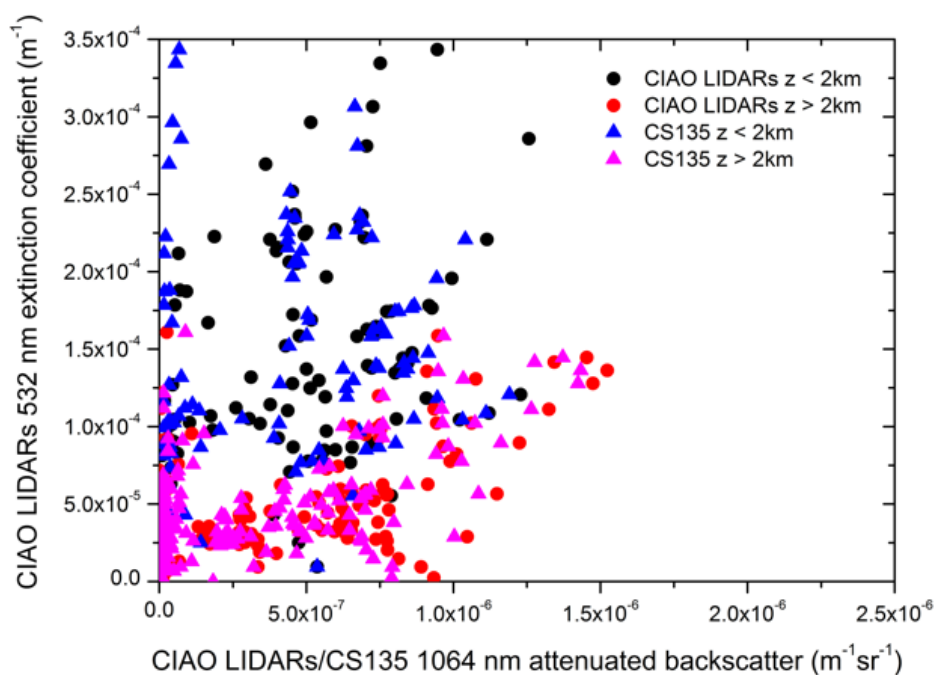
1040 Figure 13: Comparison of the scatterplots showing the 532 nm CIAO LIDAR aerosol extinction coefficient vs 1064 nm attenuated backscatter from CIAO LIDARs and CL51 (panel a ), and from CIAO LIDARs and CS135 (panel b ). Black dots are the values of CIAO LIDARs measured below 2 km, red dots are the values of CIAO LIDARs measured above 2 km, blue triangles are the values of CL51/CS135 measured below 2 km, and pink triangles are the values of CL51/CS135 measured above 2 km.
