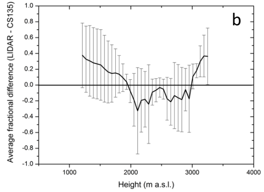
Figure 11: Panel a , profiles of the average fractional difference between CIAO LIDARs and CL51 values of the attenuated backscatter calculated for 19 cases of simultaneous and collocated measurements; panel b , same as panel a but for CIAO LIDARs and CS135 calculated for 9 cases. The vertical bars are the standard deviations of fractional differences.
