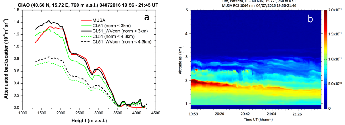
870 Figure 9: Panel a , comparison between the attenuated backscatter vertical profiles retrieved from MUSA and CL51 on 4 July 2016 from 19:56 to 21:45 UT and obtained using two different normalization ranges, the first below 3 km (solid lines) and the second below 4.3 km (dashed lines); both the raw calibrated profiles and the water vapor calibrated corrected profiles are shown; panel b , time series of the RCS measured with MUSA at 1064 nm during the same time period used to create the average profiles in the panel a .
