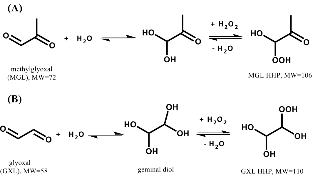
Figure 3. ROOH formation from reactions of H 2 O 2 with (A) methylglyoxal, and (B) glyoxal.
