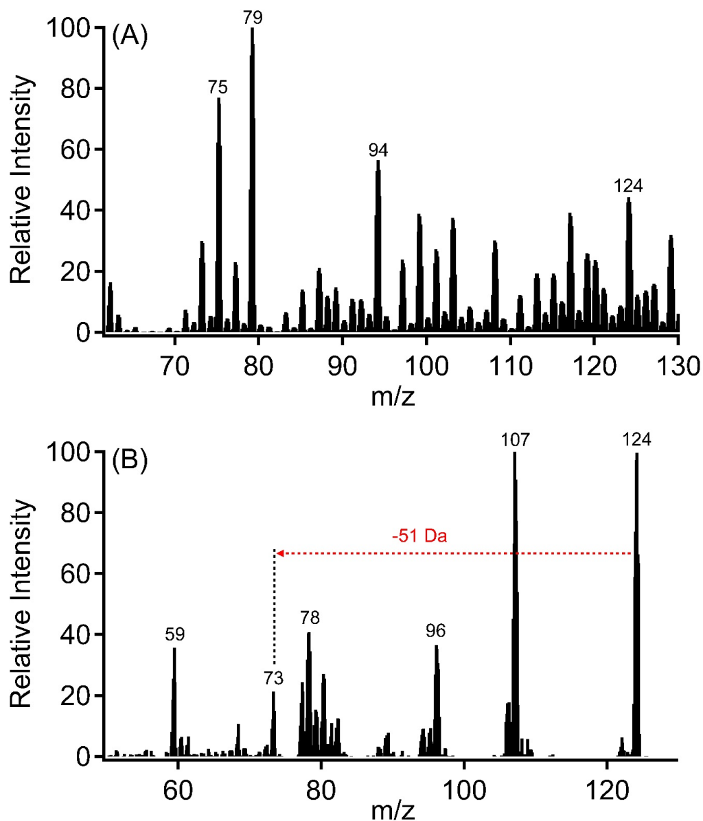
Figure 4. (A) Mass spectrum of reaction of methylglyoxal with H 2 O 2 in the presence of AA; (B) Product mass spectrum of m/z 124 from (A).
