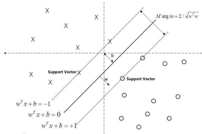
Figure 5: The decision boundary of support vector machine with the largest margin. \times and \circ denote two-class training examples, respectively. w^T x + b = 0 is the optimal hyperplane to do the separation, where w is a weight vector and b is a bias, and an SVM training model with the largest margin 2/\sqrt{w^T w} is built. The support vectors are the samples on the dotted lines. The optimization classification hyperplane is determined by the solid line.
