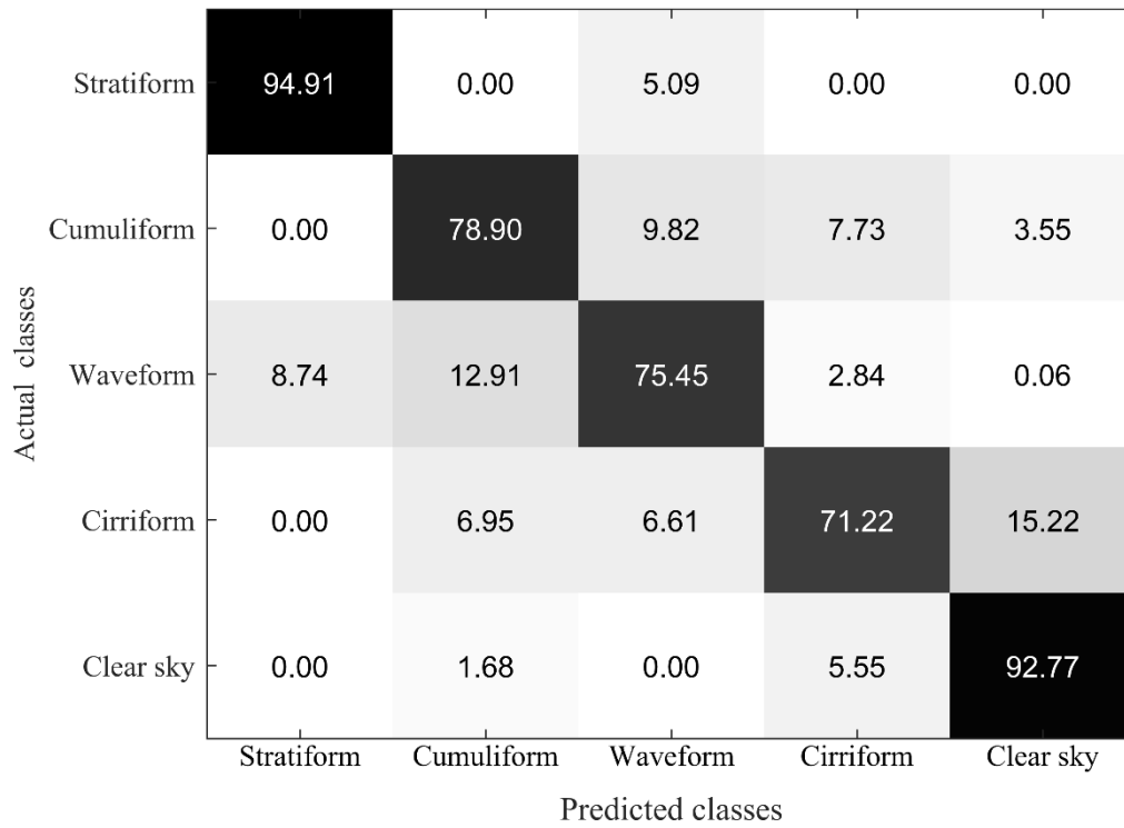
Figure 7: Confusion matrix (%) on the whole-sky dataset. (1/2 for training and the overall accuracy is 83.54%)
