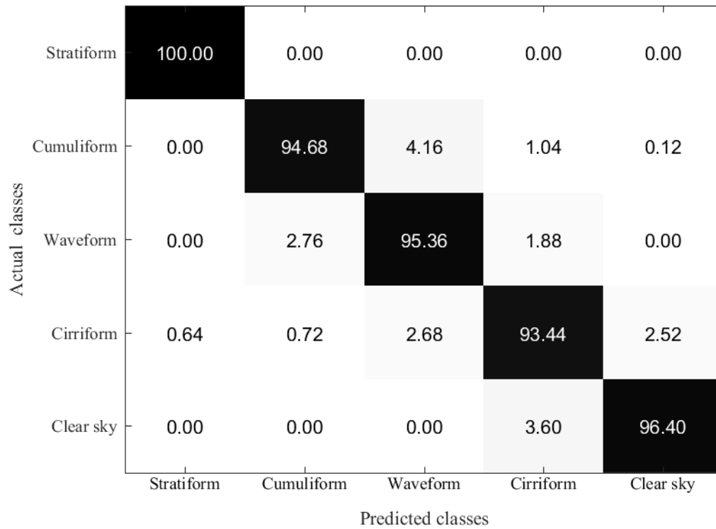
Figure 6: Confusion matrix (%) on the zenithal dataset. (1/2 for training and the overall accuracy is 95.98%)
