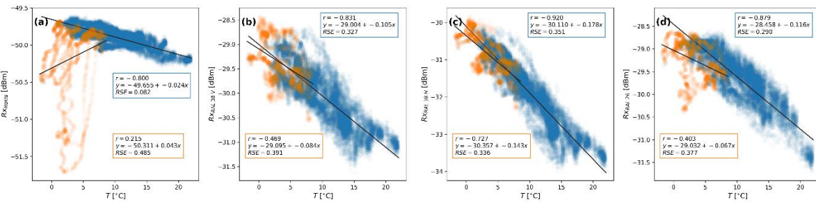
15 Figure 11: Scatterplots of link received power versus ambient air temperature measured at the “Veenkampen” meteorological station. Blue dots indicate times when relative humidity (as measured at “Veenkampen”) is < 90%; orange dots indicate times when relative humidity > 90%. Solid lines indicate linear least-squares regression fit. Links: (a) Nokia Flexihopper, (b) RAL 38 GHz vertical, (c) RAL 38 GHz horizontal, (d) RAL 26GHz.
