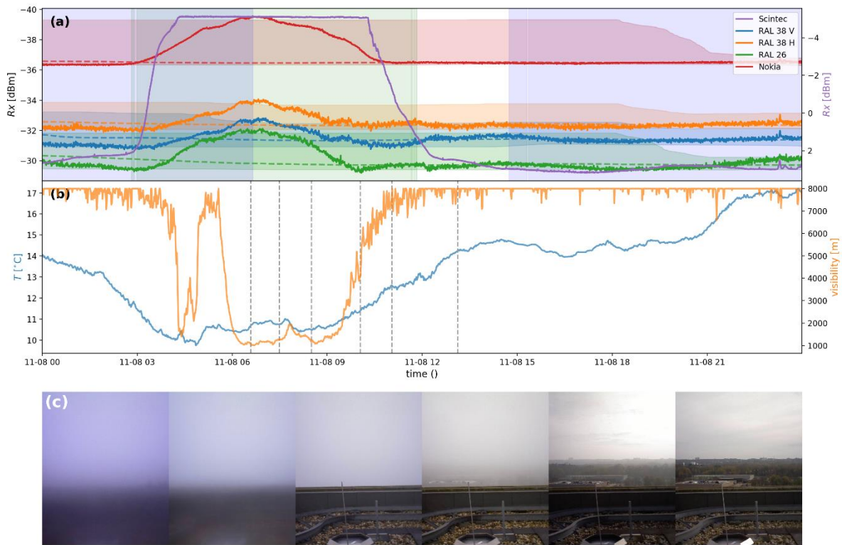
5 Figure 12: Time series of an event on 8 November 2015. (a): Received power levels at the detectors (solid lines) and reference levels (median over dry periods in a 24-hour moving window) (dashed lines). Periods with a negative net radiation flux at the surface are indicated with blue shading. Periods with a relative humidity >90% are indicated with green shading. (b): Several atmospheric variables measured at the “Veenkampen” meteorological station: visibility and ambient air temperature at 2 m indicated with orange and blue lines, respectively. (c): Images from the time-lapse camera at the location of the receiving antennas aimed along the link path. The times at which these images were captured are indicated by the vertical dotted lines.
