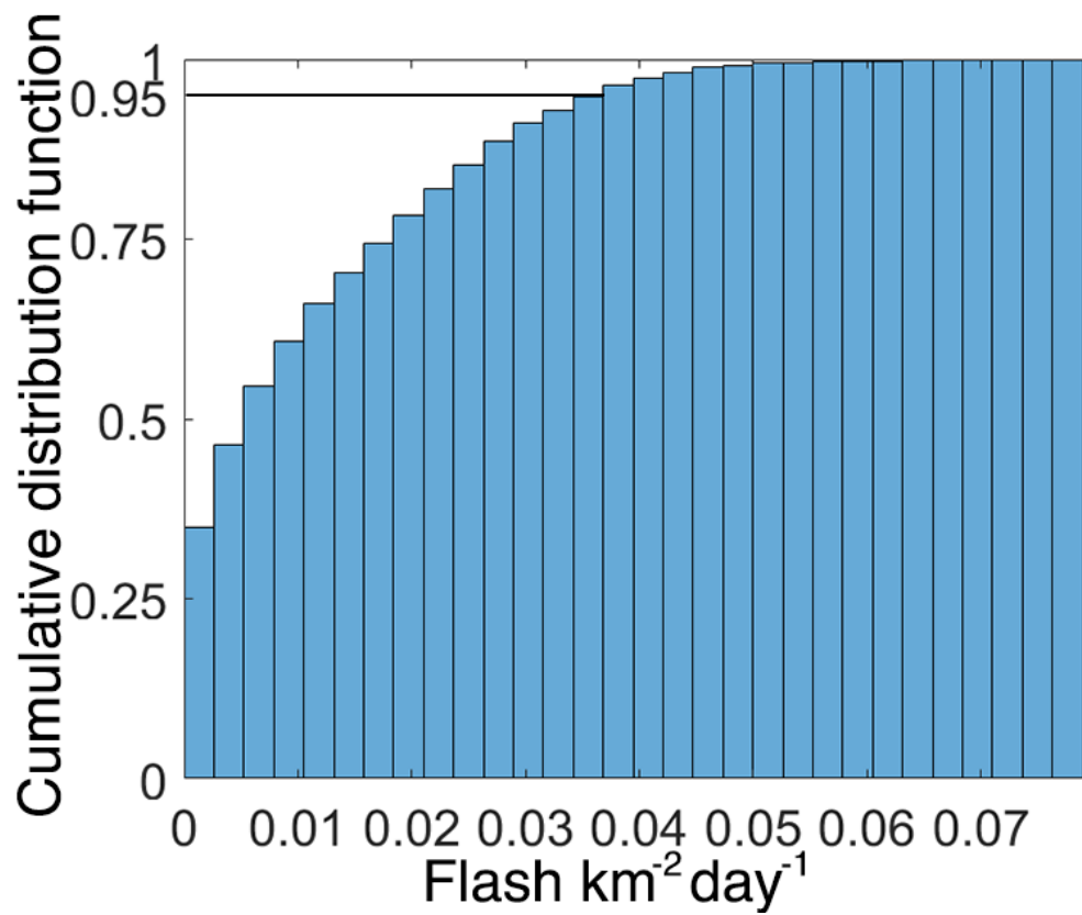
Figure S2. The cumulative distribution function of NLDN detected CG lightning density in the South.
