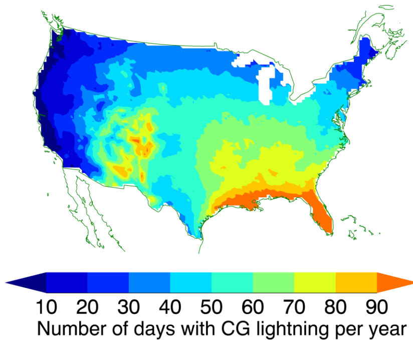
Figure 3. Number of days with NLDN detected CG lightning per year during 2005-2014. The lightning occurrences are calculated using the REAM grid resolution.
