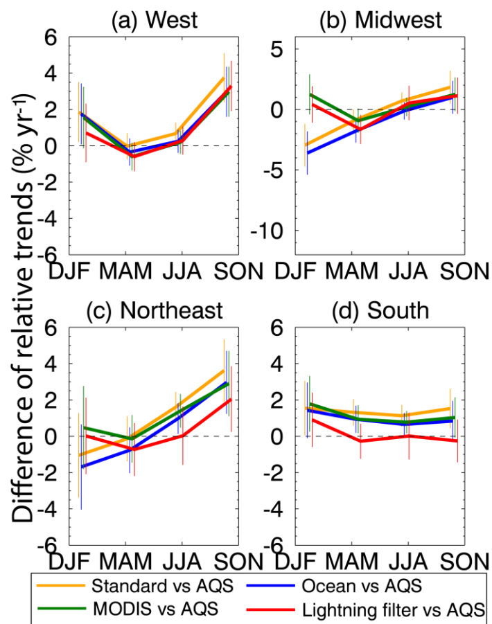
Figure 7. Seasonal differences of OMI-based relative trends from those computed from AQS in situ data. The relative trends are shown in Figs. 6 and 8. The figure legends are the same as in Figs. 6 and 8 but with the AQS trends subtracted from the OMI-based trends.
