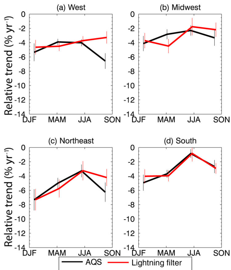
Figure 6. Same as Figure 5 but for coincident AQS (black line) and OMI data (red line) after applying the lightning filter. The coincident data points are less than used in Figure 5 and therefore the AQS trends are not the same.
