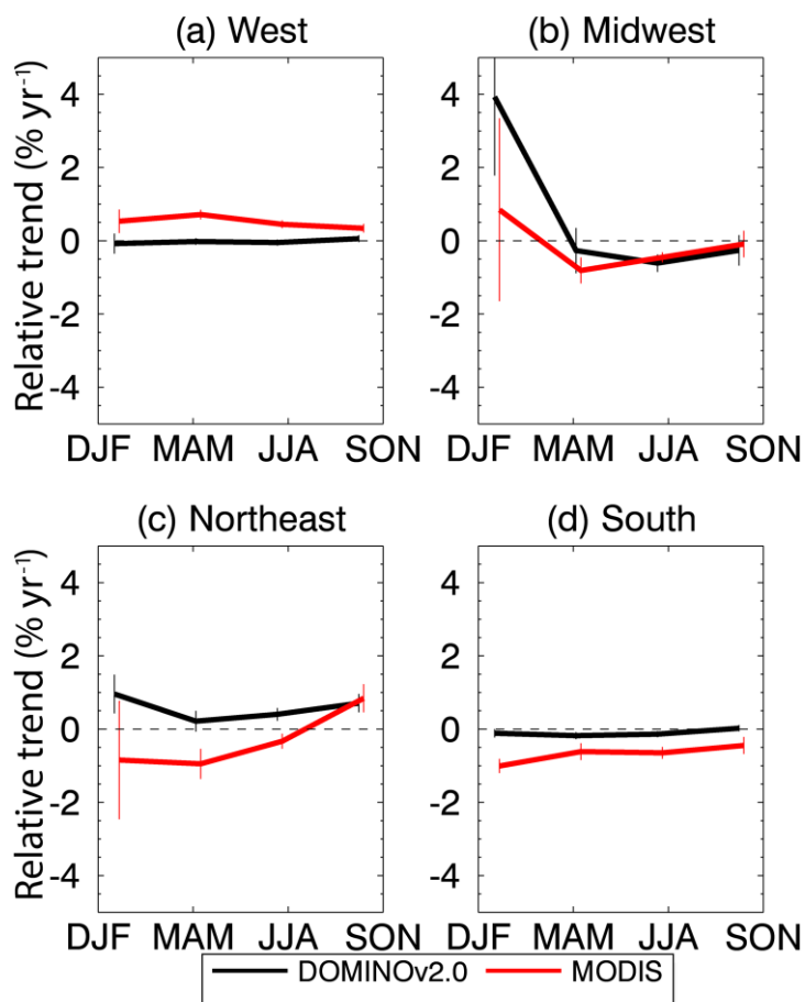
Figure 5. Seasonal relative albedo trends of OMI (black line) and MODIS (red line) surface reflectance products, coincident with AQS in situ data used in Figure 5. The error bars represent 95% confidence intervals.
