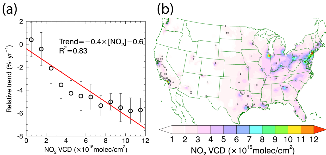
Figure 9. (a) “Lightning filter” OMI-based NO 2 relative trend as a function 2005-2014 averaged OMI tropospheric NO 2 VCD binned every 1 \times 10^{15} \text{ molec/cm}^2 . Red line shows a least-squares regression. (b) The distribution of 2005-2014 averaged OMI tropospheric NO 2 VCD. Black bordered circles represent AQS sites. The corrected OMI tropospheric NO 2 data are used.
