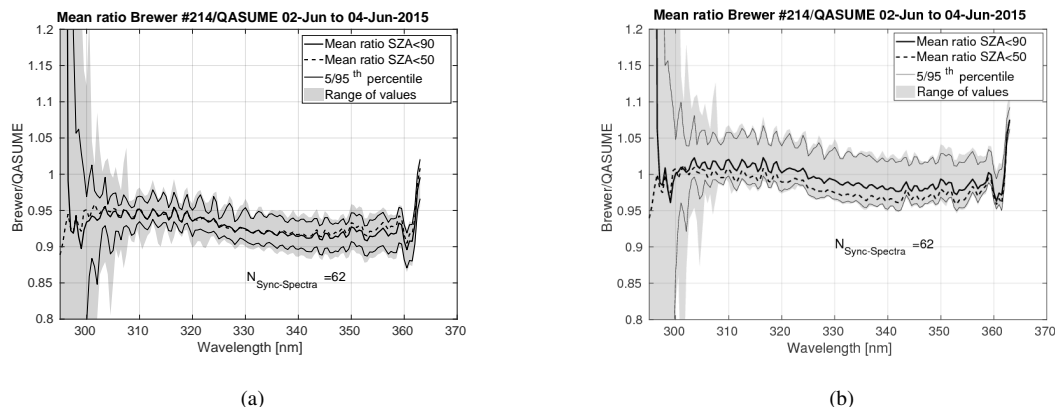
Figure 6. Mean ratio and range of measurements between Brewer #214 and QASUME irradiances for measurements done at SZA < 90° and SZA < 50° in the comparison campaign in Huelva during 2nd–4th June 2015. The 5th and 95th percentile and the range of the values, and the number of QASUME synchronized spectra ( N_{\text{Sync-Spectra}} ) are shown. a) No cosine error correction was applied to the data. b) The data was cosine error corrected.
