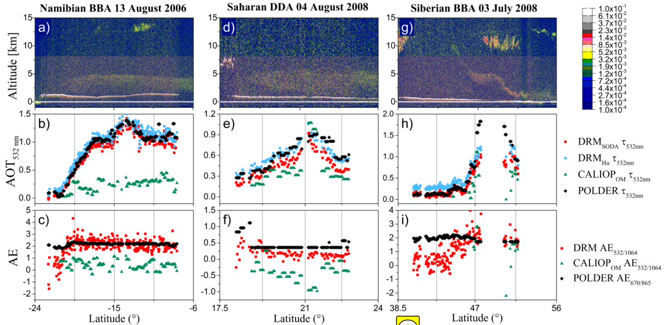
Figure 1: The first row of the panel shows the lidar CALIOP backscatter profile at 532 nm ( \text{km}^{-1} \text{sr}^{-1} ) for three case studies: African biomass-burning (BBA) aerosols above clouds on 13 August 2006 ((a), (b), (c)), Saharan dust (DDA) on 4 August 2008 ((d), (e), (f)) and Siberian biomass-burning aerosols over the Okhotsk Sea on 3 July 2008 ((g), (h), (i)). For these cases, the above-cloud AOT at 532 nm and the Ångström exponent (AE) as a function of latitude, measured with several techniques are displayed.
