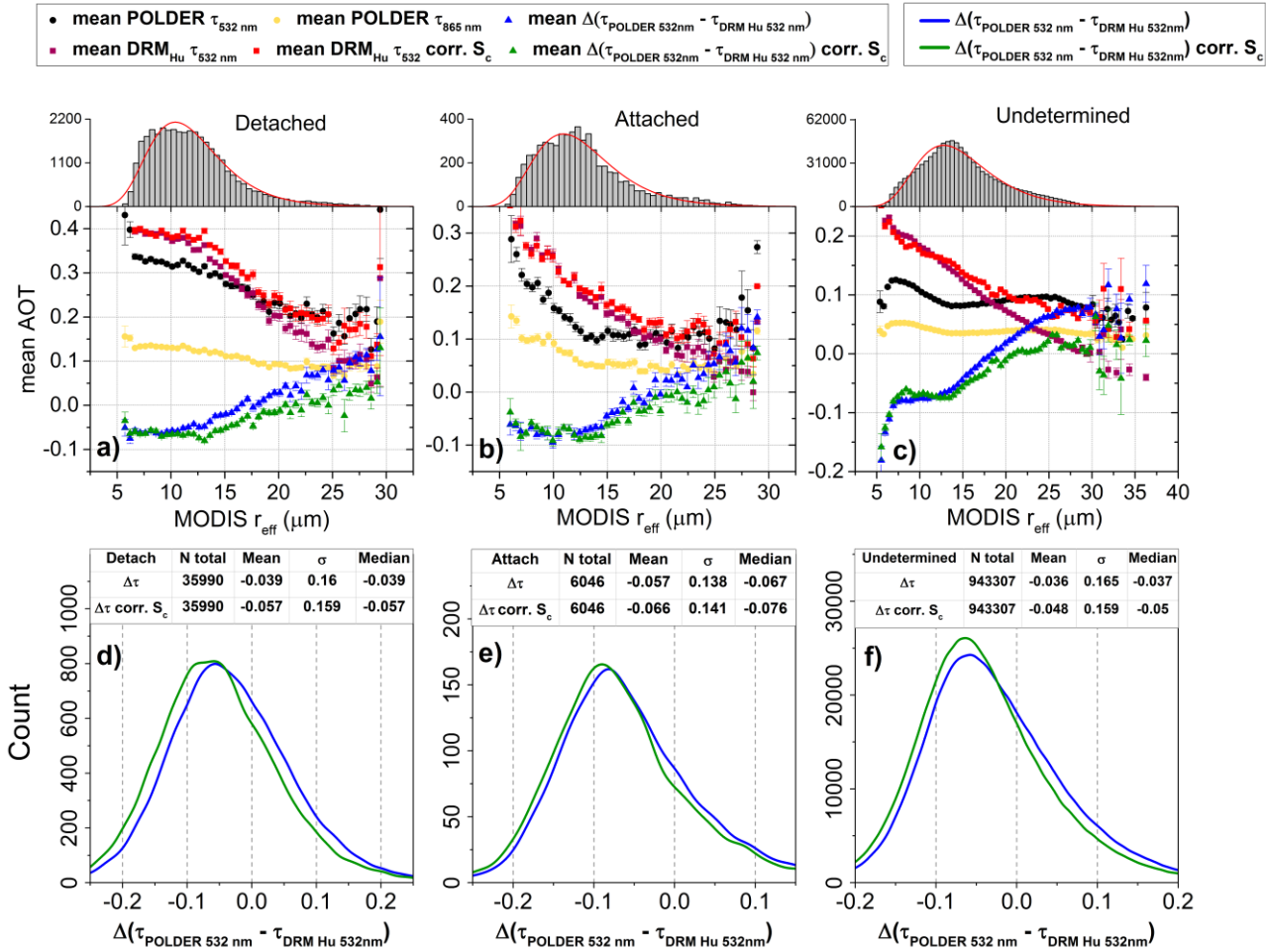
Figure 6: Same as Fig. 5, POLDER and DRM Hu above cloud AOT retrievals as a function of MODIS effective radius ( r_{\text{eff}} , \mu\text{m} ).
