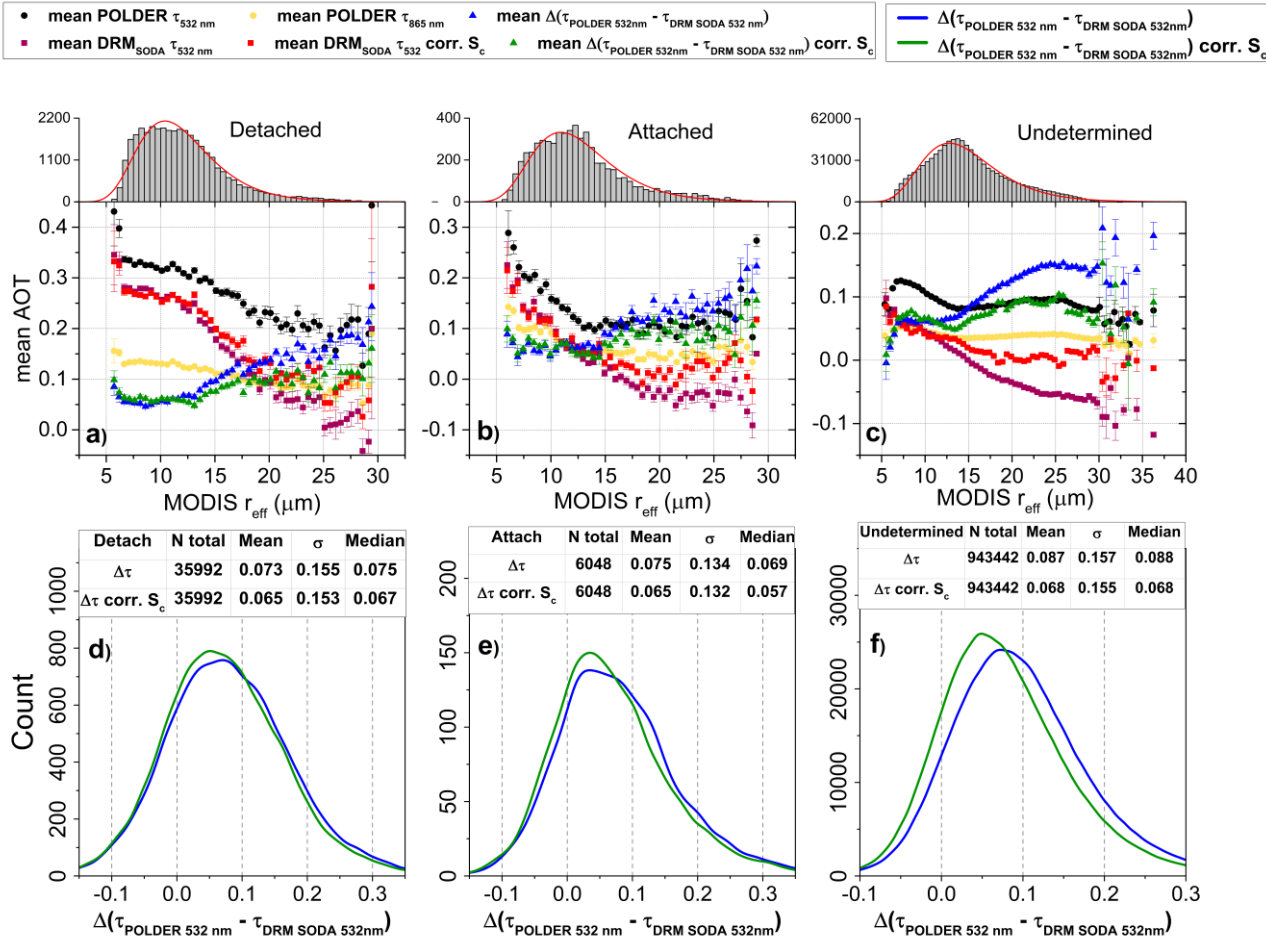
Figure 5: 4.5 years of global study on the evolution of POLDER and DRMSODA above cloud AOT retrievals as a function of MODIS effective radius ( r_{eff} , \mu\text{m} ) for situations where: the aerosol layer is detached from the cloud top ((a) and (d)), for cases where the aerosol layer is attached to the cloud top ((b) and (e)) and for undetermined situations (c) and (f)). The histograms from figures (a), (b) and (c) represent the distribution of r_{eff} . The histograms in figures (d), (e) and (f) present the difference between POLDER and DRMSODA mean AOTs, before the correction of DRMSODA AOT with r_{eff} ( \Delta\tau ) and after this correction ( \Delta\tau corr. S_c ). The associated tables indicate the number of cases, mean, standard deviation ( \sigma ) and median values of these differences. The error bars in figures (a), (b) and (c) represent the standard error of the mean (SEM).
