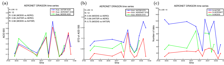
Figure 7. (a) Time series of AOD for the entire DRAGON campaign area for AATSR ADVand , AERONET , and MODIS . The AERONET data has been temporally averaged in a 1 h time-window centred at the AATSR overpass time for each day. Overpasses with less than 10 AATSR or MODIS data points in the area, respectively, are excluded. The error-bars show the spatial standard deviation of AOD AERONET and MODIS data are shown only for the area on days when AATSR data is available. The text inset shows the corresponding day AOD correlation coefficients for three cases: MODIS against AERONET, AATSR against AERONET, and MODIS against AATSR. (b) Corresponding plot for the spatial standard deviation \sigma_{AOD} . (c) The number of AATSR and MODIS pixels in the area for each day, and the number of AERONET sites with data close to the satellite overpass time ( \pm 0.5 h).
