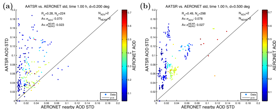
Figure 5. Comparison of spatial aerosol variability estimates between AATSR and AERONET, calculated from the standard deviation of AOD within the sampling distance, for d = 0.2^\circ (a) and d = 0.5^\circ (b). The temporal sampling window used here is \pm 1 h, and at least three observations in the spatial sampling area are required for each data source ( N_{ADV} > 2 and N_{NEAR} > 2 ). The color shows AERONET AOD at 555 nm. Higher AOD values are generally associated with higher variability.
