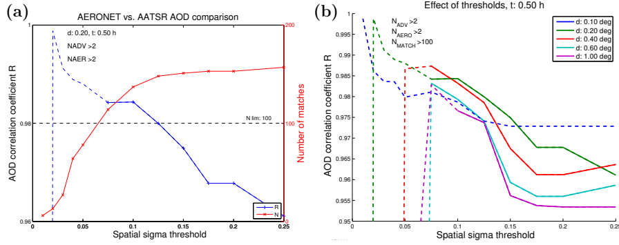
Figure 8. (a) Effect of \sigma_{\text{AATSR}} threshold te-on the AOD comparison with d = 0.2^\circ and \Delta t = 0.5 h. We have also applied the thresholds N_{\text{ADV}} > 2 and N_{\text{AERO}} > 2 to assure-ensure sufficient statistics for calculating \sigma_{\text{AATSR}} . The blue line shows the AOD correlation coefficient R (left y-axis), and the red line shows the corresponding number of matches N (right y-axis) after an upper threshold on \sigma_{\text{AATSR}} (x-axis) has been applied. Results with N < 100 (dashed horizontal black line) are shown by the dashed blue line. (b) The same for various sampling distances. The dashed lines show results for which less than 100 matches are left.
