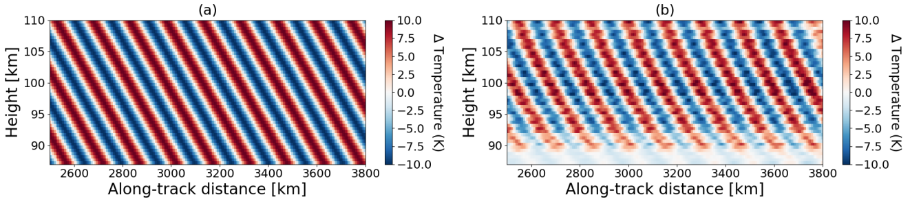
Figure 10. Simulated GW (a) with a vertical wavelength of 10 km and horizontal wavelength of 150 km, and retrieved wave structure (b) assuming a turning angle \alpha of 0^\circ .
