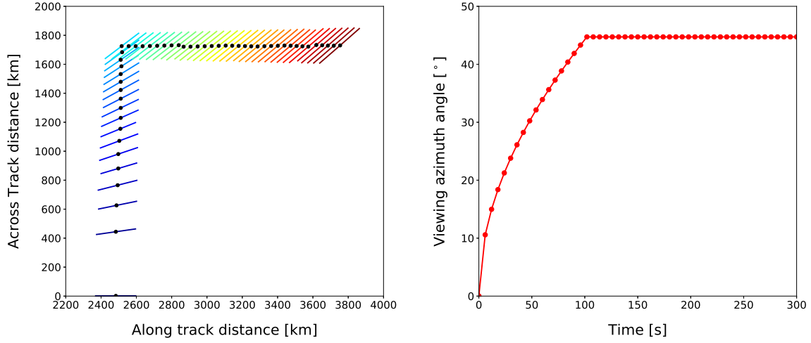
Figure 5. Viewing-angle variations Illustration of simulated the 'sweep mode' measurements central measurement track (a) and viewing angle variations (b). Flight direction is to the right, 0^\circ viewing direction is to the right as well. For a single measurement, the LOS that targets at 70 km tangent altitude is traced. In panel (a), the solid lines indicate the segments of propagation paths between 70 km and 71 km in the atmosphere. The locations of corresponding tangent points are represented by black circles.
