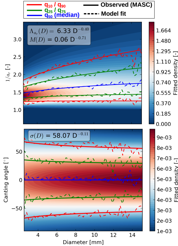
Figure 5. Fitted probability density functions for the inverse of the aspect-ratio (top) and the canting angle (bottom). The power-laws relating the particle density function parameters to the diameter are displayed in the grey boxes on the top-left. Note that the fit was performed on the inverse of the aspect-ratio (major axis over minor axis).
