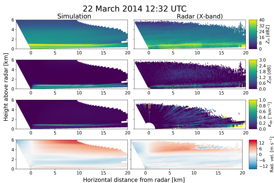
Figure 10. Example of RHI showing the observed and simulated melting layer during the PARADISO campaign in Spring 2014 (Table 3). The left panel corresponds to the simulated radar observables, the right panel to the observed values at X-band. Note that there is an area with velocity folding (blue area in the middle of a larger red area) around 5 km altitude and 10-15 km horizontal distance on the radar RHI scan.
