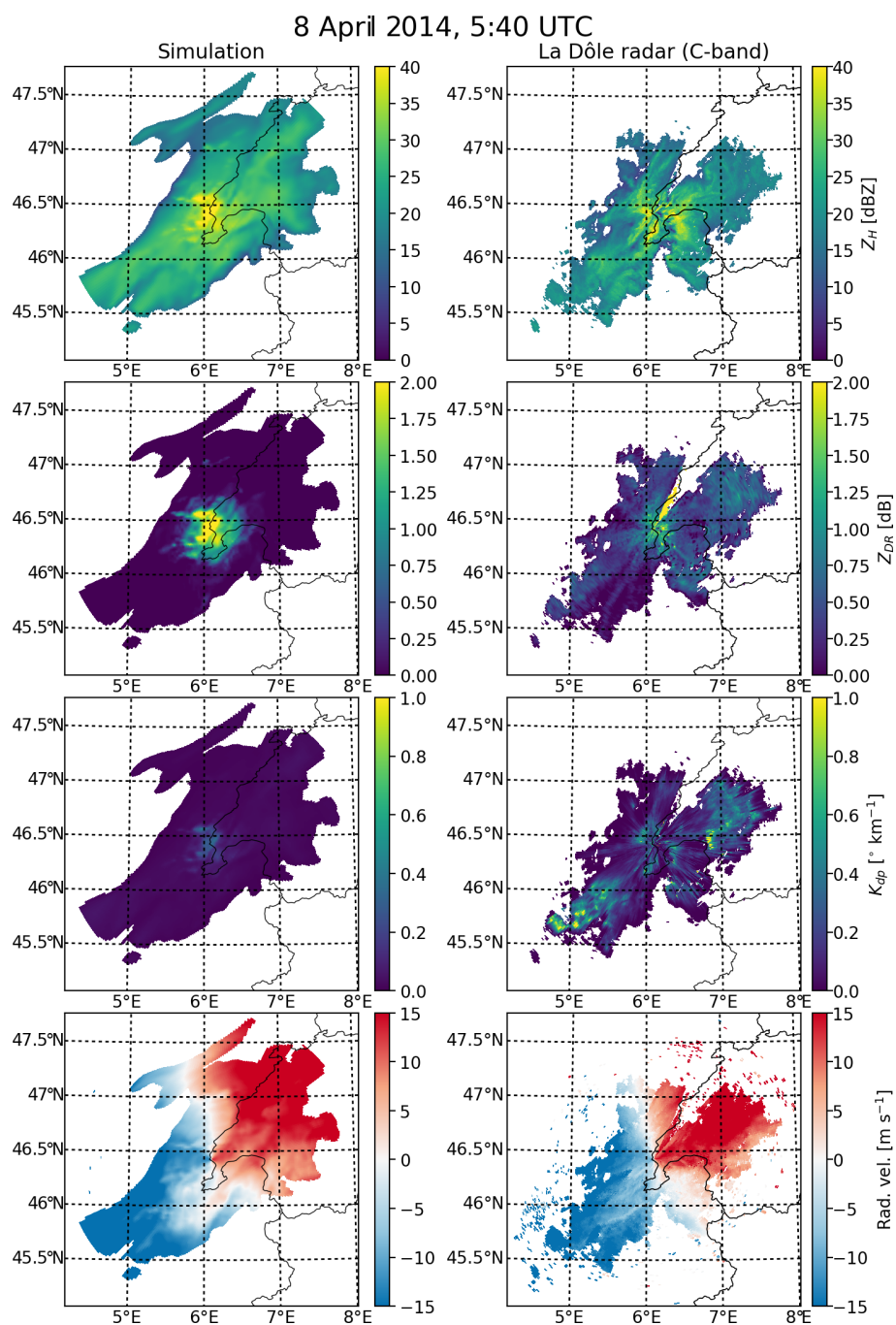
Figure 9. Same as Figure 8 but for the stratiform event on the 8 April 2014 (Table 3).
