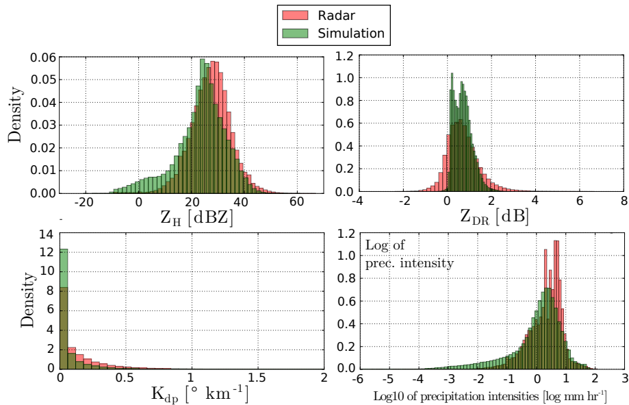
Figure 15. Observed (red) and simulated (green) distributions of polarimetric variables ( Z_H , Z_{DR} and K_{dp} ) as well as the precipitation intensities on the ground (in log scale) for the one-moment scheme with \mu^{\text{rain}} = 2 in the liquid phase.
