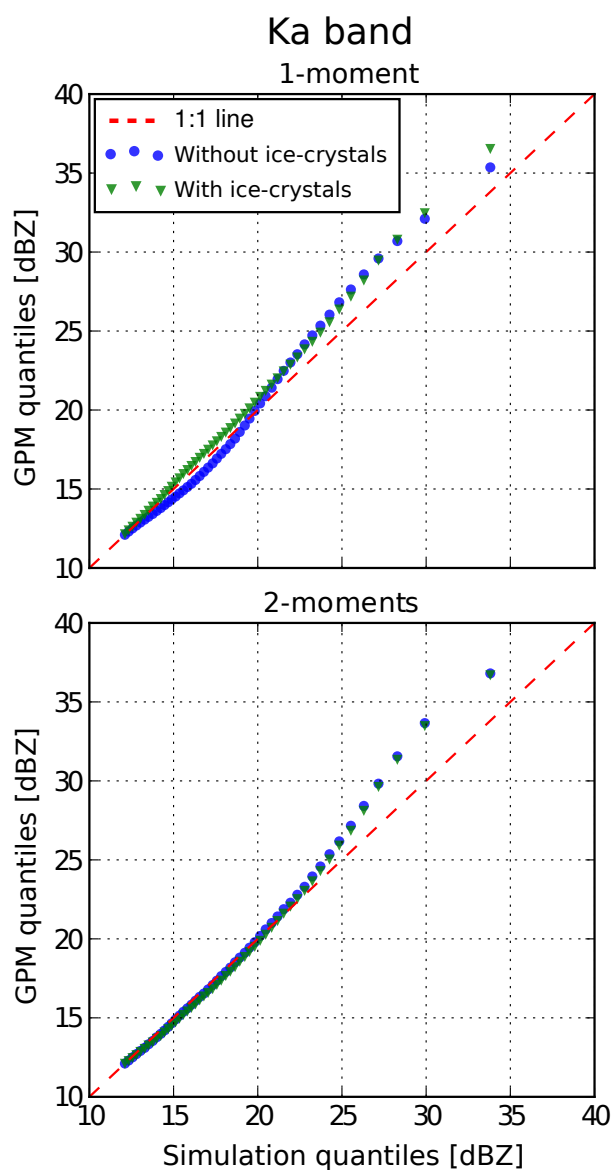
Figure 20. QQ-plots of the quantiles of simulated Z_H values versus the quantiles of observed GPM Z_H values at Ka band. The red line corresponds to the 1:1 line indicating a perfect match with observed quantiles.
