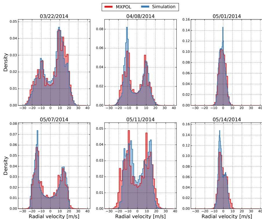
Figure 12. Distributions of simulated (blue) and observed (red) radial velocities at X-band during six days of precipitation in Western Switzerland.
