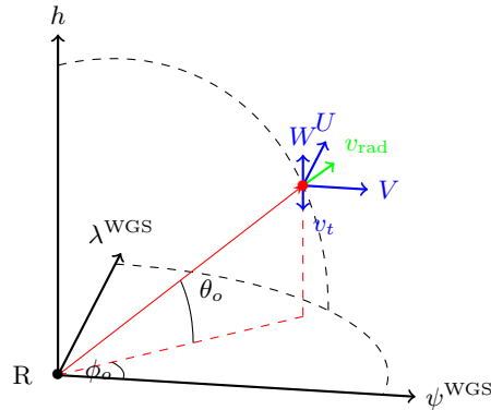
Figure 7. Trigonometric expression of the radial velocity as the power-weighted sum of the projection into the beam axis of the 3-dimensional wind field ( U, V, W ) and the hydrometeor terminal velocity v_t .
