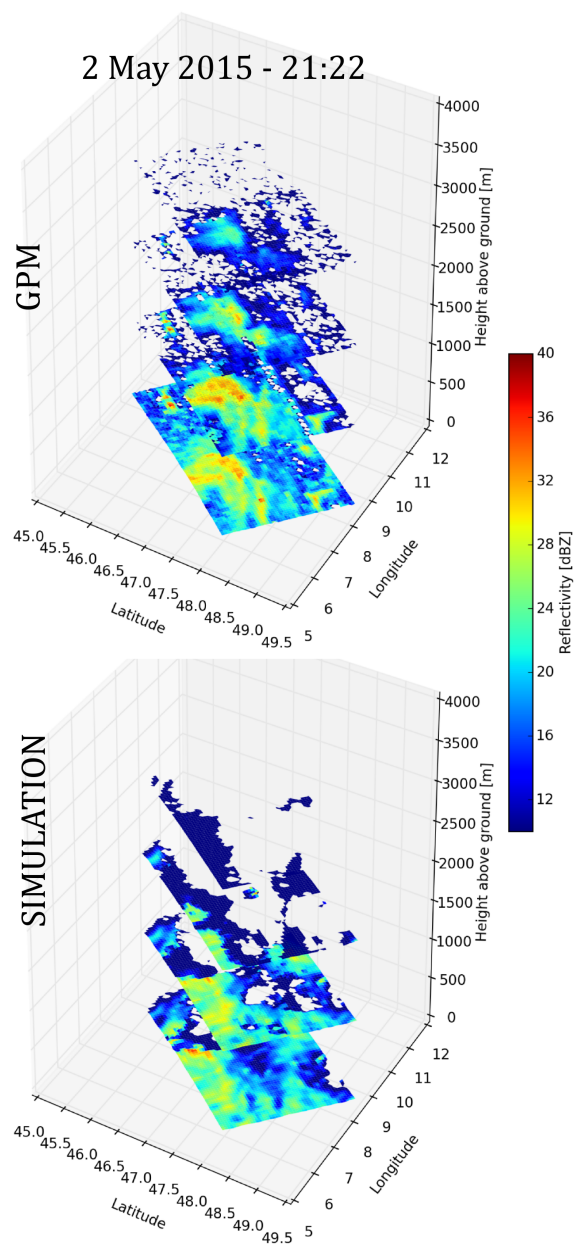
Figure 11. Example of comparison at several altitude levels between GPM radar observations at Ka band (top) and the corresponding radar operator simulation from the COSMO model (bottom) for one GPM overpass.
