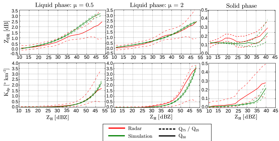
Figure 16. Observed (red) and simulated (green) Z_H - Z_{DR} and Z_H - K_{dp} relationships for the COSMO one-moment scheme in liquid and solid phases. These membership functions are computed by dividing all simulated values in bins of reflectivity of 1 dBZ of width, and computing the quantiles of the dependent variable (on the y -axis) within every bin.
