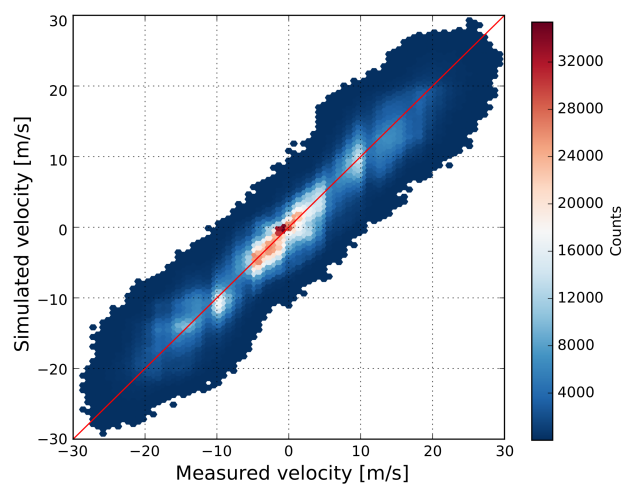
Figure 13. Scatter-plot of the measured and simulated radial velocities (for all events). The red line shows the 1:1 relation. The coefficient of determination ( R^2 ) is 0.9.
