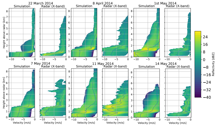
Figure 14. Simulated and measured daily averaged Doppler spectrum at X-band at vertical incidence during six days of precipitation in Western Switzerland. The dashed line represents the radial velocity calculated from the spectrum (Equation 35)
