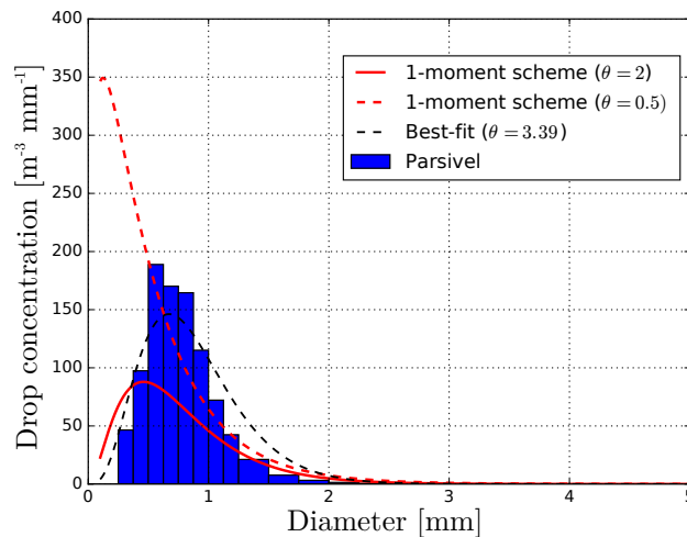
Figure 17. Average measured (blue bins) and parameterized rain DSDs at the ground in Payerne over six stratiform precipitation events. The dashed black line corresponds to the best fit of a gamma DSD on the measurements
