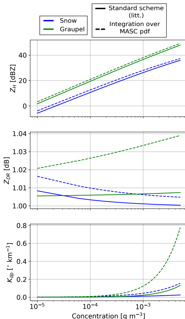
Figure 6. Polarimetric variables as a function of the mass concentration for snow and graupel when using canting angle and aspect-ratio parameterizations from the literature (Ryzhkov et al., 2011) (solid line) and when using the parameterization based on MASC data (dashed line).
