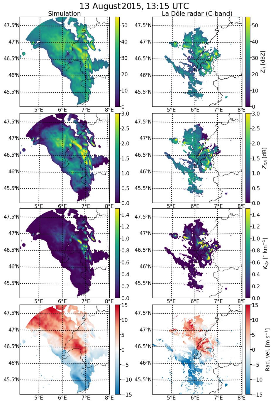
Figure 8. Example of simulated and observed (with the Swiss La Dôle C-band radar) PPI at 1^\circ elevation during the 13 August 2015 convective event (Table 3). The left side panel corresponds to the simulated radar observables and the right side to the observed ones. The displayed variables are, from top to bottom, the horizontal reflectivity factor (in dBZ), the differential reflectivity (in dB), the specific differential phase shift upon propagation (in ^\circ\text{km}^{-1} ), and the radial velocity (in \text{m s}^{-1} ).
