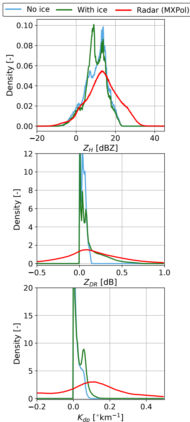
Figure 19. Observed and simulated (with and without ice crystals) distributions of polarimetric variables during three pure snowfall events for the one-moment microphysical scheme.
