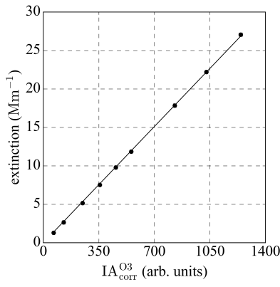
Figure 3: Photoacoustic spectrometer response (microphone integrated area (IA)) and concurrent cavity ring-down spectrometer extinction coefficient for nine ozone concentrations at wavelength 405 nm. Each point is the mean of 90 seconds of 1Hz data and error bars represent the 2\sigma precision of each measurement; these are not discernible by eye due to the excellent precision.
