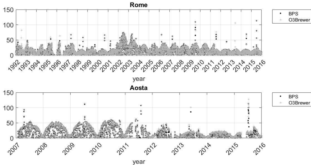
Figure 10. Time plot of the number of individual ozone values per day.
