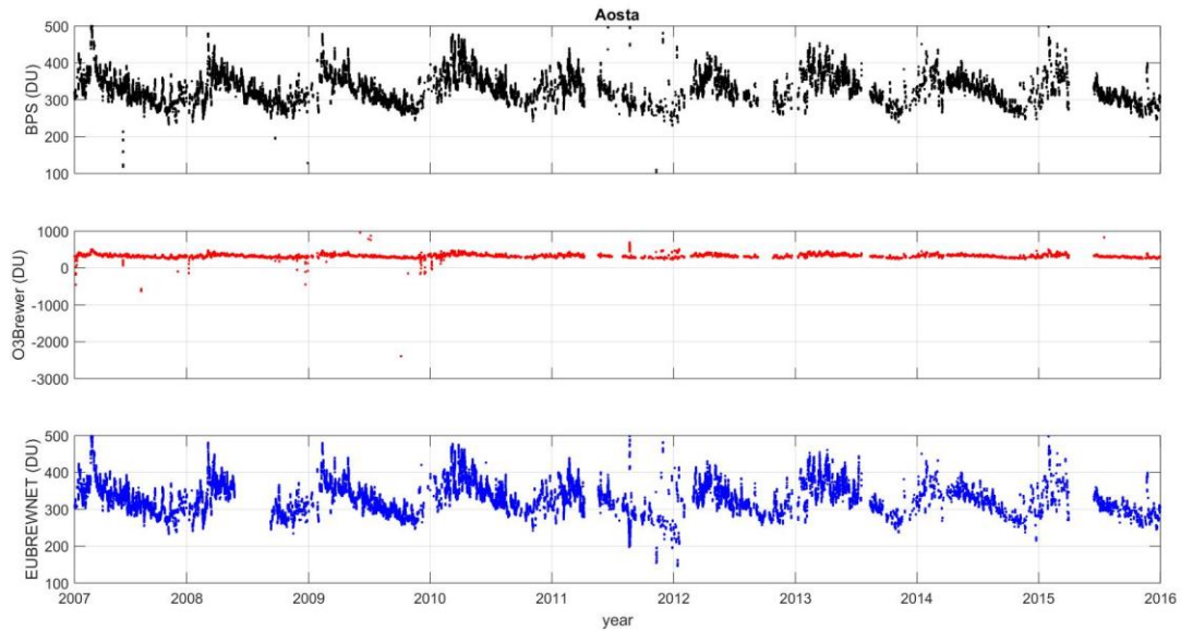
Figure 3. Individual TOC values generated by BPS (black), O3Brewer (red) and EUBREWNET (blue) at Aosta.
