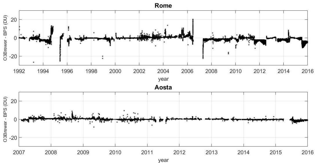
Figure 12. Difference between individual TOC values generated by BPS and O3Brewer at Rome (upper panel) and at Aosta (bottom panel) when anomalous values were discarded.
