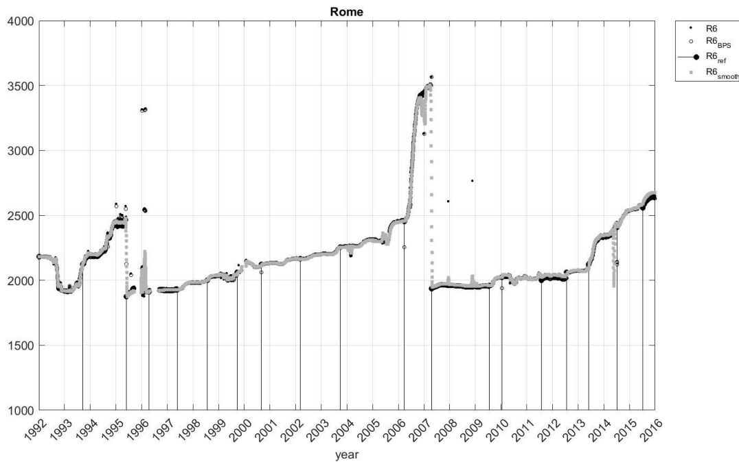
Figure 8. Daily series of the ratios R6 , R6_{BPS} and R6_{smooth} at Rome. Vertical lines represent R6_{ref} established during each calibration campaign.
