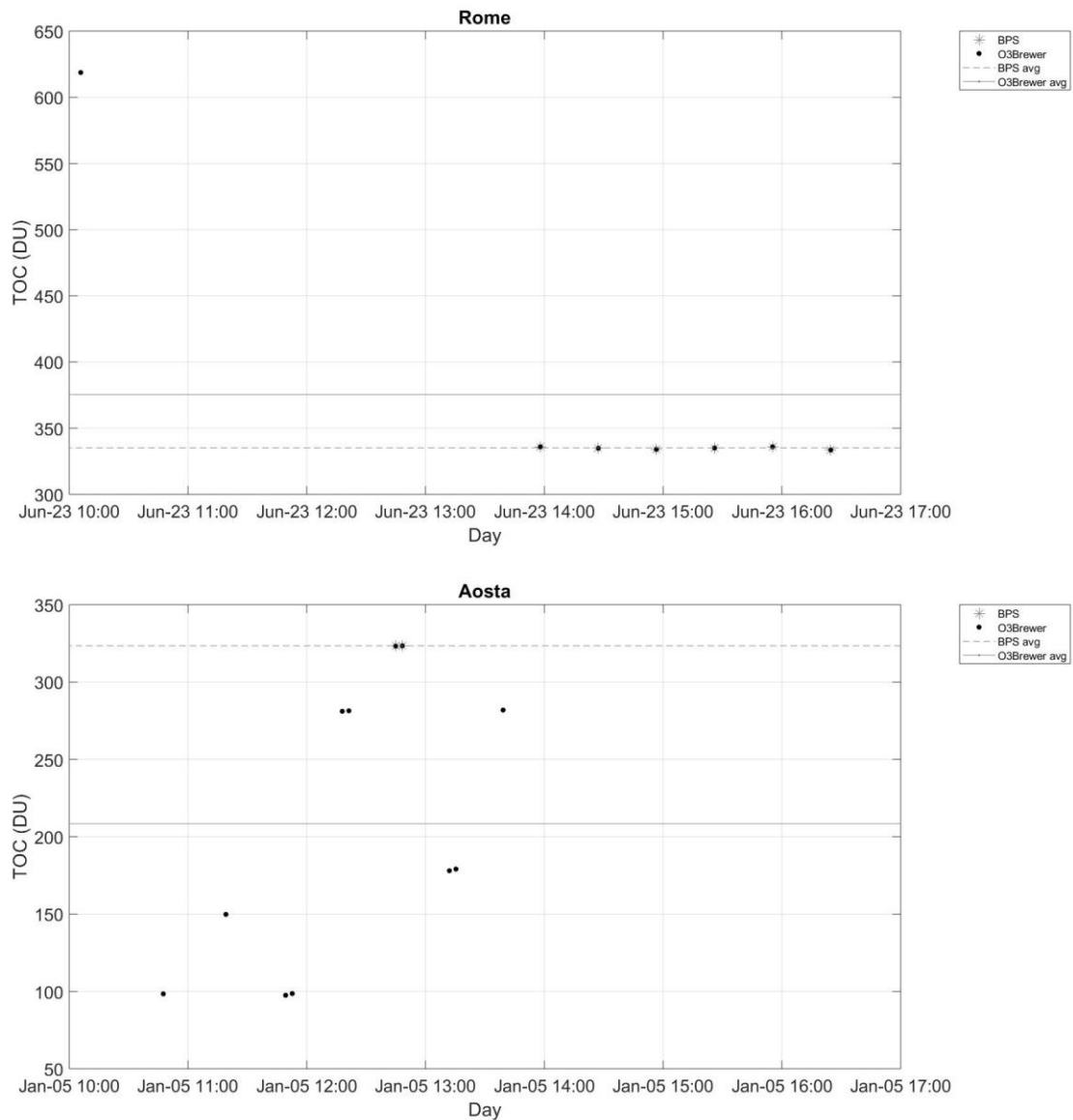
Figure 11. Individual TOC values generated by BPS and O3Brewer on 23/06/2001 at Rome (upper panel) and on 5/1/2010 at Aosta (bottom panel) taken as examples where large difference between occurred although the SL correction is similar. Horizontal lines (dashed for BPS; solid for O3Brewer) represent the daily average (avg).
