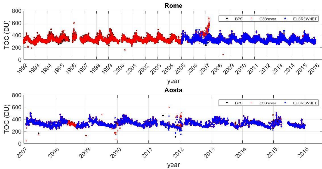
Figure 1. Time series of TOC daily means from BPS (black), O3Brewer (red) and EUBREWNET (blue) at Rome (upper panel) and at Aosta (lower panel). At Aosta the EUBREWNET L1.5 ozone values were not generated between May 24 and September 8, 2008, because the standard lamp got burned out since May 2008 and was replaced in September 2008.
