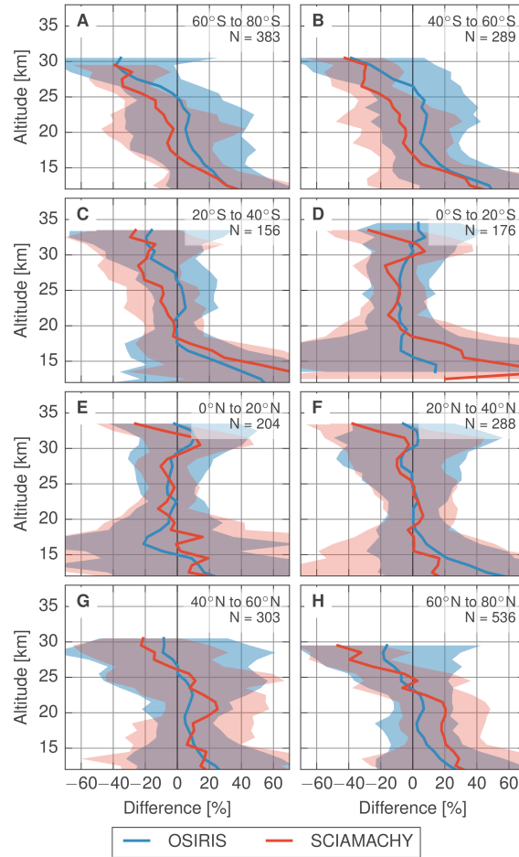
Figure 8. Coincident comparison with SAGE II when both OSIRIS and SCIAMACHY measurements have been processed with the USask algorithm.
