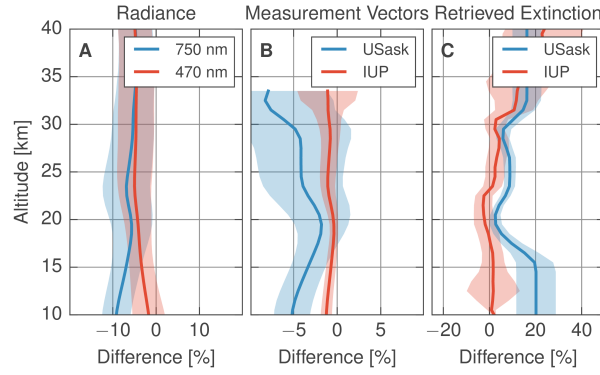
Figure 2. Comparisons of the radiative transfer models. Panel A shows the differences in radiance computed using SASKTRAN and SCIA-TRAN. Panel B shows the difference in measurement vectors. Panel C shows the difference in retrieved profiles. Differences in Panels A and B are computed as (\text{SASKTRAN} - \text{SCIATRAN}) / (\text{SASKTRAN} + \text{SCIATRAN}) \times 200\% . Extinction error is computed as (\text{Retrieved} - \text{True}) / \text{True} \times 100\% .
