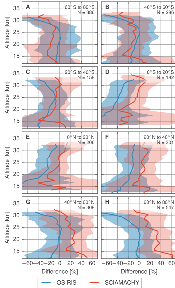
Figure 9. Coincident comparison with SAGE II when both OSIRIS and SCIAMACHY measurements have been processed with the IUP algorithm.
