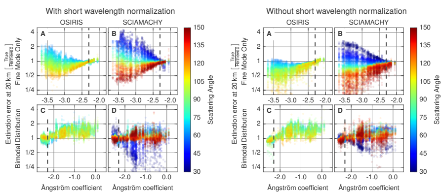
Figure 7. Error in the retrieved USask extinction as a function of Ångström coefficient at 20 km. The colour of the points show the solar scattering angle. The top row shows the error for conditions when only a fine mode of aerosol is present. The bottom row shows the error when there is both a fine and coarse mode distribution. The black dashed line indicates the Ångström coefficient corresponding to the particle size distribution used in the retrievals.
