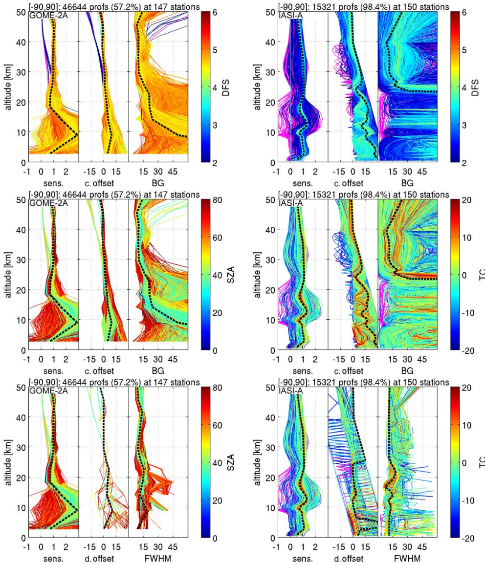
Figure 5: Global GOME-2A (left) and IASI-A (right) information content in terms of vertical sensitivity, retrieval offset (in km), and averaging kernel width (in km) and their dependence on DFS, SZA, or thermal contrast (TC). Black dashed lines represent median values, while out-of-range profiles are plotted in magenta. Different measures are used for the offset and kernel width in the second and third rows, which include the centroid offset (c. offset) and Backus-Gilbert spread (BG), and the direct offset (d. offset) and FWHM, respectively. Plot titles provide the absolute and relative amounts of profiles after screening, and the number of ground-based overpass stations.
