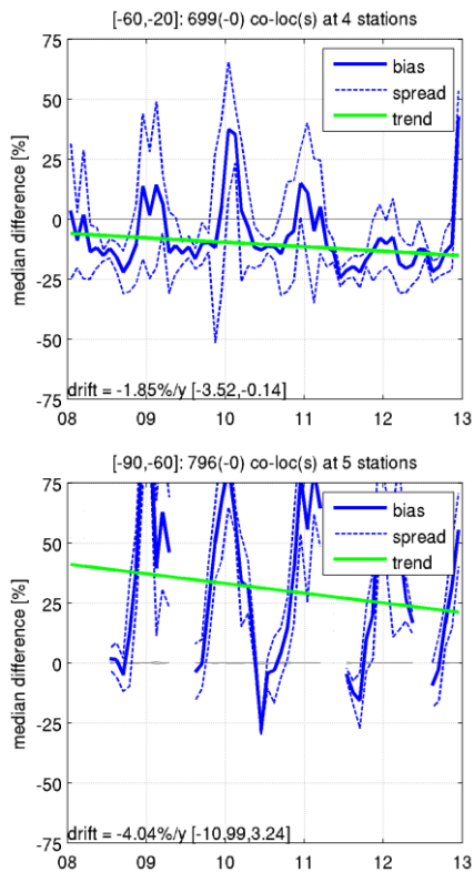
Figure 16: Time series of the median bias (solid blue), spread (dashed blue), and linear drift (green line) for direct comparisons of IASI L3 monthly gridded mean tropospheric ozone column data (0 to 6 km) with vertically integrated ozonesonde reference data (at stations with at least six launches per month), divided into five latitude bands (sorted north to south). The number of filtered values is added between brackets in the title of each plot, while the yearly linear drift value and its 95 % confidence interval are added in the lower-left corner.
