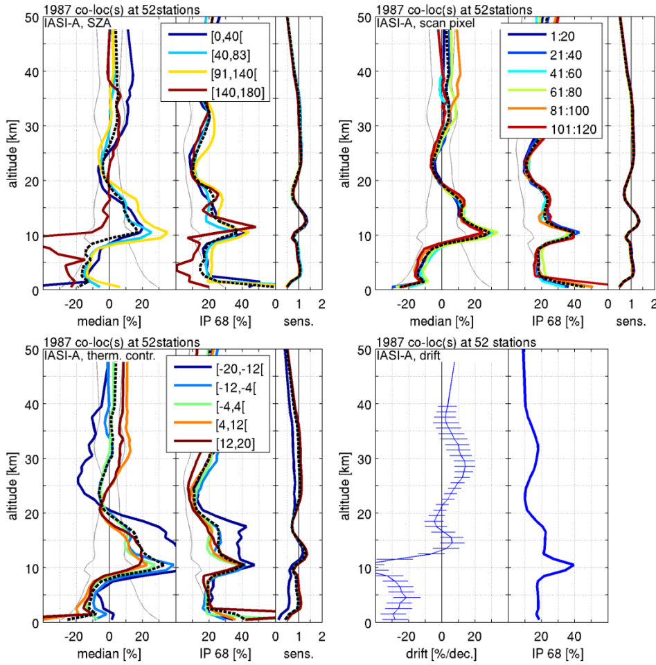
Figure 14: Median relative differences, 68% interpercentile spreads, and vertical sensitivities for comparison of FORLI v20151001 L2 IASI-A retrieved profiles with ground-based reference measurements (2008-2015). The same difference and information statistics are redistributed in each plot over several influence quantity ranges, with the influence quantities being (from left to right and top to bottom) latitude, quarter, total ozone column (DU), DFS, SZA, scan pixel index, and thermal contrast. In the corresponding legend entries, open brackets are used to indicate that the last value is not included (i.e. values in the set go up to, but don't equal the last value). The black dashed line shows the average of the coloured curves, while light grey lines indicate the satellite uncertainty provided in the product.. The bottom right plot contains the corresponding relative decadal drift and 68% interpercentile spread. Two sigma error bars, resulting from a bootstrapping with 1000 samples, are added to the drift profile.
