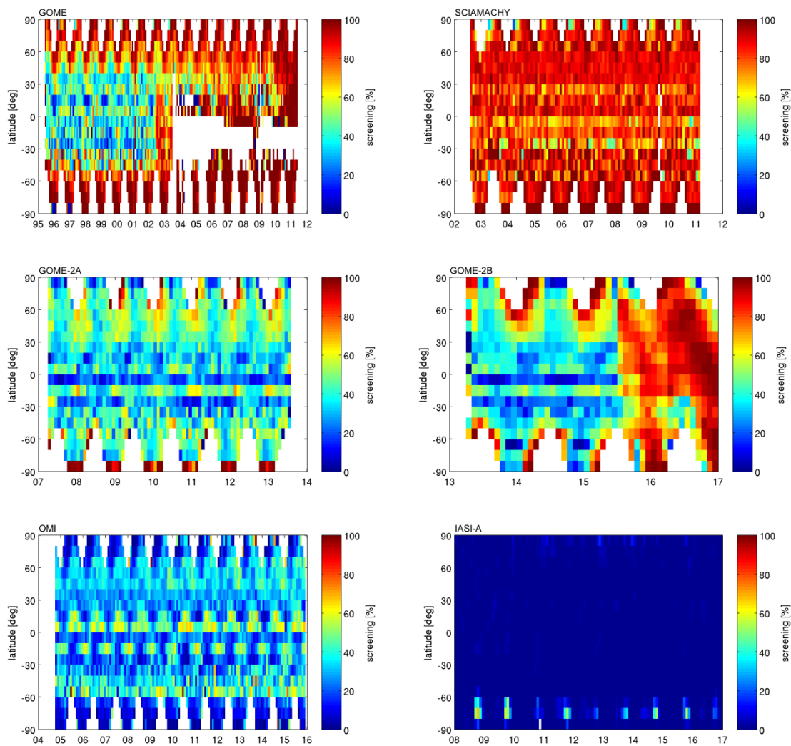
10 Figure 3: GOME, SCIAMACHY, GOME-2A, GOME-2B, OMI, and IASI-A (left to right and top to bottom) latitude-time distribution of relative data screening, taking into account the quality flags presented in Table 3. The decreased GOME-2B availability from June 2015 onwards points at a retrieval issue. IASI-B is fully similar to IASI-A.
