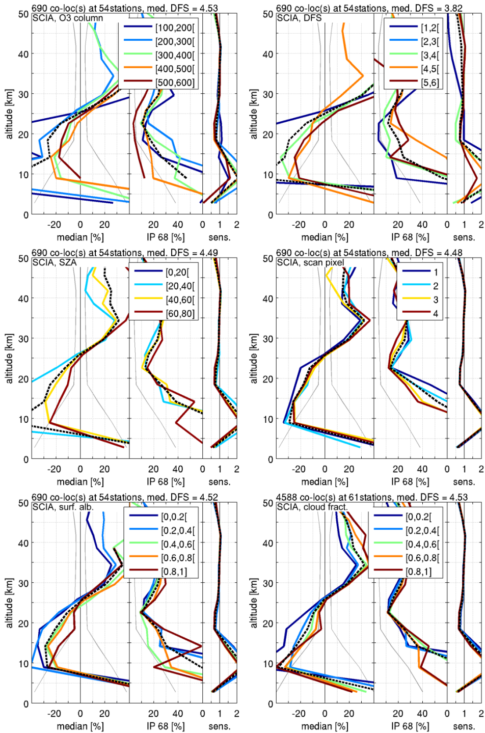
Figure 7: As for Figure 6, but for RAL v2.14 L2 SCIAMACHY data (2003-2010).
