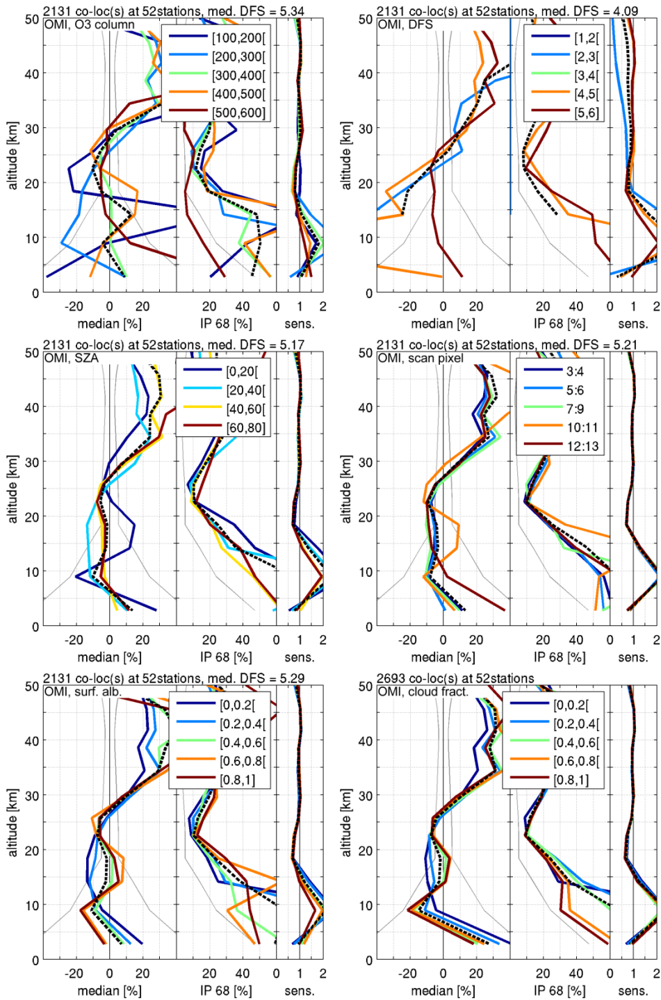
Figure 10: As for Figure 6, but for RAL v2.14 L2 OMI data (2005-2015).
