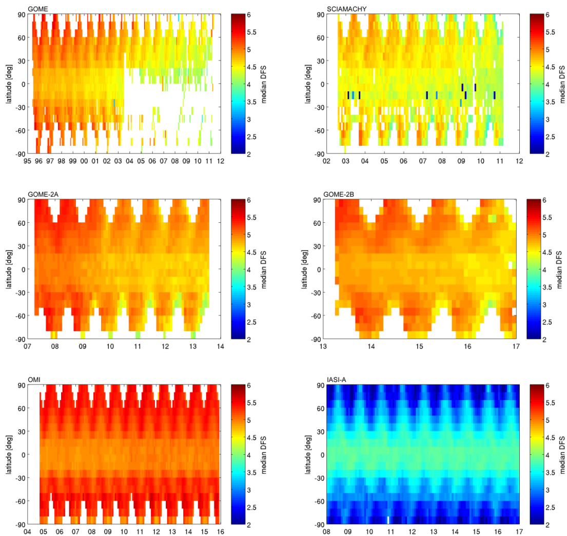
10 Figure 4: GOME, SCIAMACHY, GOME-2A, GOME-2B, OMI, and IASI-A (left to right and top to bottom) latitude-time distribution of degrees of freedom in the signal (DFS). IASI-B is fully similar to IASI-A.
