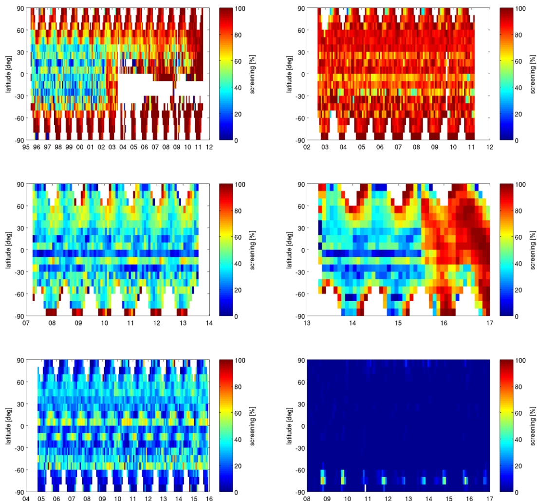
5 Figure 3: GOME, SCIAMACHY, GOME-2A, GOME-2B, OMI, and IASI-A (left to right and top to bottom) latitude-time distribution of relative data screening, taking into account the quality flags presented in Table 3. The decreased GOME-2B availability from June 2015 onwards justifies additional screening. IASI-B is fully similar to IASI-A.
