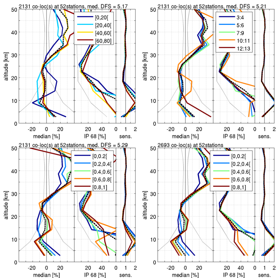
Figure 10: As for Figure 6, but for RAL v2.14 L2 OMI data (2005-2015).
