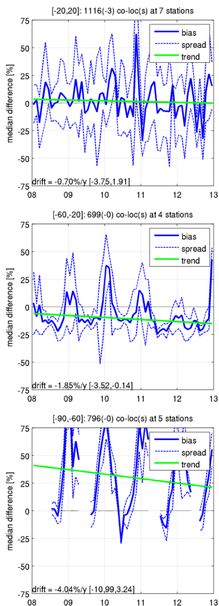
5 Figure 16: Time series of the median bias (solid blue), spread (dashed blue), and linear drift (green line) for direct comparisons of IASI L3 monthly gridded mean tropospheric ozone column data (0 to 6 km) with vertically integrated ozonesonde reference data (at stations with at least six launches per month), divided into five latitude bands (sorted north to south). The number of filtered values is added between brackets in the title of each plot, while the yearly linear drift value and its 95 % confidence interval are added in the lower-left corner.
