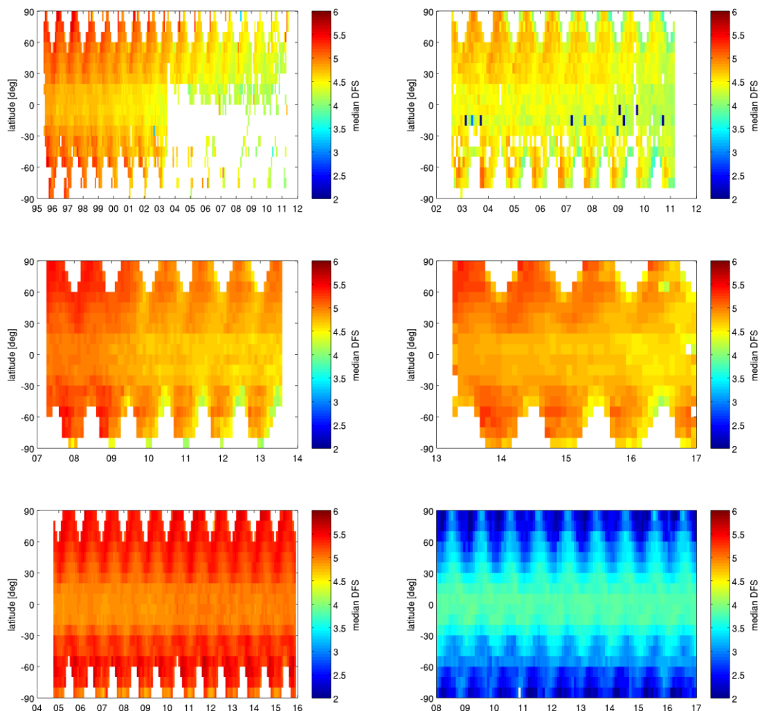
5 Figure 4: GOME, SCIAMACHY, GOME-2A, GOME-2B, OMI, and IASI-A (left to right and top to bottom) latitude-time distribution of degrees of freedom in the signal (DFS). IASI-B is fully similar to IASI-A.
