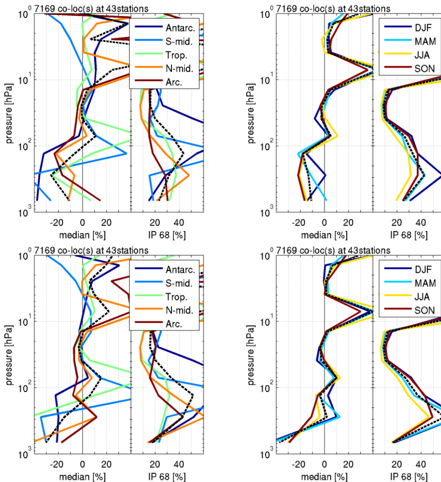
Figure 11: Median relative differences and 68% interpercentile spreads for comparison of L3 GOME, SCIAMACHY, GOME-2A, and OMI data (top to bottom) with ground-based reference measurements. The same difference statistics are redistributed in each line over two influence quantity ranges, with the influence quantities being the latitude (left) and quarter (right). The black dashed line shows the average of the coloured curves.
