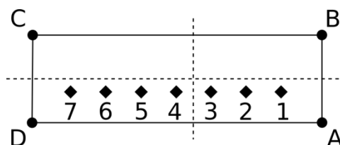
5 Figure 1: A L2 ground pixel ABCD is divided into ground subpixels (diamonds 1 to 7). Each subpixel is assigned to a TM5 assimilation grid cell (dashed) and the average and standard deviation are calculated (see text).
