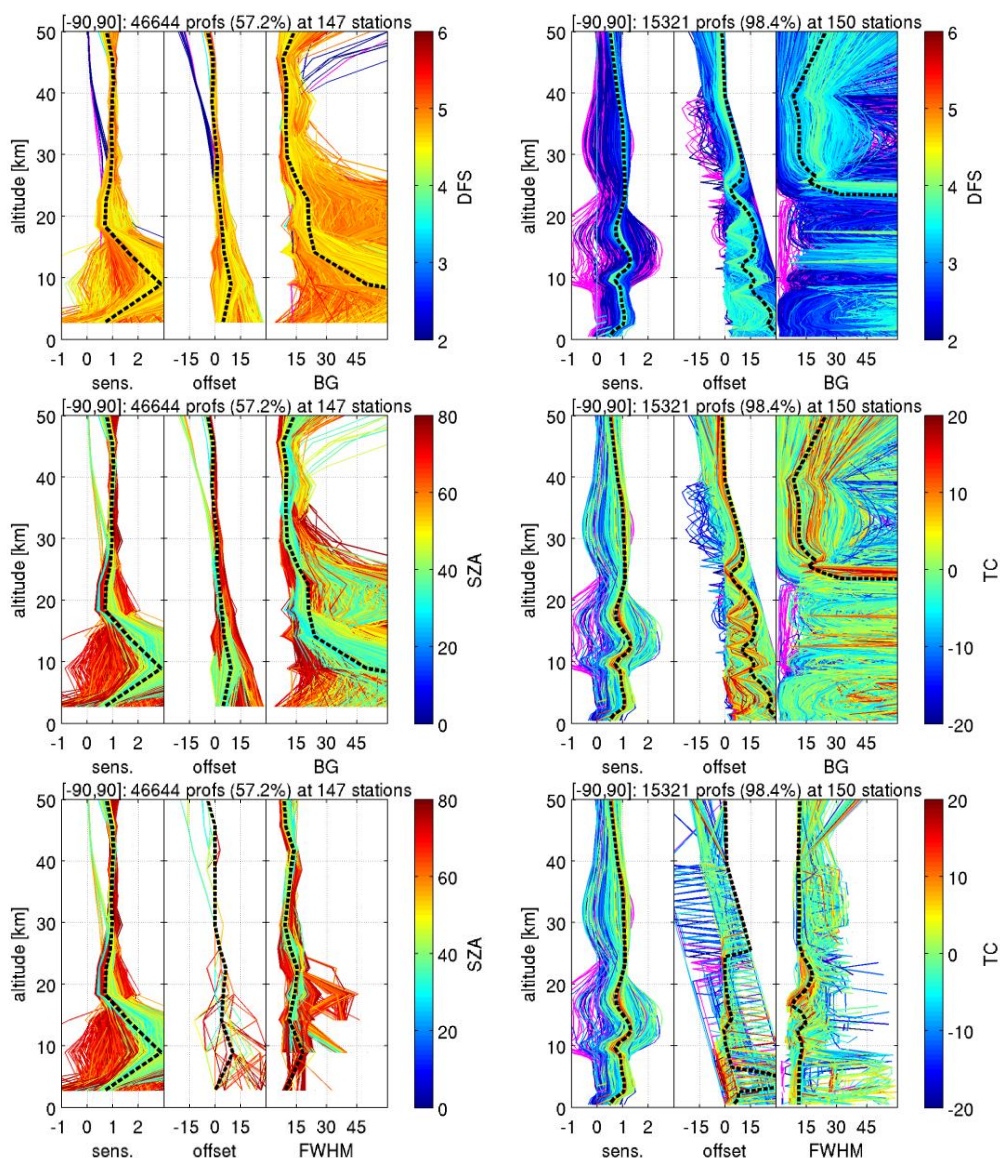
5 Figure 5: Global GOME-2A (left) and IASI-A (right) information content in terms of vertical sensitivity, retrieval offset (in km), and averaging kernel width (in km) and their dependence on DFS, SZA, or thermal contrast (TC). Out-of-range profiles are plotted in magenta. Different measures are used for the offset and kernel width in the second and third rows. Plot titles provide the absolute and relative amounts of profiles after screening, and the number of ground-based overpass stations.
