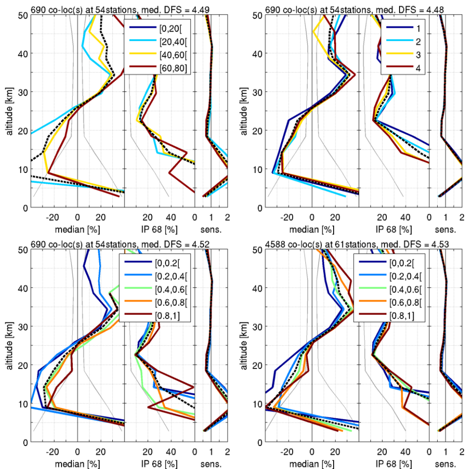
Figure 7: As for Figure 6, but for RAL v2.14 L2 SCIAMACHY data (2003-2010).
