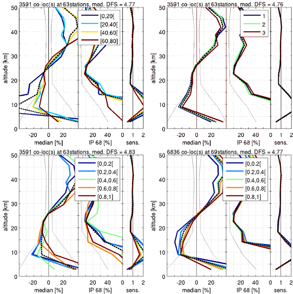
5 Figure 6: Median relative differences, 68% interpercentile spreads, and vertical sensitivities for comparison of RAL v2.14 L2 GOME retrieved profiles with ground-based reference measurements (1996-2010). The same difference and information statistics are redistributed in each plot over several influence quantity ranges, with the influence quantities being (from left to right and top to bottom) latitude, quarter, total ozone column (DU), DFS, SZA, scan pixel index, surface albedo, and effective cloud fraction. The black dashed line shows the average of the coloured curves, while light grey lines indicate the satellite uncertainty provided in the product. The number of comparisons is higher for the latter as the ECF filter has been switched off.
