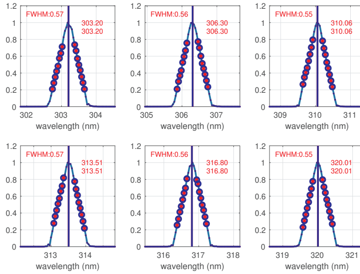
Figure 1. Results of Brewer measurements in the ozone mode obtained while the laser wavelength [.. 35 ] was changed every [.. 36 ] 0.04 nm. The central wavelength and the FWHM calculated are displayed in red using the same methodology of the dispersion test.
