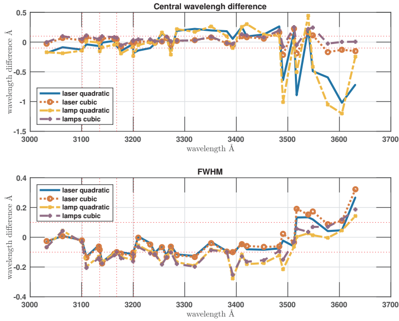
Figure 7. [.95] Differences between the central wavelengths (upper panel) and FWHMs (lower panel) determined directly and by the scanning methods: with the laser wavelengths in [.96] equally spaced grid every 5 nm and lines of the discharge lamps; in both cases quadratic and cubic fits are used.
