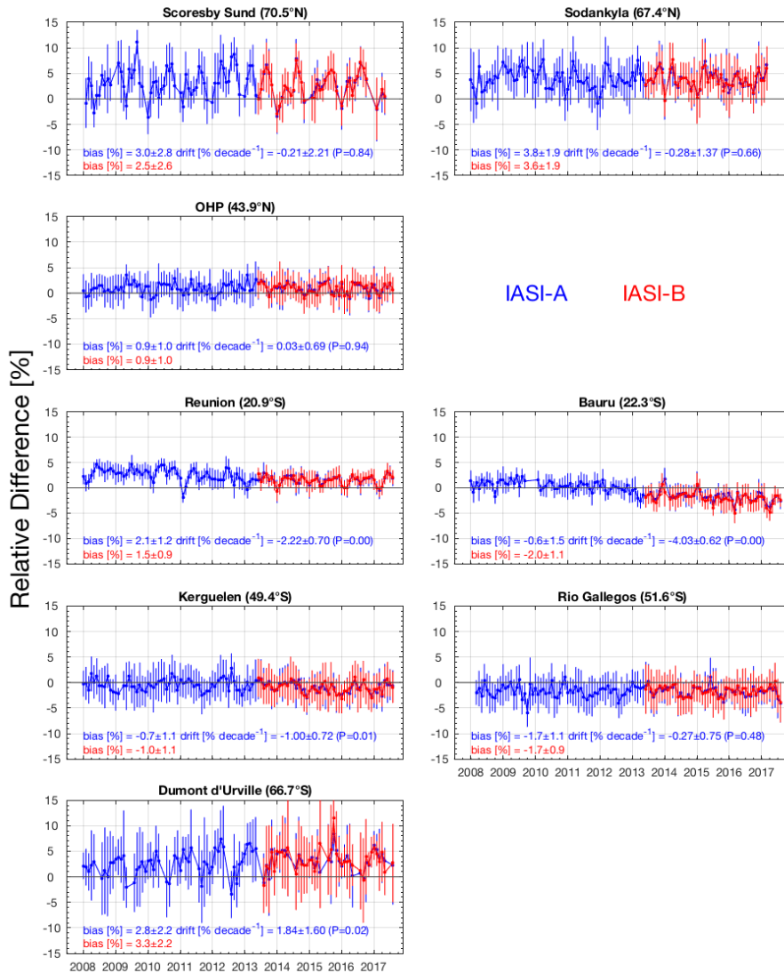
5 Figure 11: Time series of the monthly relative differences (in percent) between IASI-A (blue) and IASI-B (red) against collocated 10 SAOZ TOC measurements for eight stations from North to South. For each daily SAOZ measurement, a relative difference is calculated as 100 \times (\text{IASI} - \text{SAOZ}) / \text{SAOZ} [\%] . All the relative differences are then monthly averaged. For the period May 2013 onwards, only the common collocations between IASI-A and IASI-B are shown. The standard deviation of the average is also displayed (vertical bars). Comparison statistics including the mean bias and its 1- \sigma standard deviations in % for the period 2008 – 2017 (IASI-A) and 2013 – 2017 (IASI-B) are indicated on each panel. The decadal drift, its 2- \sigma standard deviation (in %) and the P value for the IASI-A time series are also indicated on each panel.
