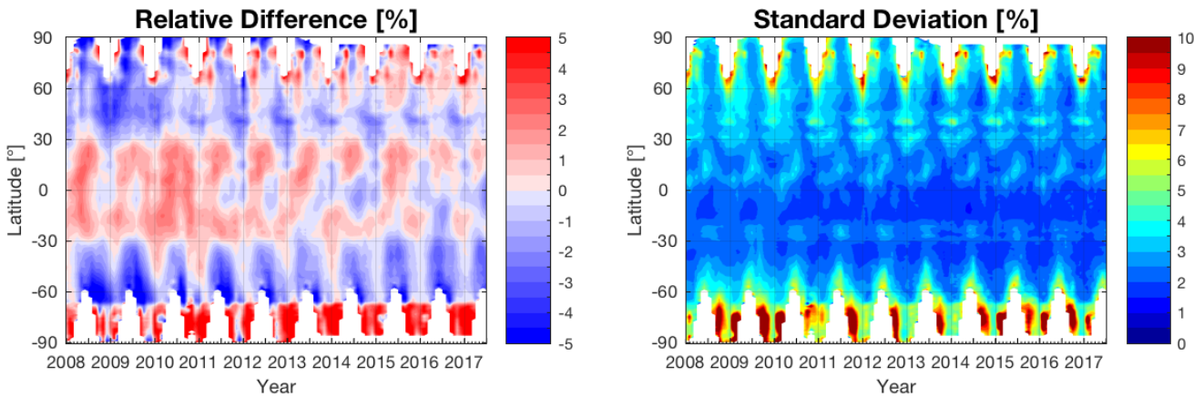
15 Figure 6: (left) Relative differences (in percent) between IASI-A and GOME-2A for 1° zonal monthly mean Total Ozone Columns during the period 2008 – 2017; (right) Associated standard deviation (in percent). The relative difference is calculated as 100 \times (\text{IASI-A} - \text{GOME-2A}) / \text{GOME-2A} .
