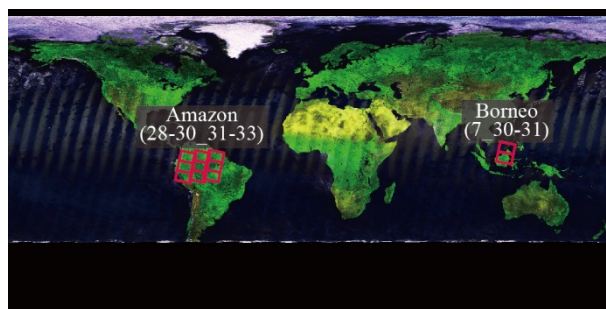
10 Figure 4: Study areas in Borneo and the Amazon. CAI path and frame system: XX_YY (XX indicates CAI path number and YY indicates CAI frame number). Red rectangles indicate the locations of CAI frames. The background image was generated from the CAI L3 global reflectance distribution product (15 June 2013 to 14 July 2013). (single column)
