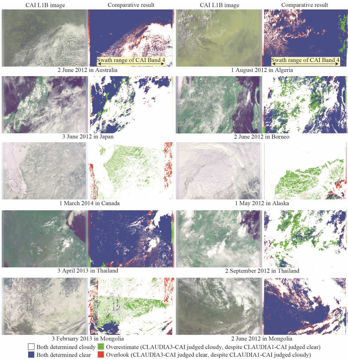
Figure 10: CAI L1B images (R: Band 2, G: Band 3, B: Band 1) and comparative results of CLAUDIA1-CAI and CLAUDIA3-CAI for various land cover types. (2 column)
