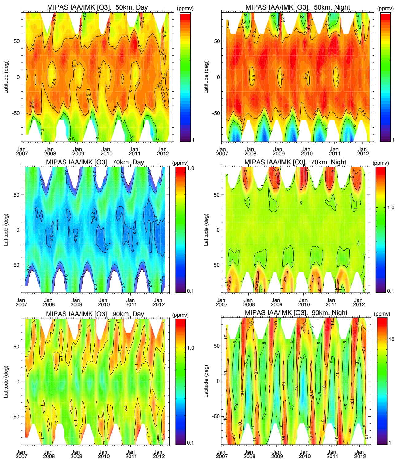
Figure 14. Cross section of latitude/time MIPAS O 3 at 50 km, 70 km and 90 km for daytime (left column) and nighttime (right column). Note the different color scales in some panels.
