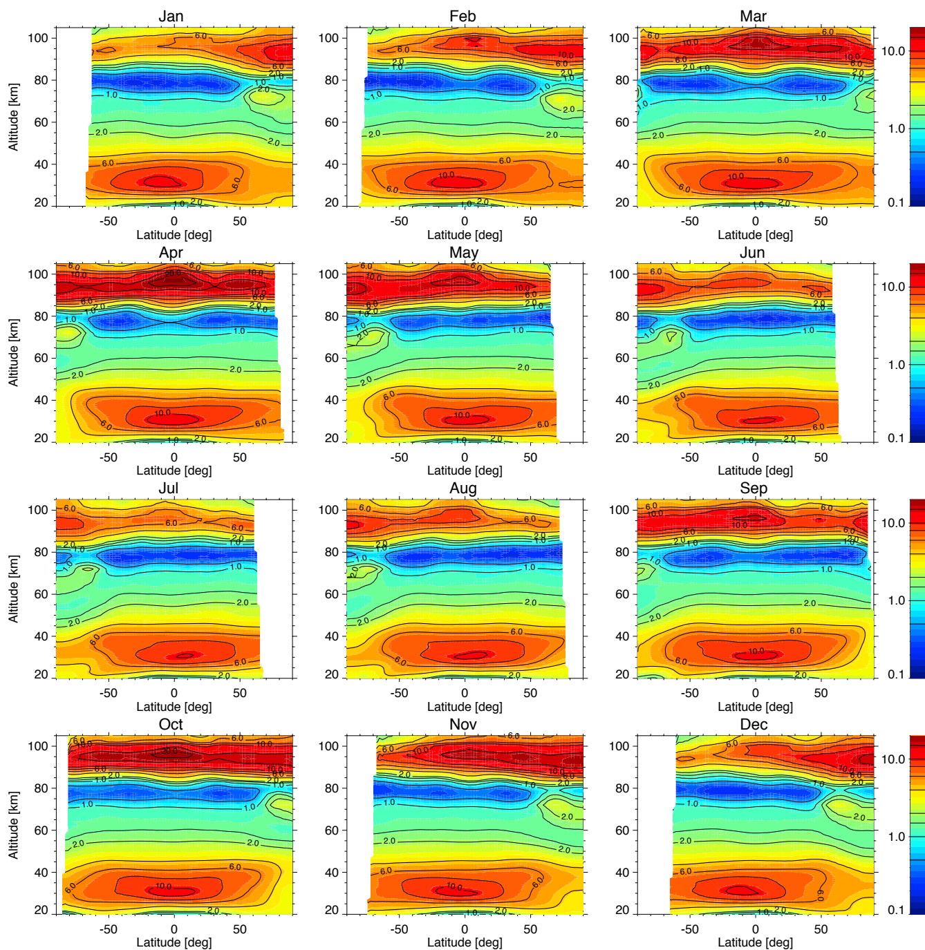
Figure 11. Composite monthly zonal mean of MIPAS data for the 2017-2012 period for nighttime. Contours are 0.5, 1, 1.5, 2, 4, 6, 8, 10, 15, and 20 ppmv.
