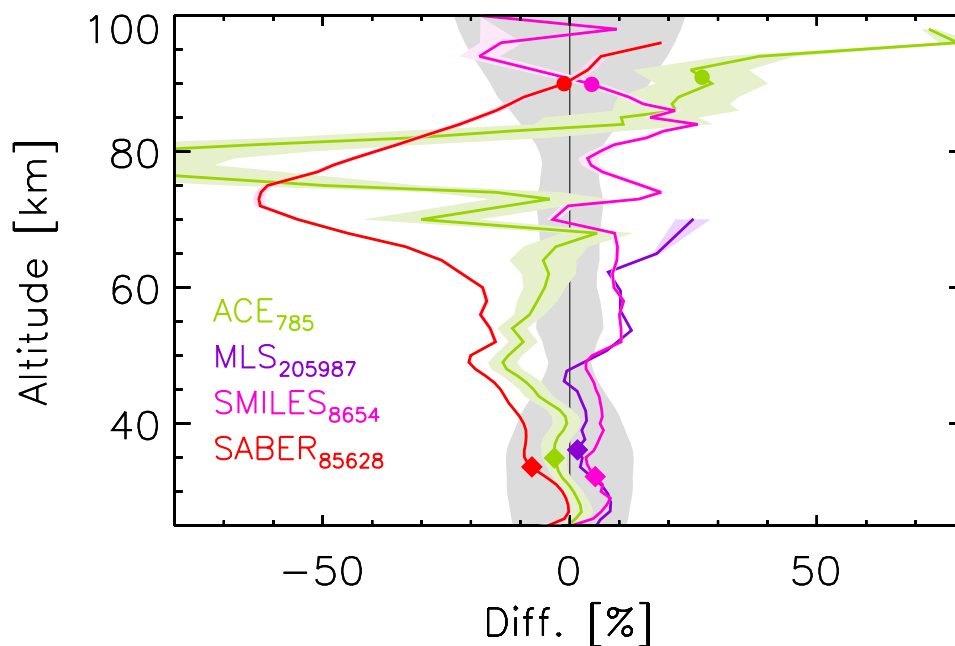
Figure 8. Global mean (for all latitudes and seasons) of the daytime O 3 vmr differences (MIPAS–instrument) in % of MIPAS between co-located pairs of measurements of MIPAS (MA mode) with ACE-FTS (green), SABER (red), MLS (purple), and SMILES (magenta). For more details see caption of Fig. 6.
