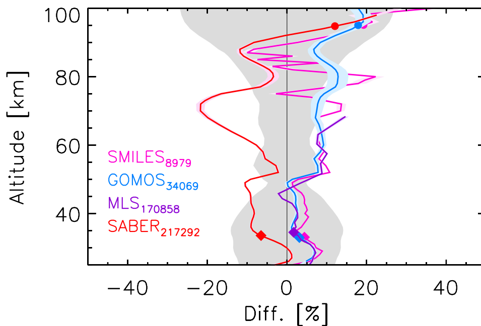
Figure 9. As Fig. 8 but for nighttime O 3 . Instruments colors are the same except that ACE-FTS is replaced by GOMOS (light blue).
