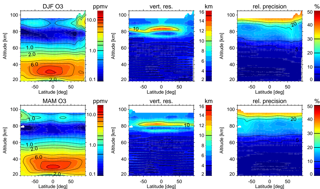
Figure 2. Latitude-altitude cross sections of MIPAS MA daytime ozone (left), its vertical resolution (center) and single profile noise error ( 1-\sigma , right) for solstice (December-January-February: DJF) (top row) and equinox (March-April-May; MAM) (bottom row). All measurements from 2005 to 2012 are included. White areas denote regions where the retrieved O_3 is not significant. Contour lines are marked in the color bar scale.
