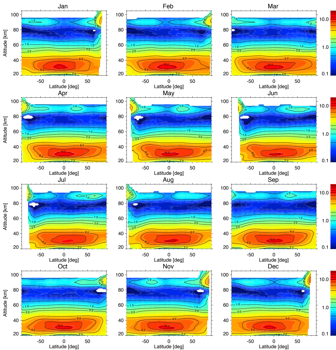
Figure 10. Composite monthly zonal mean of MIPAS data taken in the MA mode for the 2007-2012 period for daytime (local time of 10 am). White areas denote regions where MIPAS has no sensitivity to measure the very low ozone values. Contours are 0.1, 0.5, 1, 1.5, 2, 4, 6, 8, 10 and 12 ppmv.
