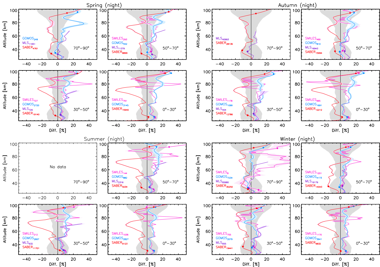
Figure 7. As Fig. 6 but for nighttime O_3 . Instruments colors are the same except that ACE-FTS is replaced by GOMOS (light blue).
