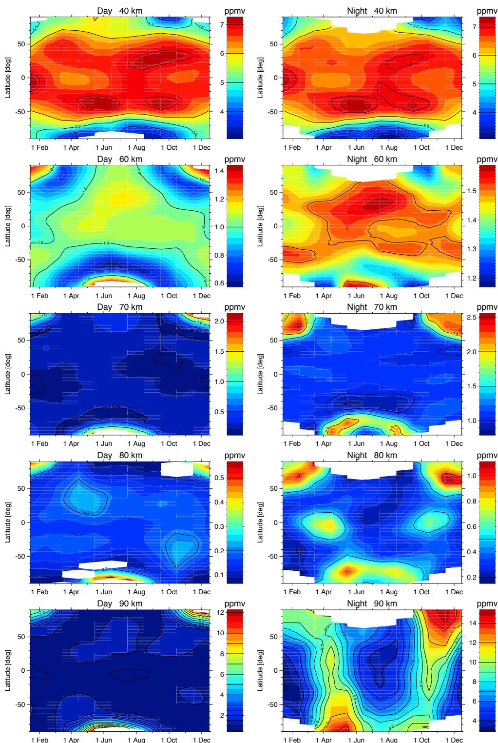
Figure 12. Seasonal evolution versus latitude of O_3 vmr at different altitudes for daytime (left row) and nighttime (right row). Note the different scales used in the different panels.
