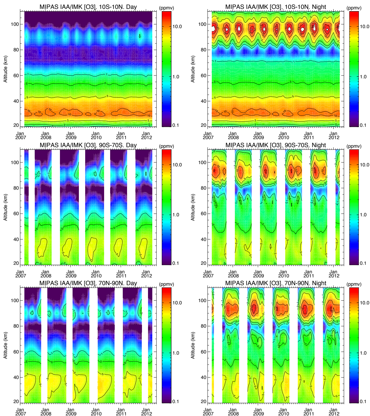
Figure 13. Altitude-resolved series, for latitudes near the equator ( 10^{\circ}\text{S} - 10^{\circ}\text{N} ) (top), the Southern polar region, 70^{\circ}\text{S} - 90^{\circ}\text{S} , (middle) and the Northern polar region, 70^{\circ}\text{N} - 90^{\circ}\text{N} (bottom), for daytime (left column) and nighttime (right column).
