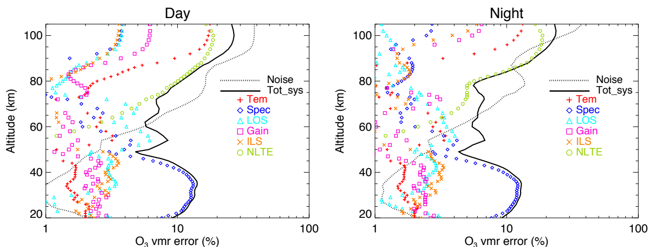
Figure 4. Errors of the retrieved O_3 vmr for daytime (left) and nighttime (right) in relative values. The different sources are described in the legend of Table 4.
