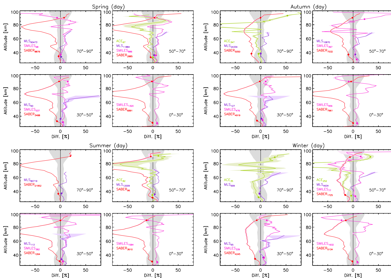
Figure 6. Mean of the daytime O_3 vmr differences (MIPAS–instrument) in % of MIPAS between co-located pairs of measurements of MIPAS (MA mode) with ACE-FTS (green), SABER (red), MLS (purple), and SMILES (magenta) for spring (MAM for NH and SON for SH) (upper/left quadrant), autumn (SON for NH and MAM for SH) (upper/right quadrant), summer (JJA for NH and DJF for SH) (bottom/left quadrant), and winter (DJF for NH and JJA for SH) (bottom/right quadrant). The symbols indicate the mean altitude of the MIPAS O_3 vmr primary (diamonds) and secondary (circles) maxima coincident with the respective instrument. The numbers of coincidences are indicated in the subscripts. The grey shaded area shows the MIPAS systematic errors. The color-shaded areas (hardly noticeable in many cases) are the standard errors of the mean of the differences.
