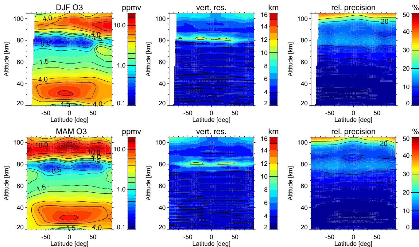
Figure 3. As Fig. 2 but for nighttime conditions.
