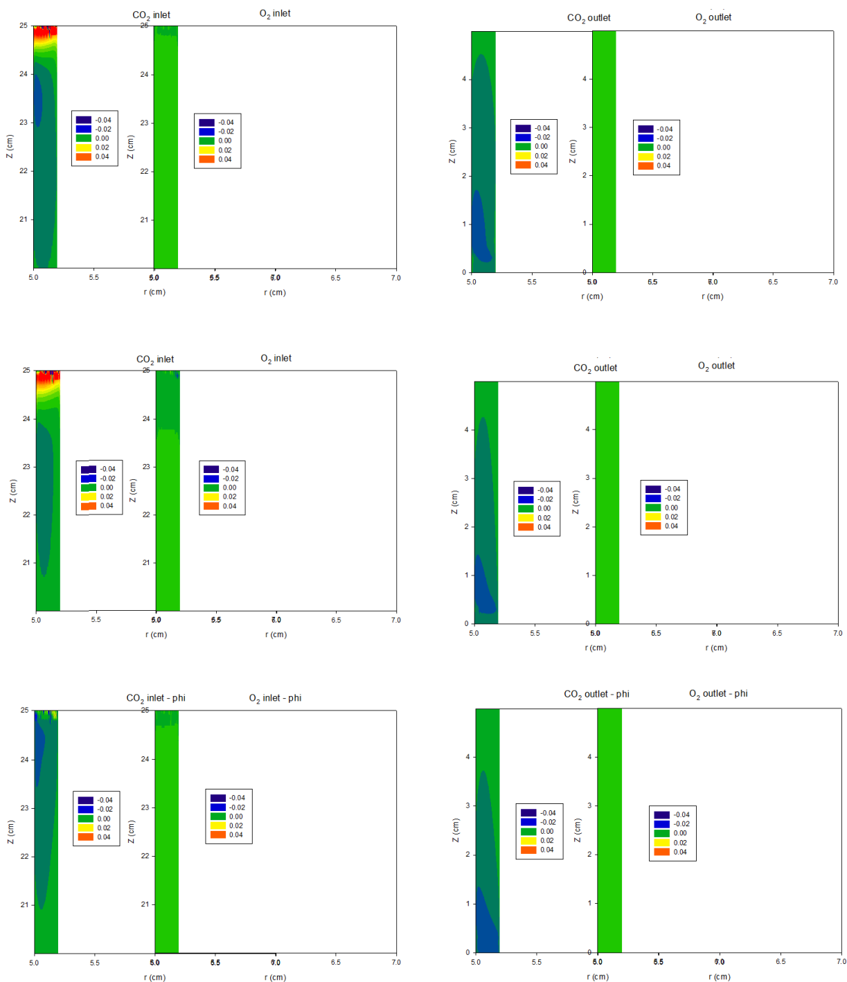
5 Figure 7: Computational fluid dynamic–simulated CO 2 and O 2 flow fields at inlet and outlet regions of APM under various rotation speeds.
