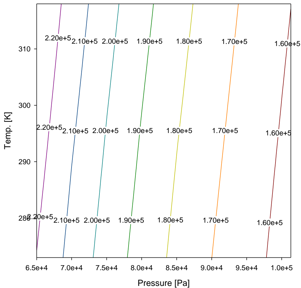
Figure 2: \frac{c_s}{\mu} ratio under various temperatures and pressures.
