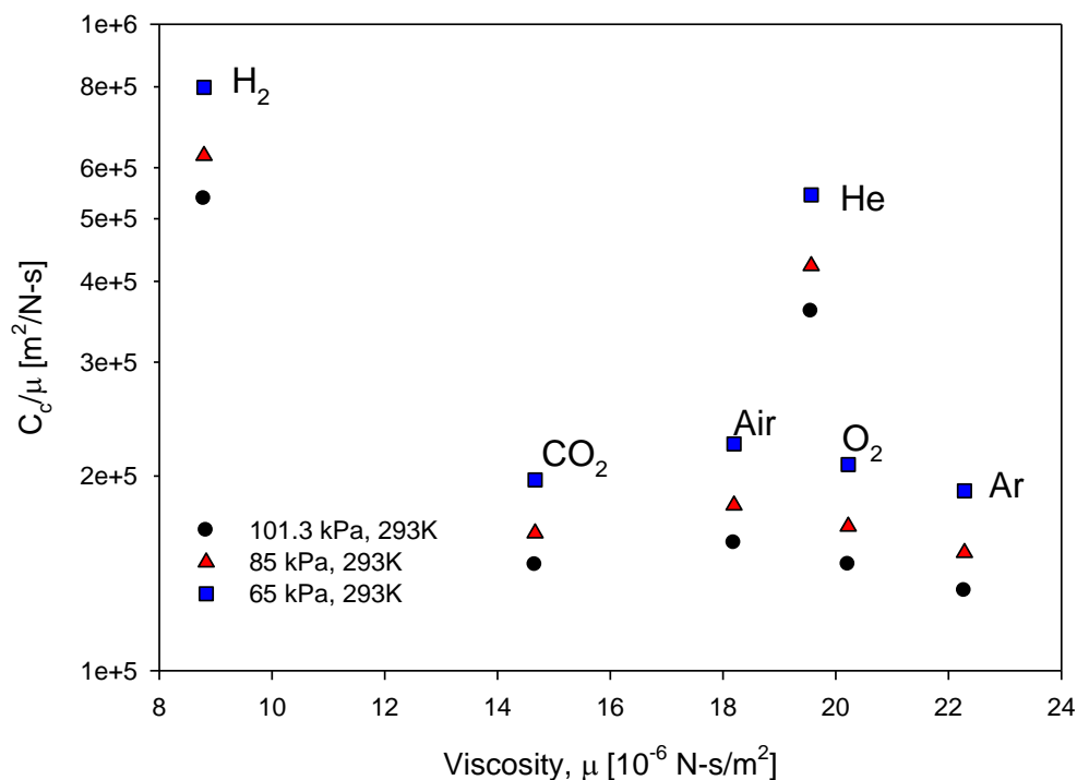
Figure 3: Pressure effect on C_c -to- \mu ratio under various carrier gases.
