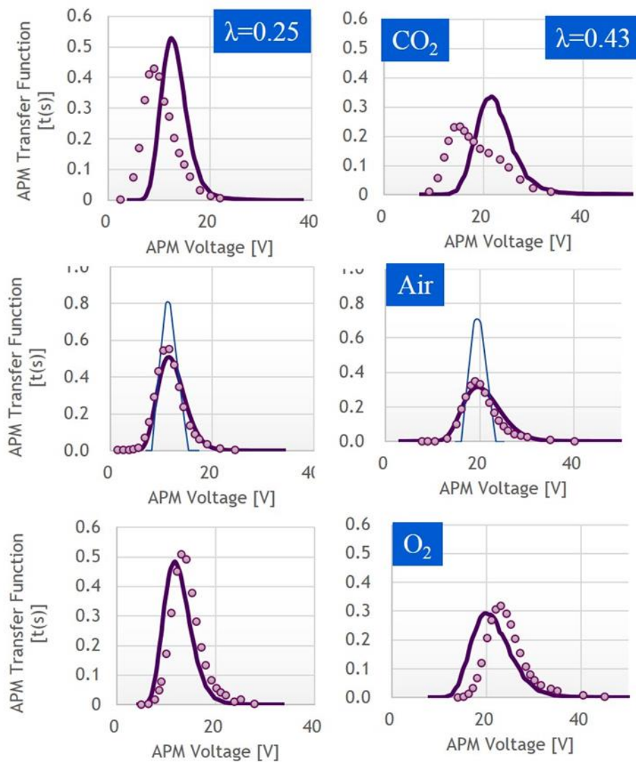
Figure 6: APM transfer function of 50-nm PSL spheres under various carrier gases with \lambda = 0.25 and 0.43 .
