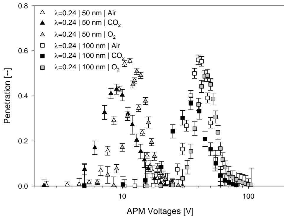
Figure 5: APM experimental transfer function of 50- and 100-nm PSL spheres under various carrier gases.
