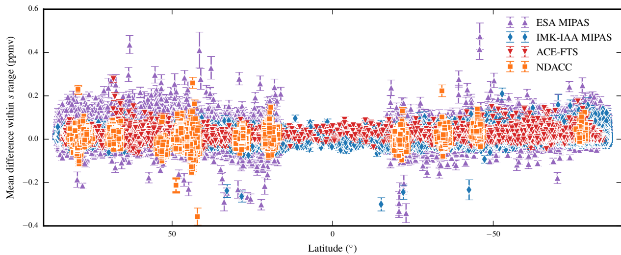
Figure 10. Mean \text{CH}_4 VMR differences between TANSO-FTS and each validation target data set, averaged vertically using the altitude range selected for integrating partial columns as a function of latitude. Differences are calculated as \text{TANSO-FTS} - \text{target} for each data set compared.
