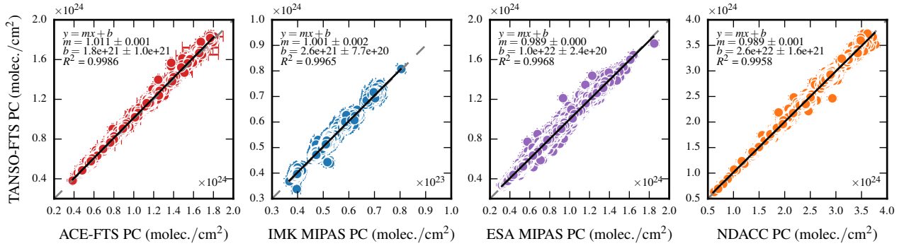
Figure 8. Partial column (PC) correlation plots comparing TANSO-FTS CH 4 to each validation instrument. Comparisons to ACE-FTS are red, to IMK-IAP MIPAS are blue, to ESA MIPAS are purple, and to NDACC are orange. The vertical range of partial column integration varies for each pair of coincident profiles based on the criteria described in Sect.7.1. The statistics for weighted linear least-squares regression are shown, with weights equal to 1/(\delta_x^2 + \delta_y^2) .
