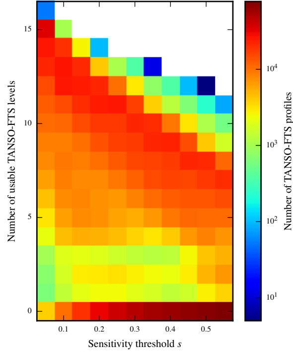
Figure 7. Two-dimensional histogram showing the number of TANSO-FTS \text{CH}_4 VMR profiles within our data set ( z -axis) that have some number of usable pressure levels ( y -axis) with a sensitivity greater than some given threshold, s ( x -axis). The data set shown here consists of all TANSO-FTS observations that are one-to-one coincident with a target validation data set. The threshold chosen for this study was s = 0.2 .
